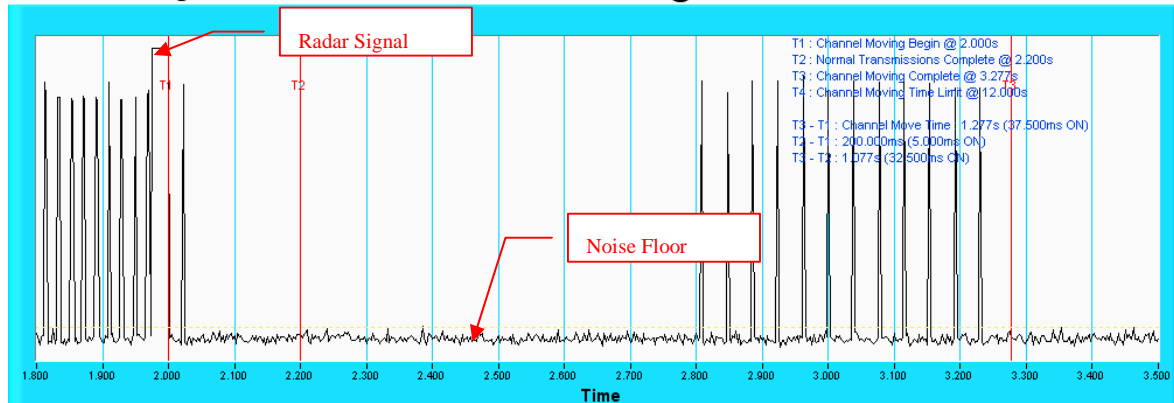
Channel Closing Transmission Time & Channel Move Time @ CH100 - 5500MHz
