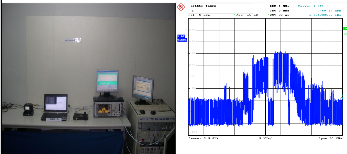
The Client device is set up to associate with the Master device and send a high enough rate of ICMP ping data from Master device.
