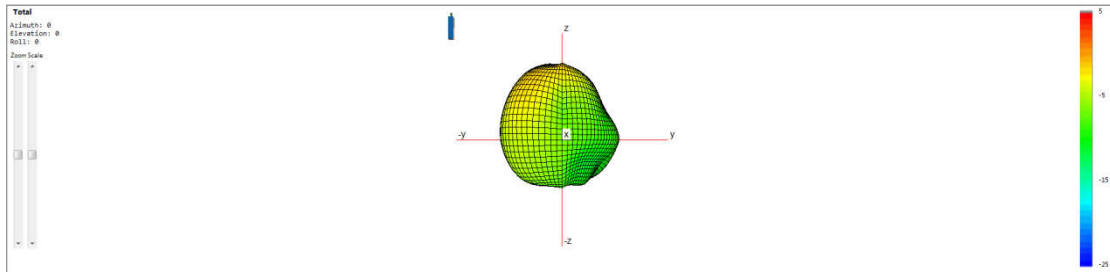
A7(Frequency=5600MHz)
