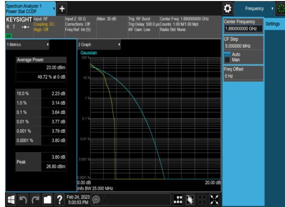
B7_N2(20M)_DFT-s-OFDM_PI_2-BPSK_Edge_1RB_Left_Mid_CH
