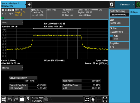
B7_N2(15M)_CP- OFDM_QPSK_Outer_Full_Mid_CH
