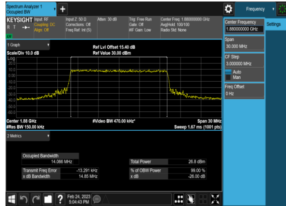
B7_N2(15M)_CP-OFDM_16 QAM_Outer_Full_Mid_CH
