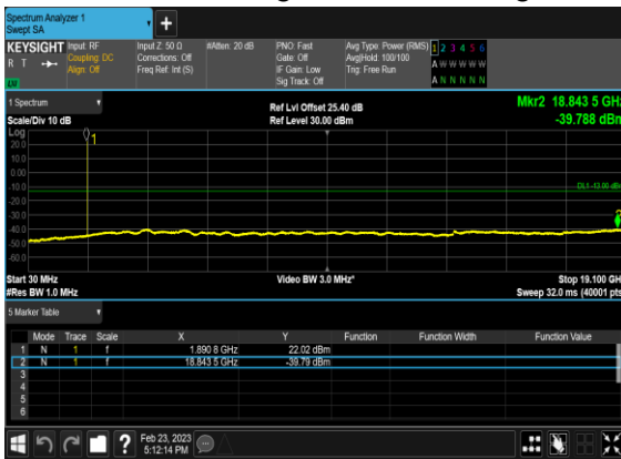
N2(20M)_DFT-s-OFDM_BPSK_Edge_1RB_Left_High_CH
