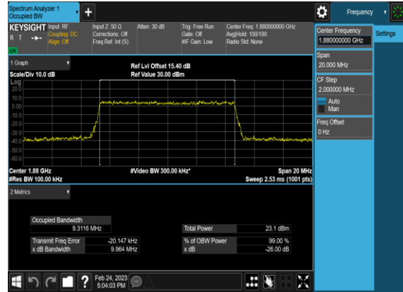
B7_N2(10M)_CP-OFDM_256 QAM_Outer_Full_Mid_CH
