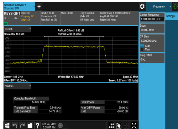
B7_N2(15M)_CP-OFDM_256 QAM_Outer_Full_Mid_CH
