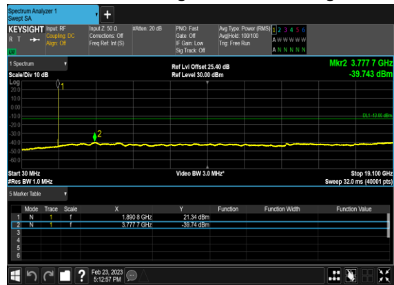
N2(20M)_DFT-s-OFDM_QPSK_Edge_1RB_Left_High_CH
