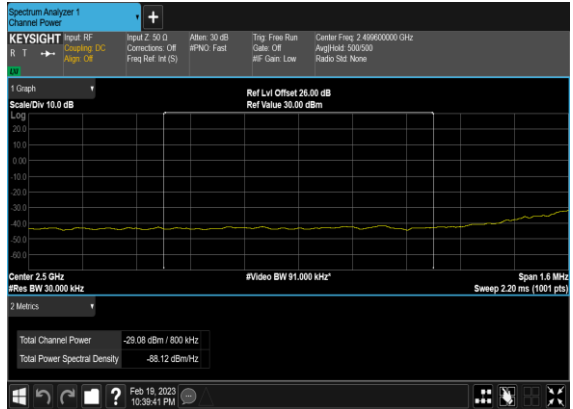
N7(40M)_DFT-s-OFDM_BPSK_Outer_Full_Low_CH_CHP_PASS
