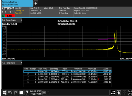
N7(40M)_DFT-s-OFDM_QPSK_Edge_1RB_Left_Low_CH
