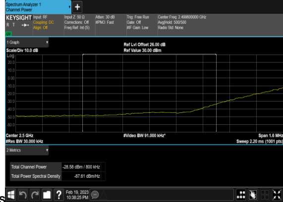
N7(40M)_DFT-s-OFDM_QPSK_Edge_1RB_Left_Low_CH_CHP_PA
