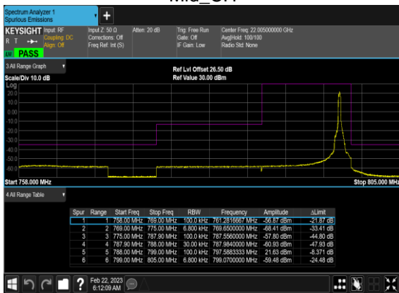
N14(10M)_DFT-s-OFDM_BPSK_Edge_1RB_Right_Mid_CH
