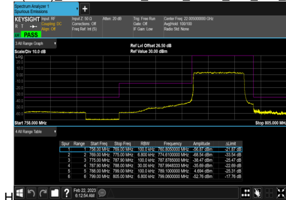
N14(10M)_DFT-s-OFDM_BPSK_Outer_Full_Mid_C
