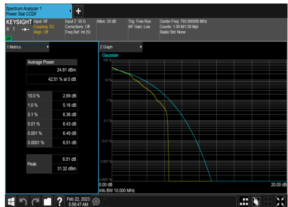
N14(10M)_DFT-s-OFDM_QPSK_Edge_1RB_Left_ _Mid_CH
