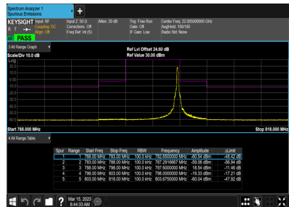
N14(10M)_DFT-s-OFDM_QPSK_Outer_Full_Mid_C
