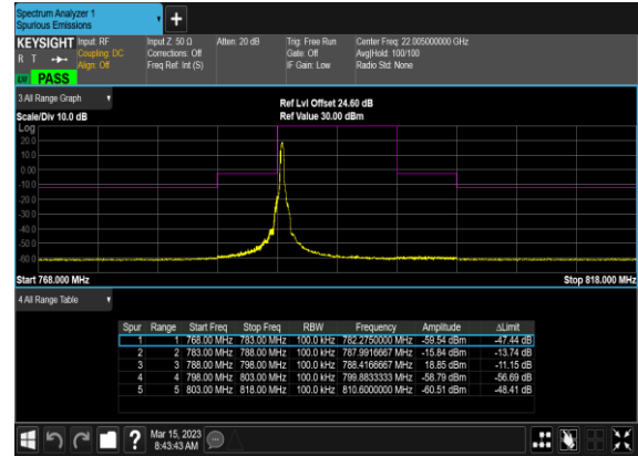
N14(10M)_DFT-s-OFDM_QPSK_Edge_1RB_Right_M
