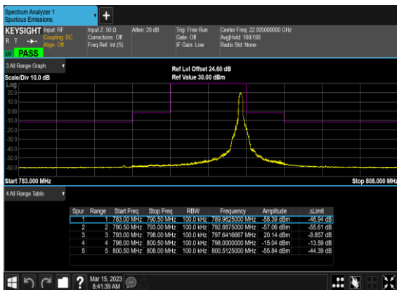
N14(5M)_DFT-s-OFDM_BPSK_Outer_Full_High_C
