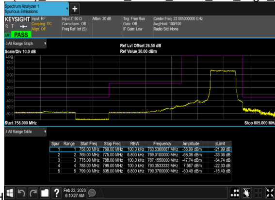
N14(5M)_DFT-s-OFDM_BPSK_Outer_Full_High_C
