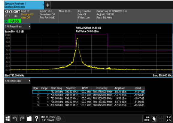
N14(5M)_DFT-s-OFDM_QPSK_Edge_1RB_Right_H
