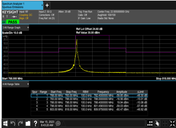
N14(10M)_DFT-s-OFDM_BPSK_Edge_1RB_Right_M
