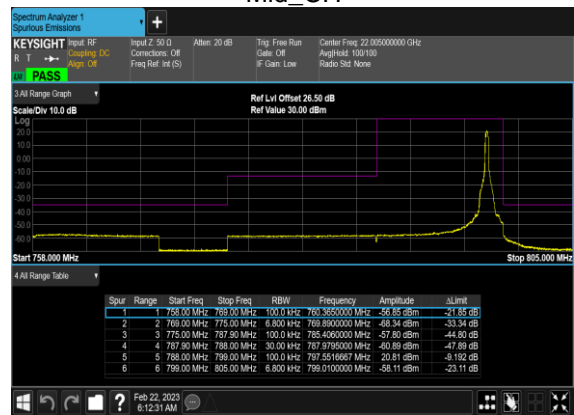
N14(10M)_DFT-s-OFDM_QPSK_Edge_1RB_Right_Mid_CH
