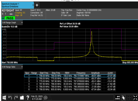
N14(10M)_DFT-s-OFDM_BPSK_Edge_1RB_Left_M id_CH
