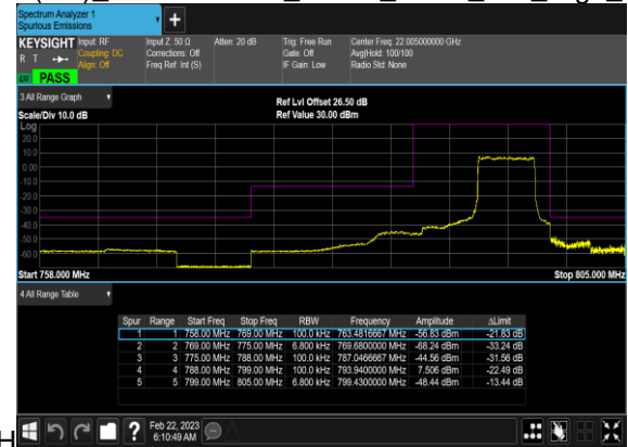
N14(5M)_DFT-s-OFDM_QPSK_Outer_Full_High_C
