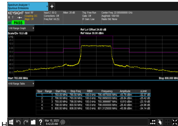
N14(5M)_DFT-s-OFDM_BPSK_Outer_Full_High_C
