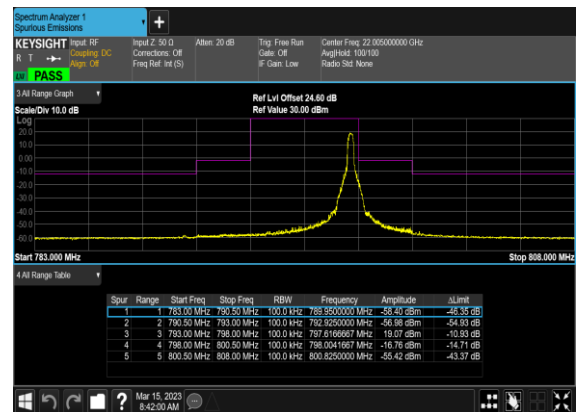
N14(5M)_DFT-s-OFDM_QPSK_Outer_Full_High_C
