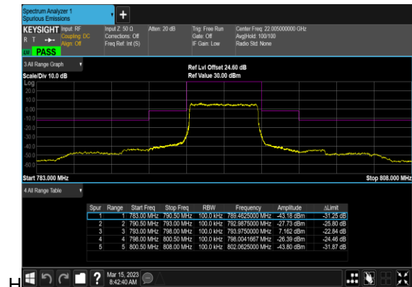
N14(5M)_DFT-s-OFDM_QPSK_Outer_Full_High_C
