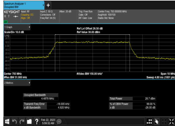
N14(5M)_CP-OFDM_16 QAM_Outer_Full_Mid_CH
