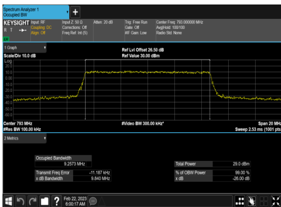
N14(10M)_CP-OFDM_QPSK_Outer_Full_Mid_CH
