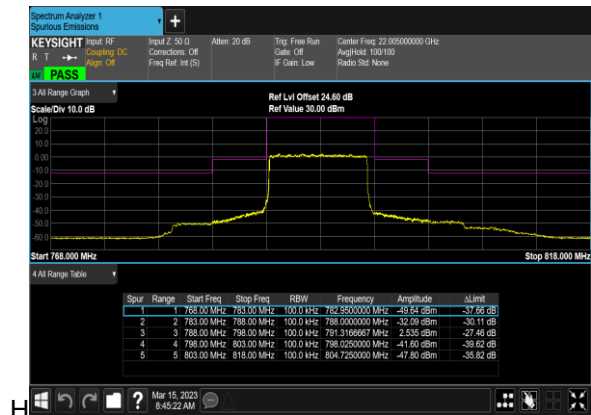
N14(10M)_DFT-s-OFDM_QPSK_Outer_Full_Mid_C
