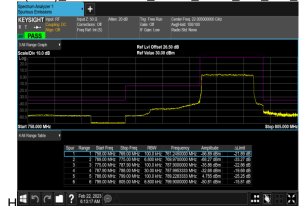
N14(10M)_DFT-s-OFDM_QPSK_Outer_Full_Mid_C
