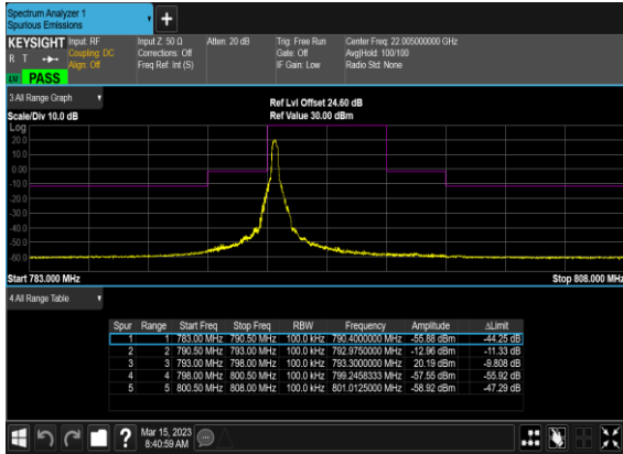
N14(5M)_DFT-s-OFDM_BPSK_Edge_1RB_Right_H
