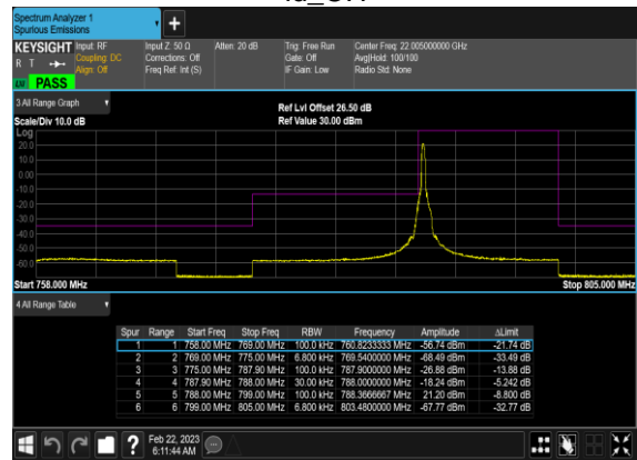
N14(10M)_DFT-s-OFDM_QPSK_Edge_1RB_Left_M id_CH
