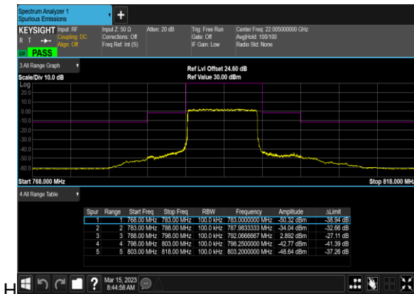
N14(10M)_DFT-s-OFDM_BPSK_Outer_Full_Mid_C
