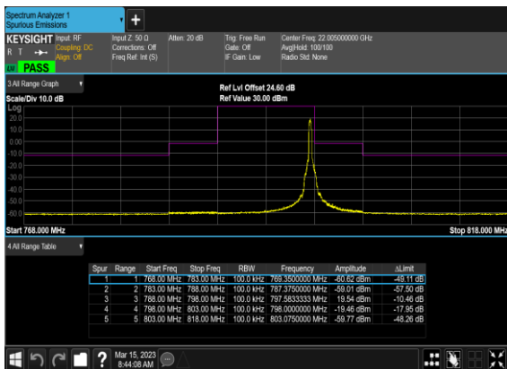
N14(10M)_DFT-s-OFDM_BPSK_Outer_Full_Mid_C
