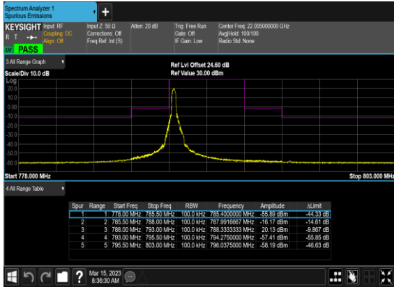
N14(5M)_DFT-s-OFDM_BPSK_Edge_1RB_Right_L
