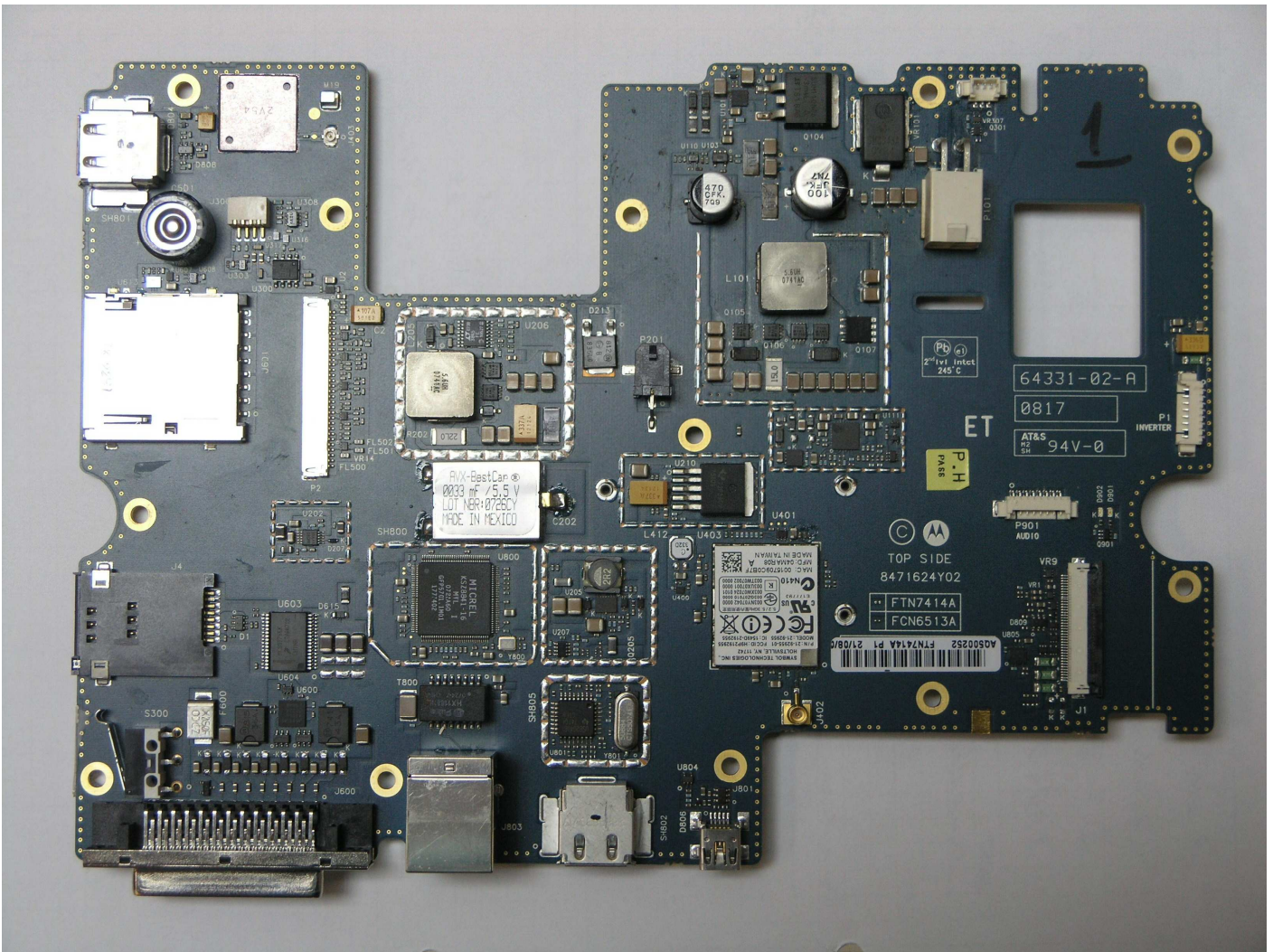
VC6096 Main Board top side with shields
