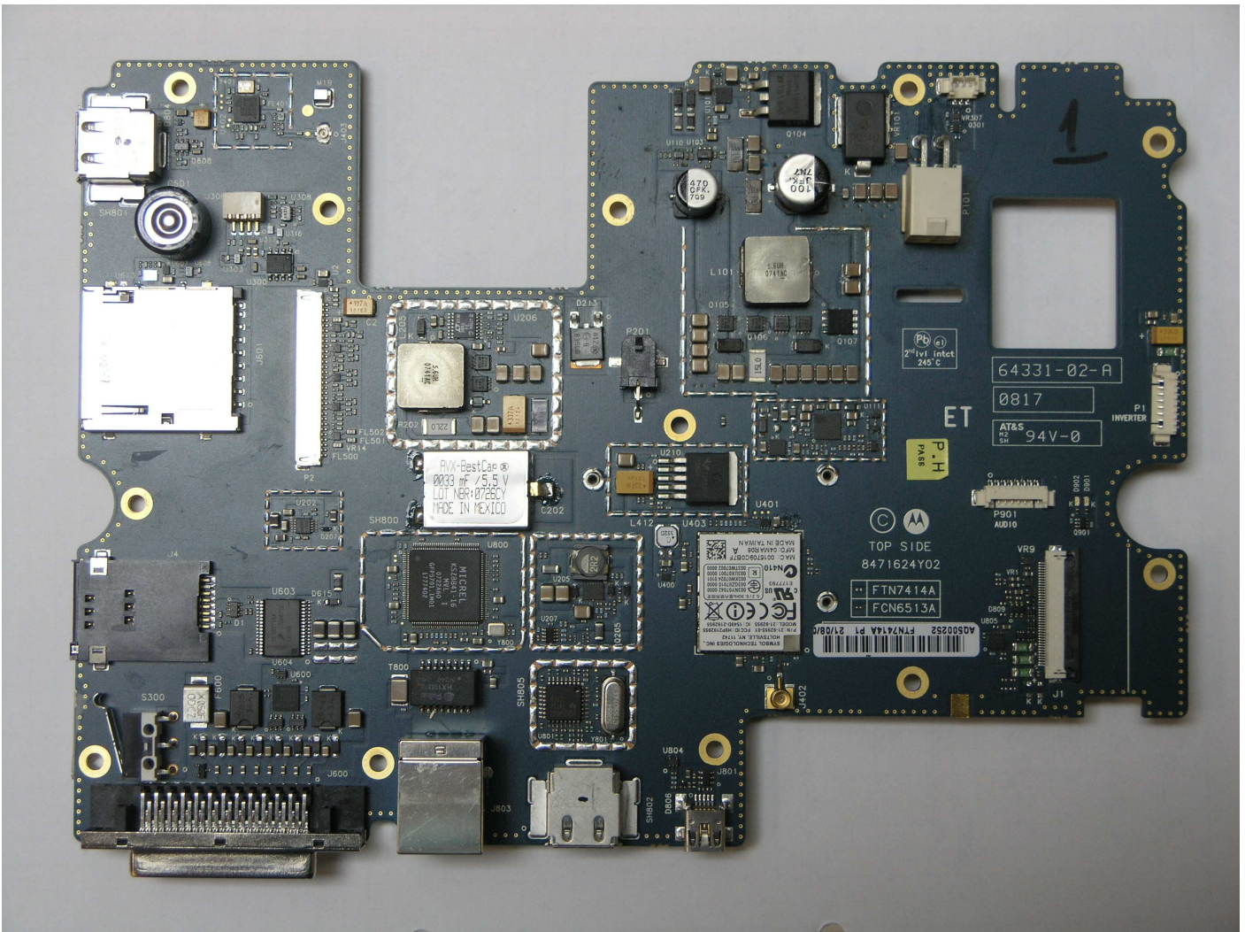
VC6096 Main Board top side w/o shields
