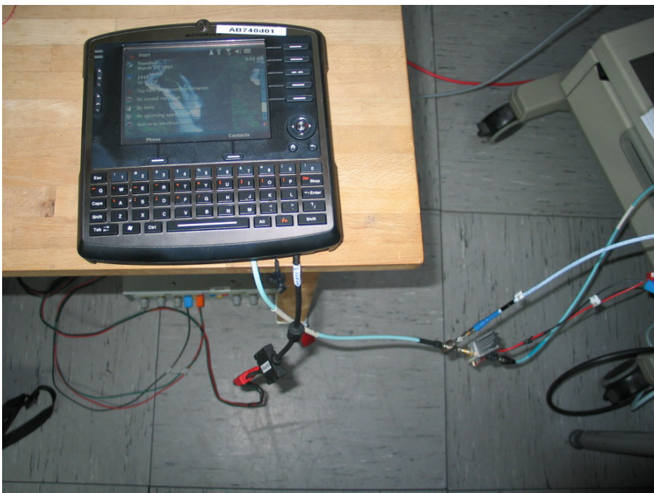
Photo 4: Setup for conducted tests
