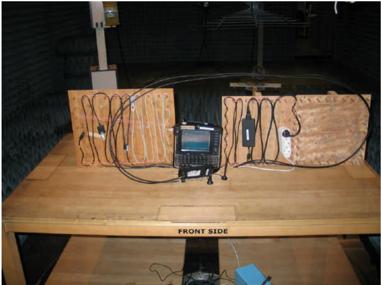
Photo 2: Test setup for radiated measurements (above 30 MHz, below 1 GHz)
