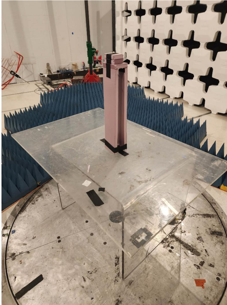
Photograph 4. Output Power Test Setup
