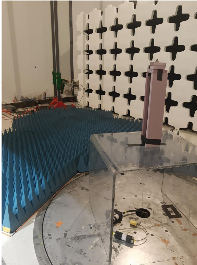
Photograph 2. Radiated Spurious Emissions Test Setup, 1-18GHz
