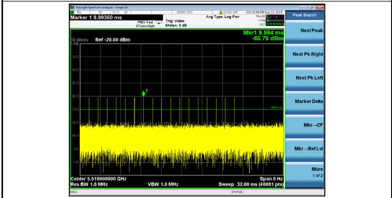
Calibration Radar #0 detection threshold level
