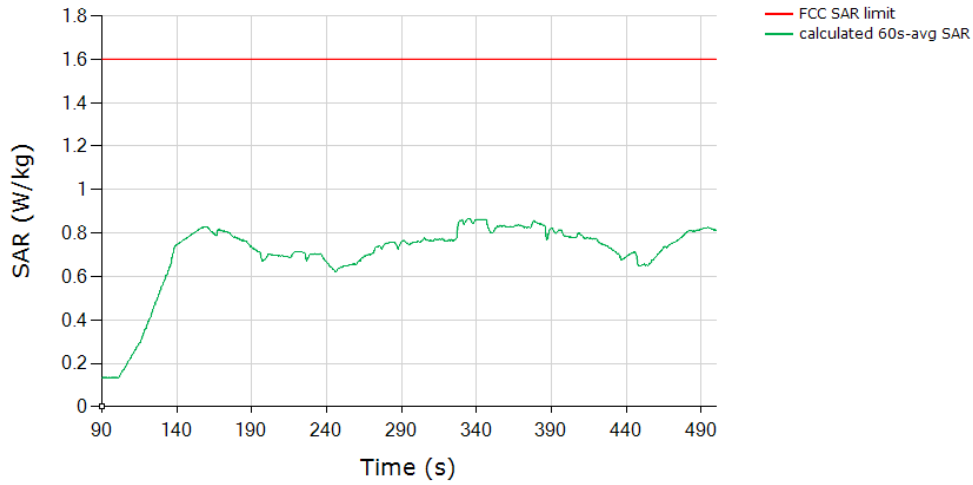
SAR (Test Sequence 2) Tech: NRSUB6SA, Band 77
