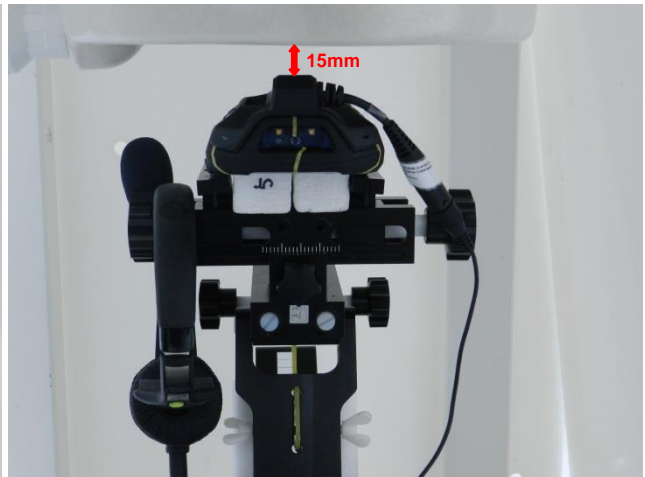
Back with Earphone 2, Test Separation 15 mm
