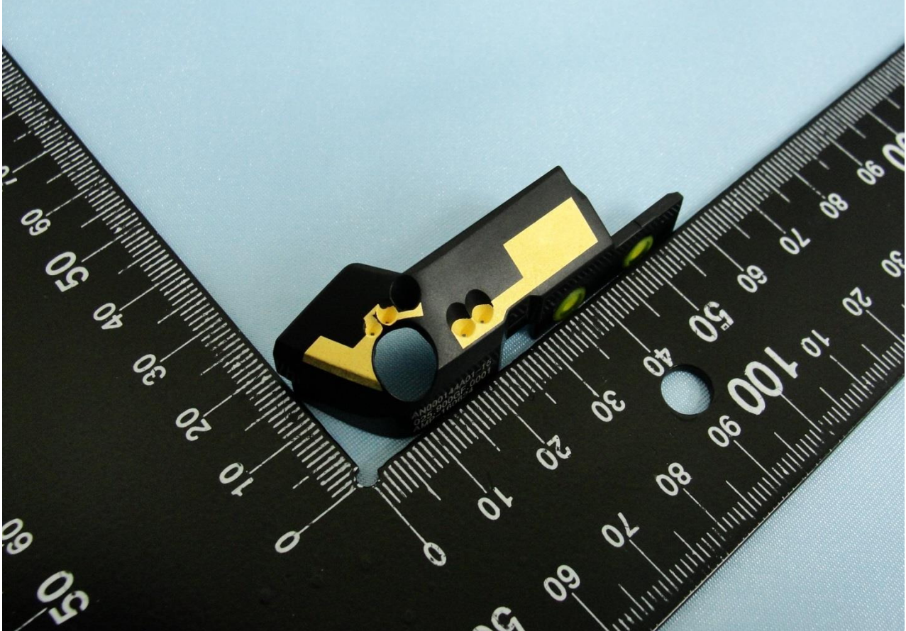
WLAN Main Antenna and Bluetooth Antenna
