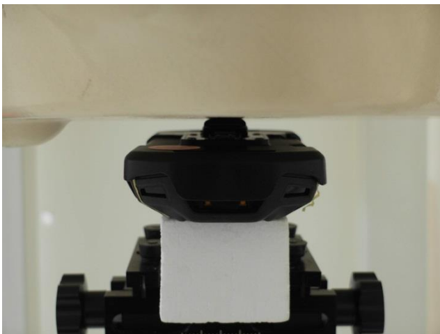
Front with Rigid Holster, Test Separation 0 mm
