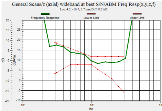
Fig 8.16 GSM850 Ch128
