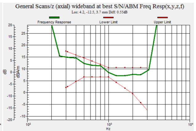
Fig 8.6 GSM1900 Ch810
