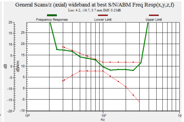
Fig 8.17 GSM1900 Ch810
