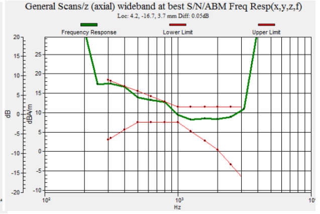
Fig 8.22 GSM1900 Ch810
