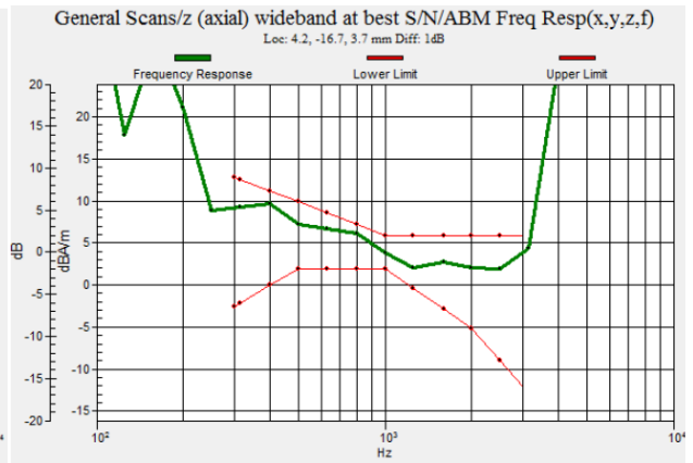
Fig 8.4 GSM1900 Ch512
