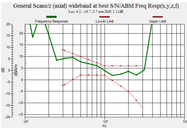
Fig 8.3 GSM850 Ch251
