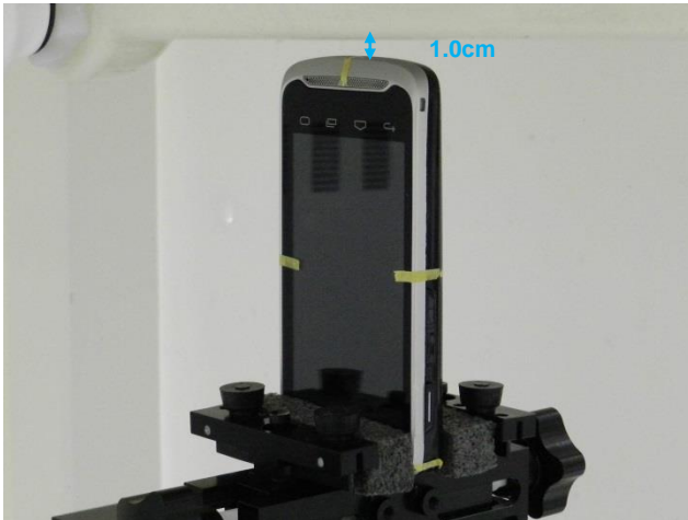
Bottom Side With Battery 1, Test Separation 1 cm
