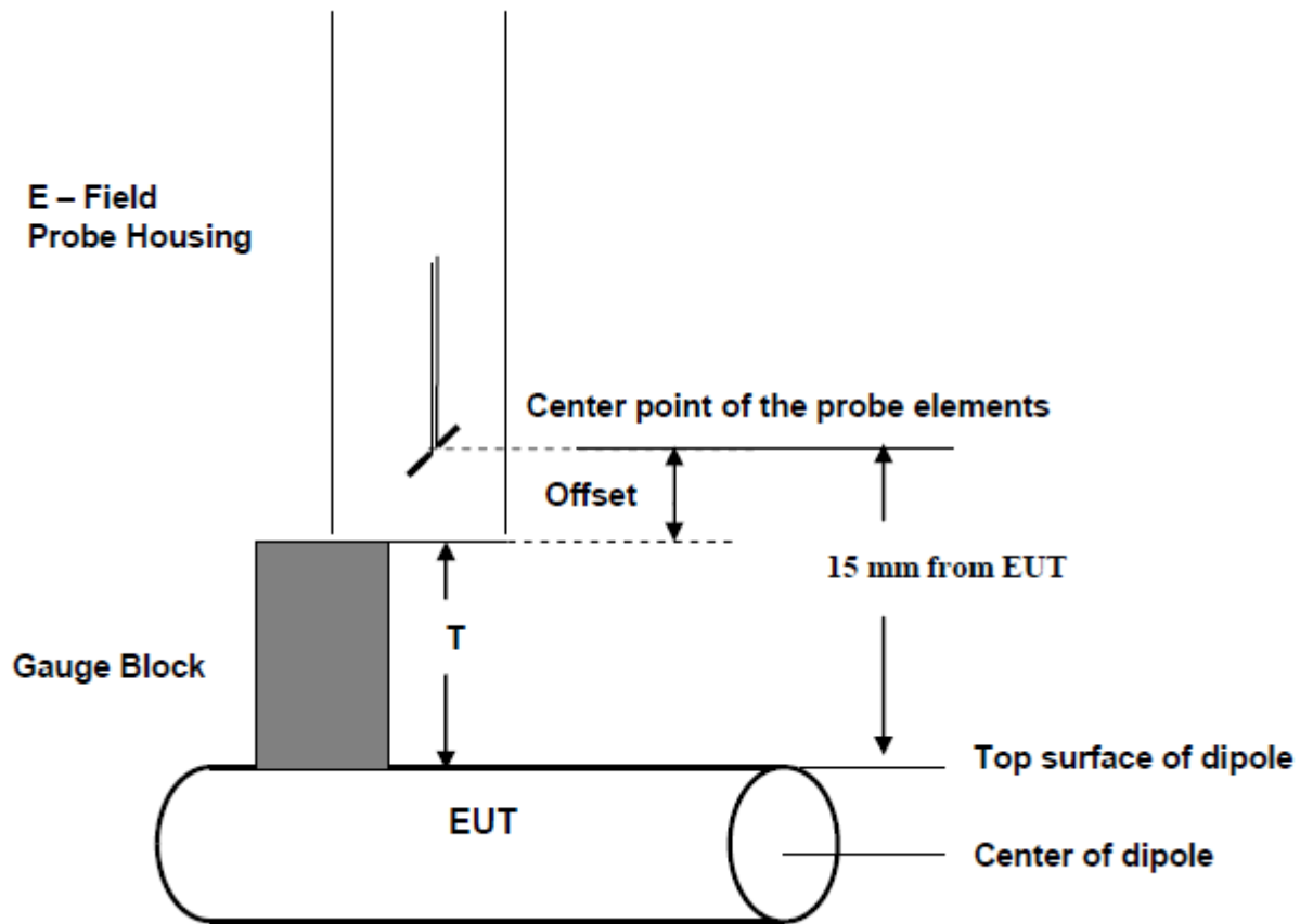
Fig. 9.2 Gauge block with E-field probe
