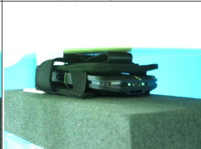
Holster - (Rear) Top join of EUT at 0 mm
