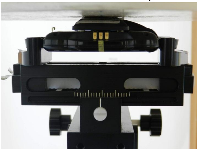
Back of the EUT with Speaker at 0 cm Gap
