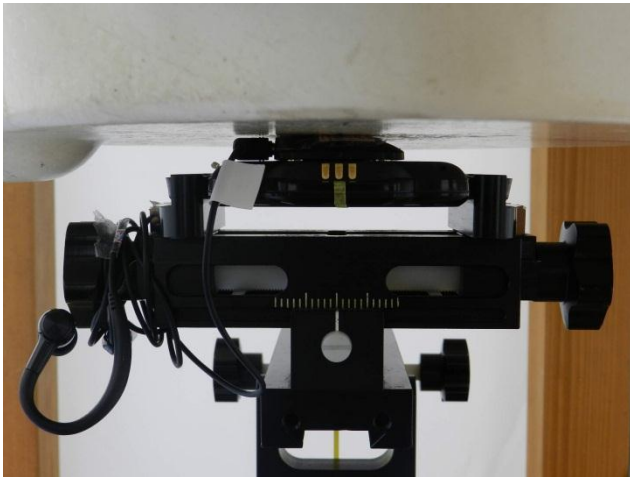
Back of the EUT with Headset nugget with Headset 1 at 0 cm Gap
