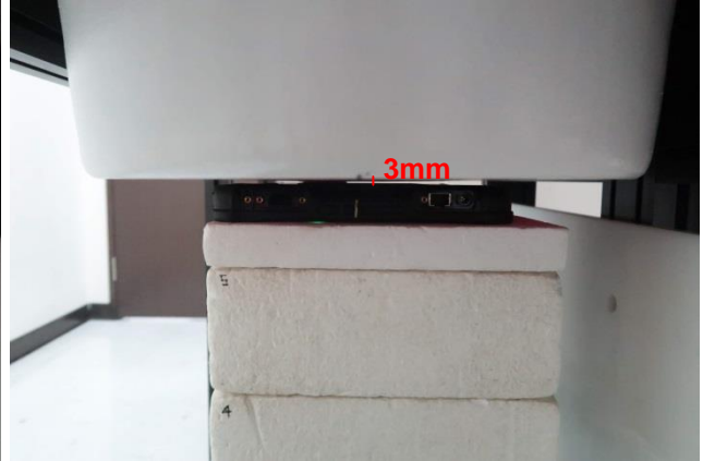
Bottom Face, Test Separation 3 mm
