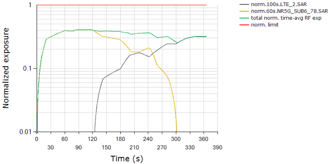
Total Normalized Time-averaged RF Exposure Tech: LTE, Band 2 / Tech: NR5G SUB6, Band 78
