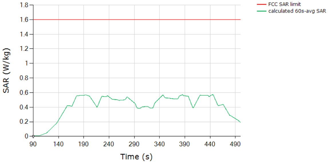
SAR (Test Sequence 2) Tech: NRSUB6SA, Band 77
