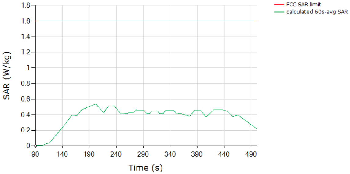
SAR (Test Sequence 2) Tech: NRSUB6SA, Band 48
