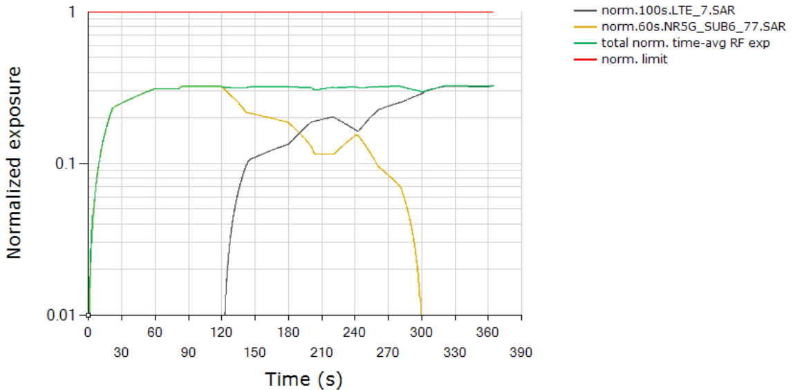
Total Normalized Time-averaged RF Exposure Tech: LTE, Band 7 / Tech: NR5G SUB6, Band 77
