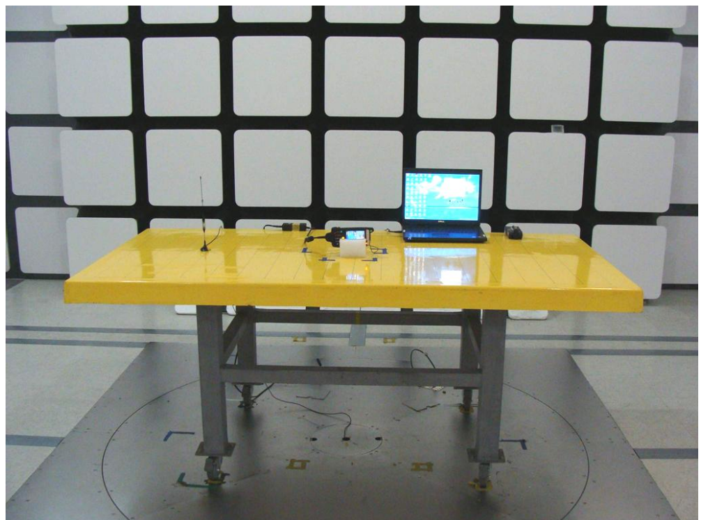
Co-location with WLAN Mode for Numeric Keypad
