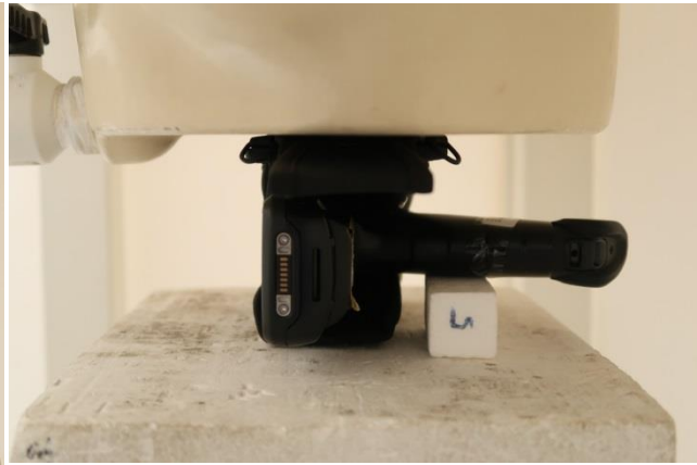
Right Side, Gun + Battery 2/3/4/5+ KeyPad + Holster 3, Test Separation 0mm
