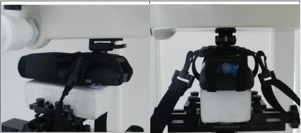
Back_0mm_Scanner 3_ EUT Type 1_ Holster 1
