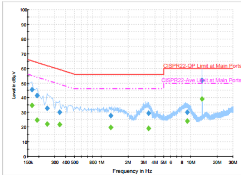
ENV216 Auto Test FCC Power Bar - N
