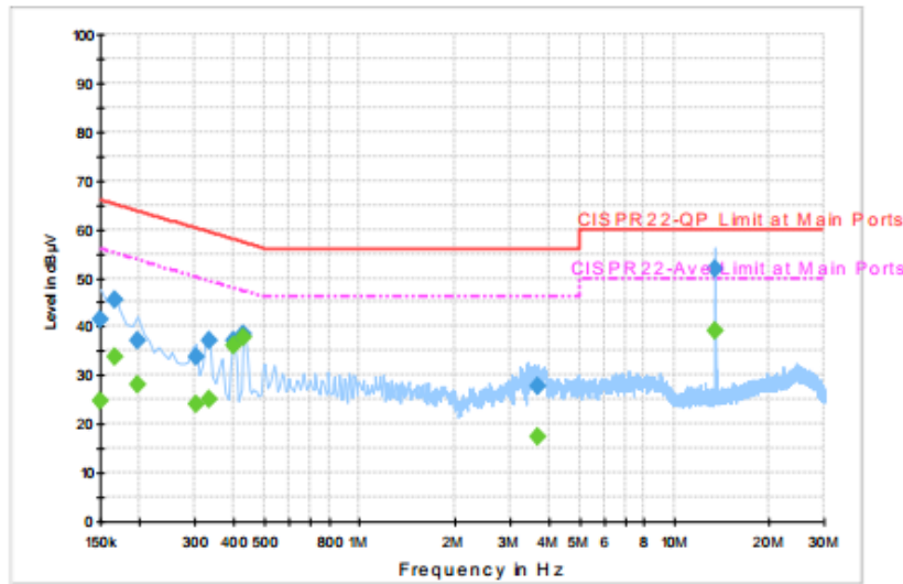
ENV216 Auto Test FCC Power Bar - L
