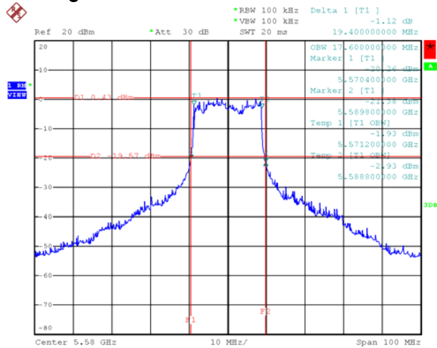
20dB Bandwidth Plot on Configuration Drafft n MCS8 20MHz / 5580 MHz
