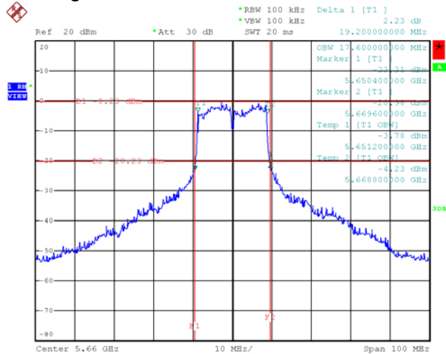
20dB Bandwidth Plot on Configuration Drafft n MCS8 20MHz / 5660 MHz
