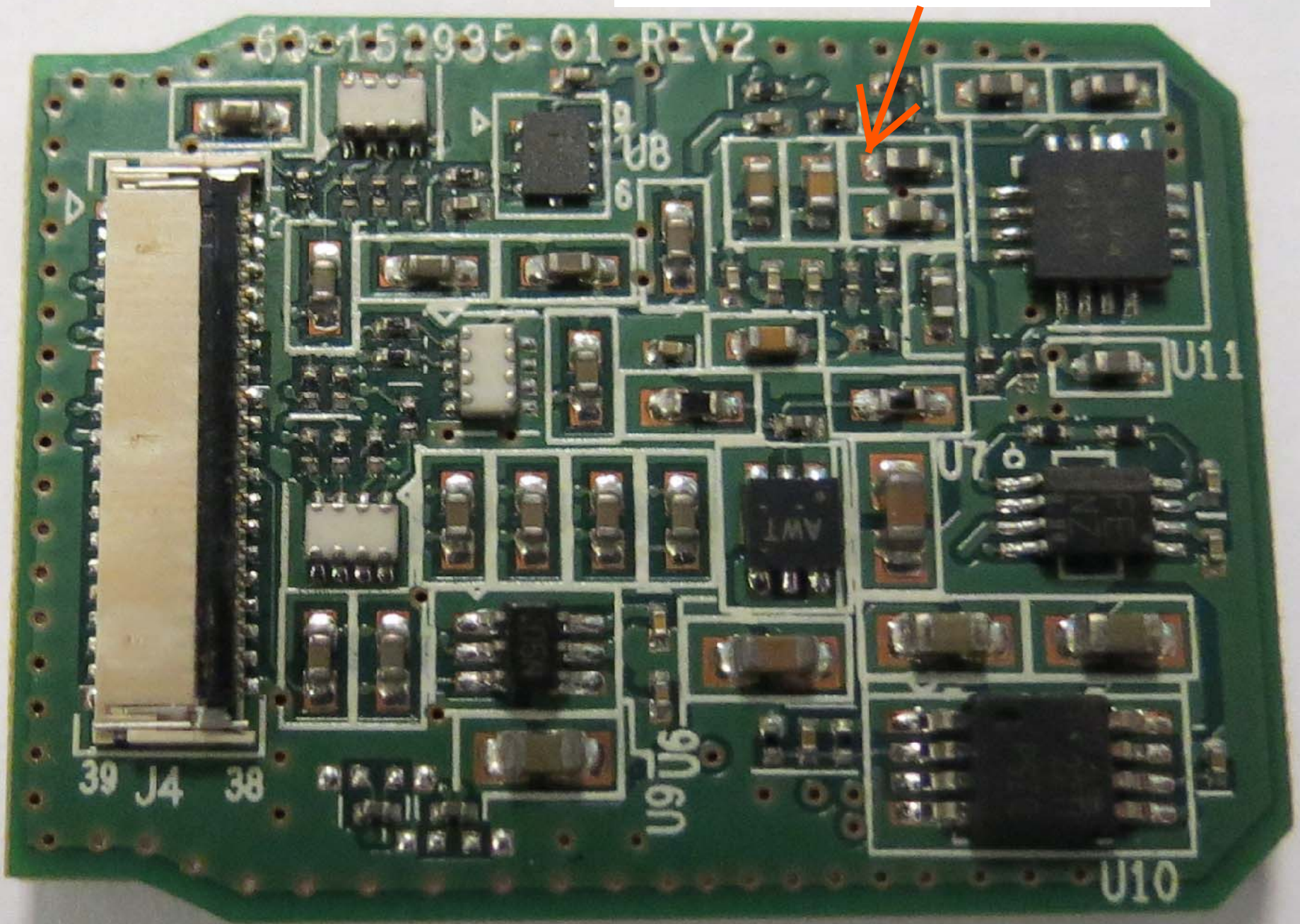
DISPLAY BOARD SECONDARY SIDE
