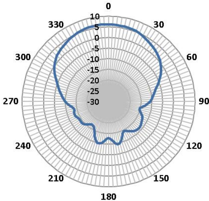
Antenna Gain - 900 MHz Band
