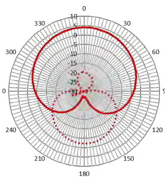
Horizontal (FCC)
