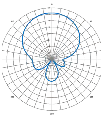
Horizontal (FCC)
