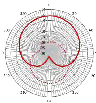
Vertical (FCC)
