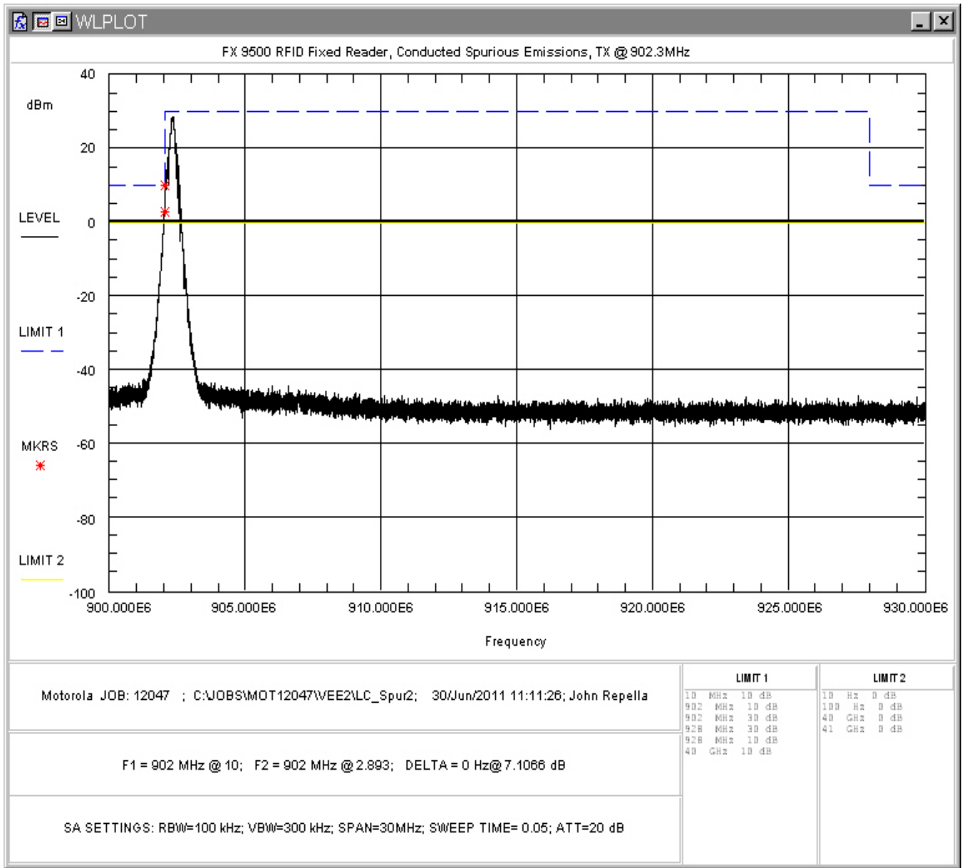
Figure 19: Conducted Spurious Emissions, Low Channel 900MHz – 930MHz
