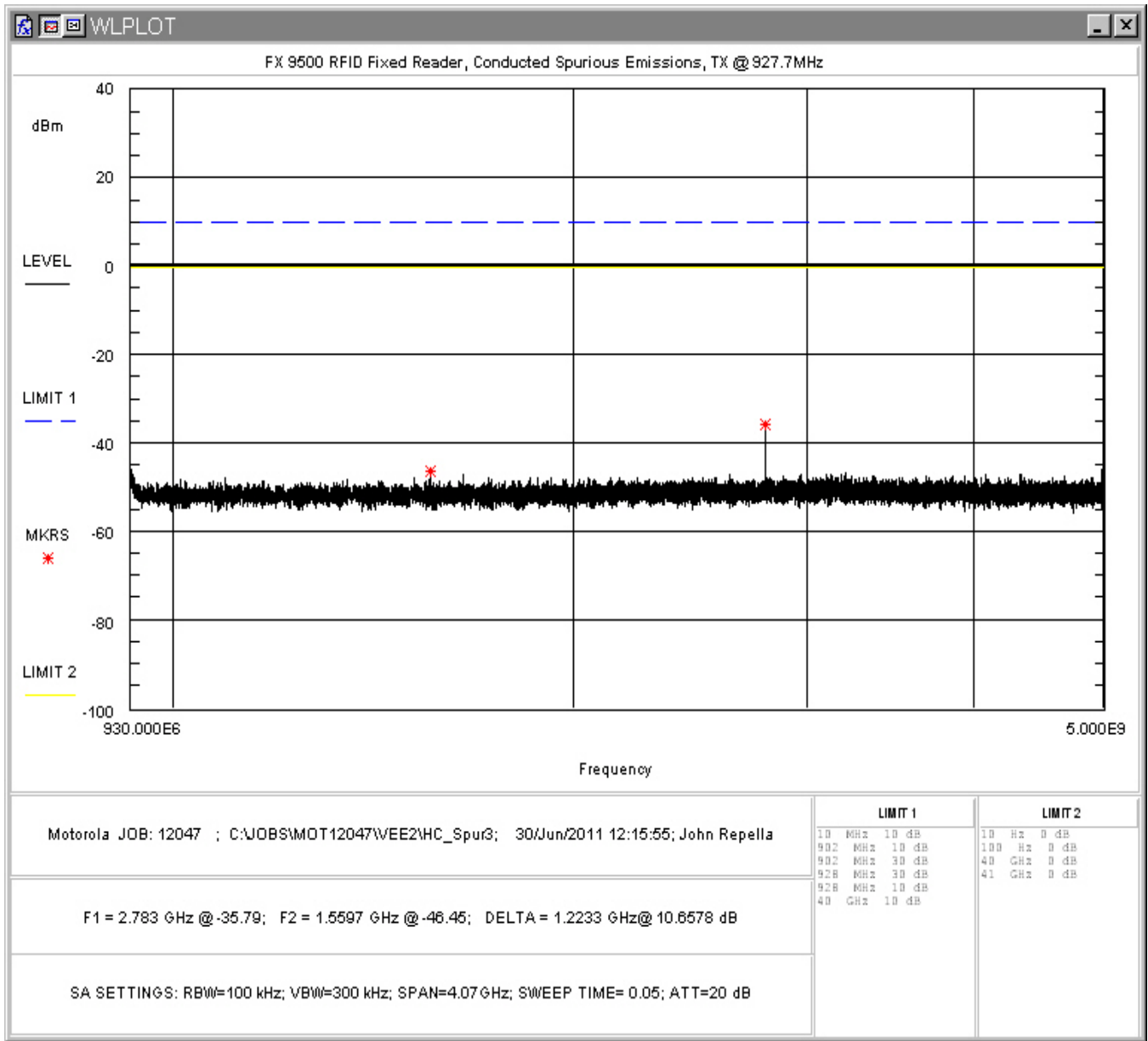
Figure 32: Conducted Spurious Emissions, High Channel 930MHz– 5GHz
