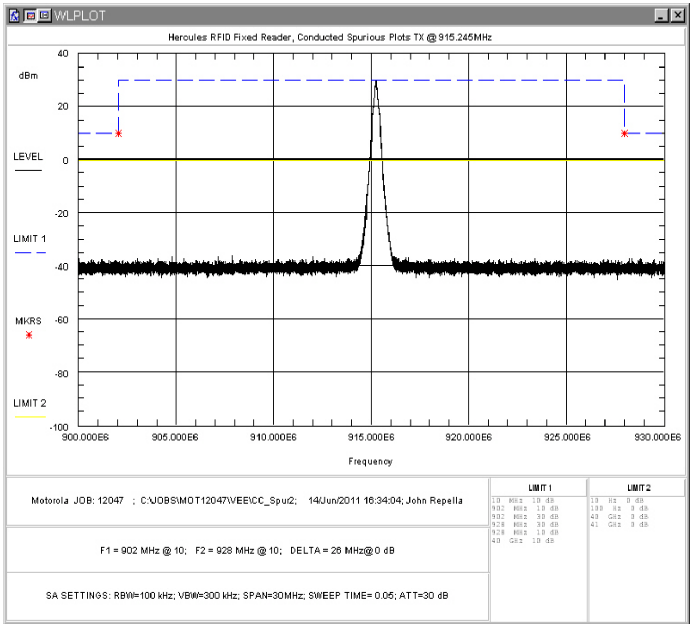
Figure 25: Conducted Spurious Emissions, Mid Channel 900MHz – 930MHz
