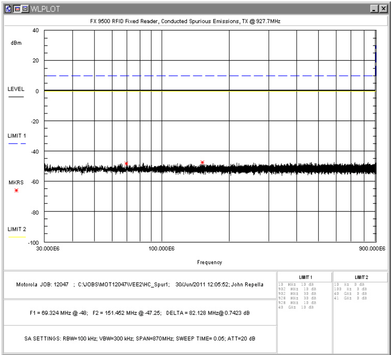
Figure 28: Conducted Spurious Emissions, High Channel 30 - 900MHz
