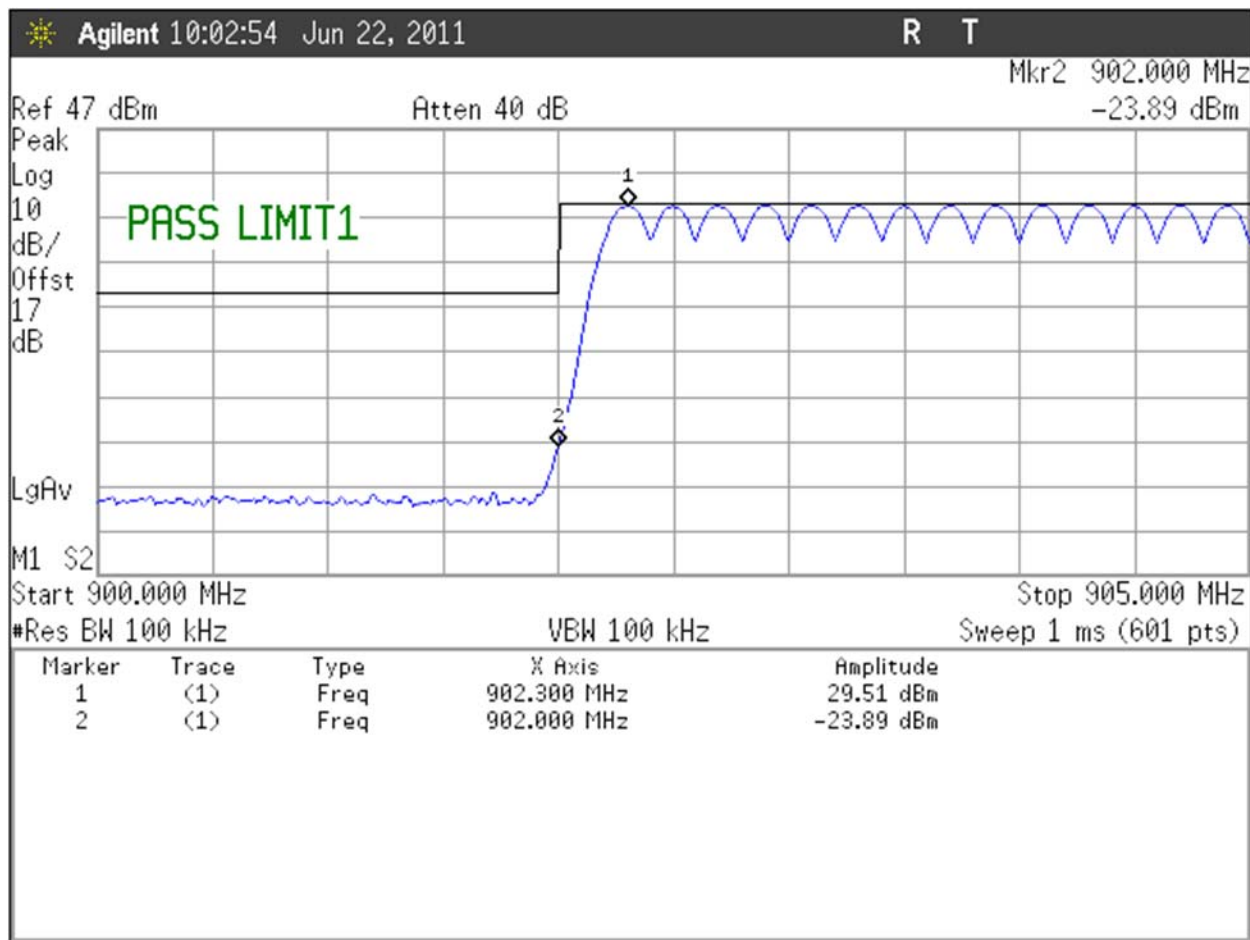
Figure 20: Band Edge Plot (Hopping), Low Channel TX @902.3MHz
