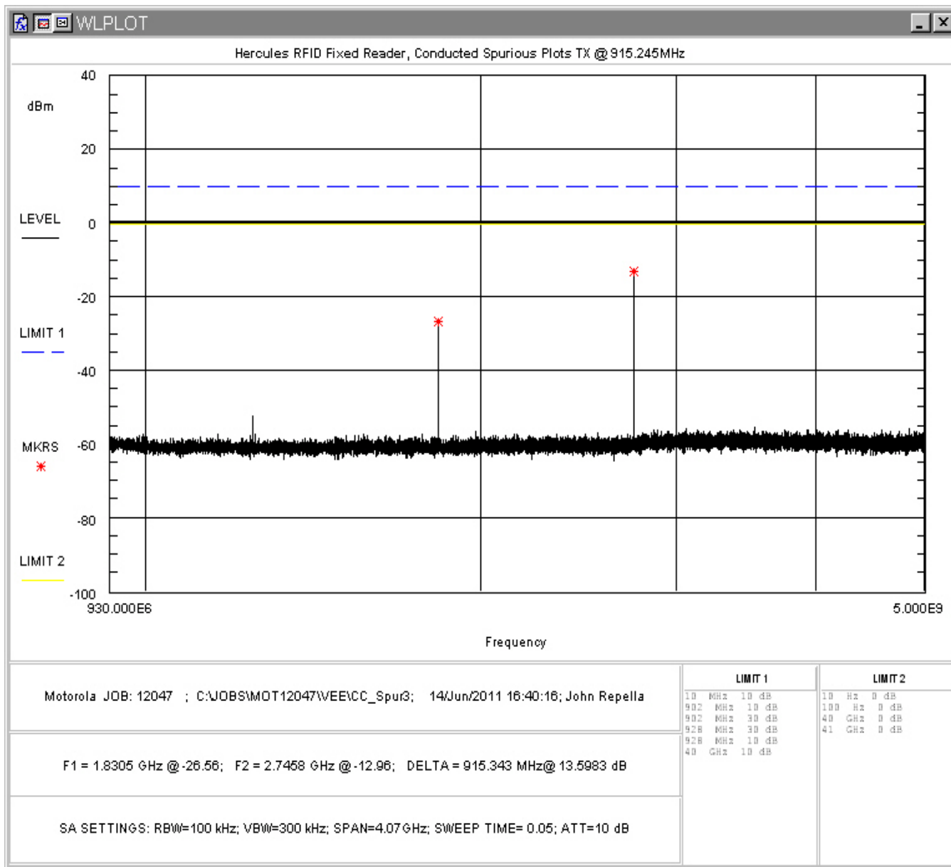
Figure 26: Conducted Spurious Emissions, Mid Channel 930MHz– 5GHz
