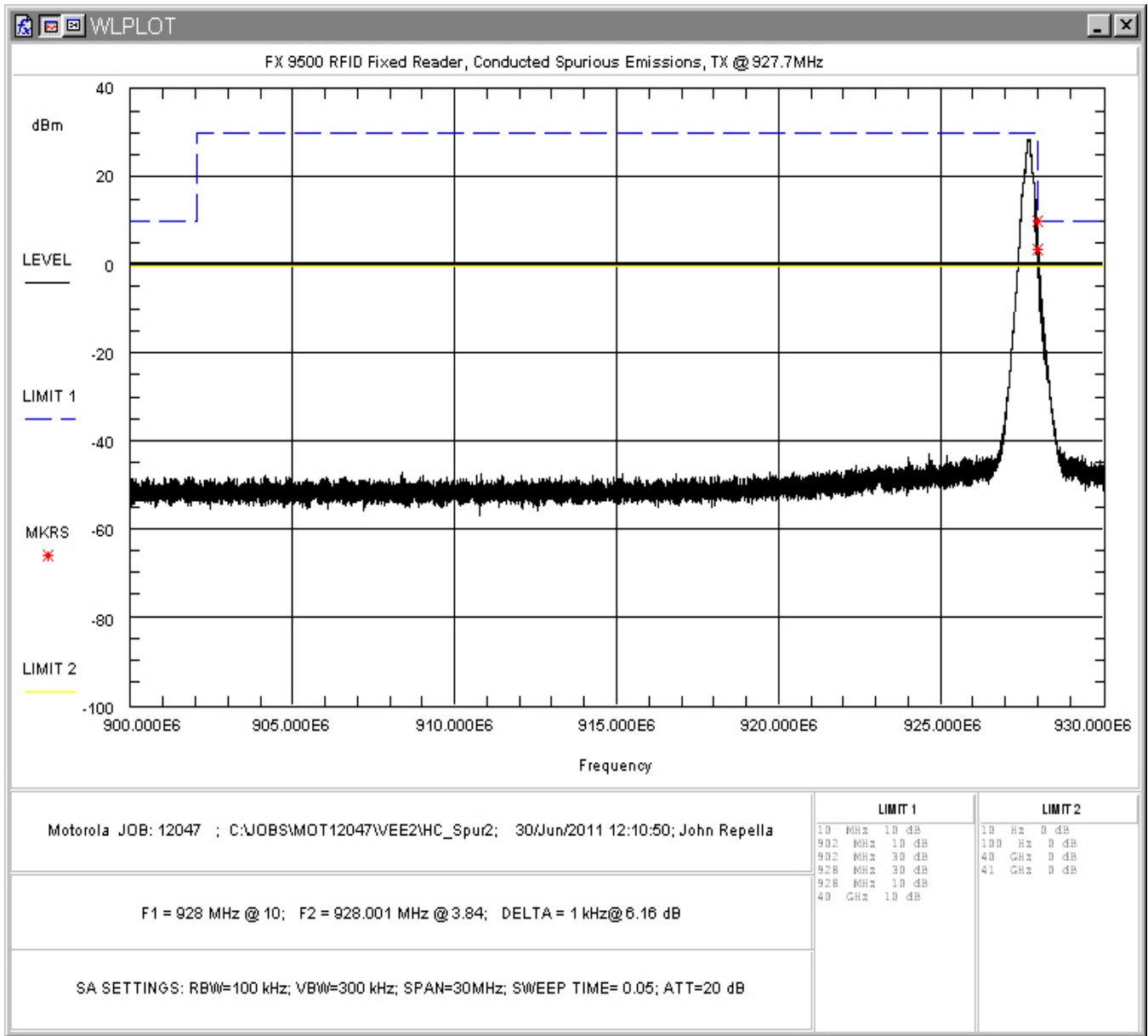
Figure 29: Conducted Spurious Emissions, High Channel 900MHz – 930MHz
