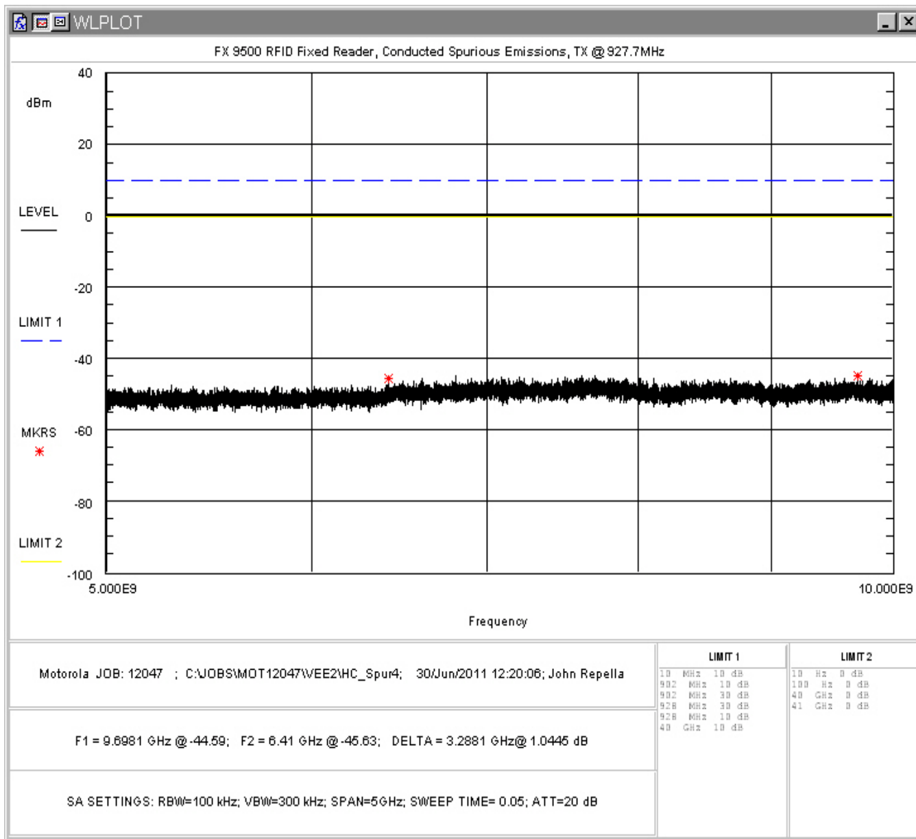
Figure 33: Conducted Spurious Emissions, High Channel 5 - 10GHz
