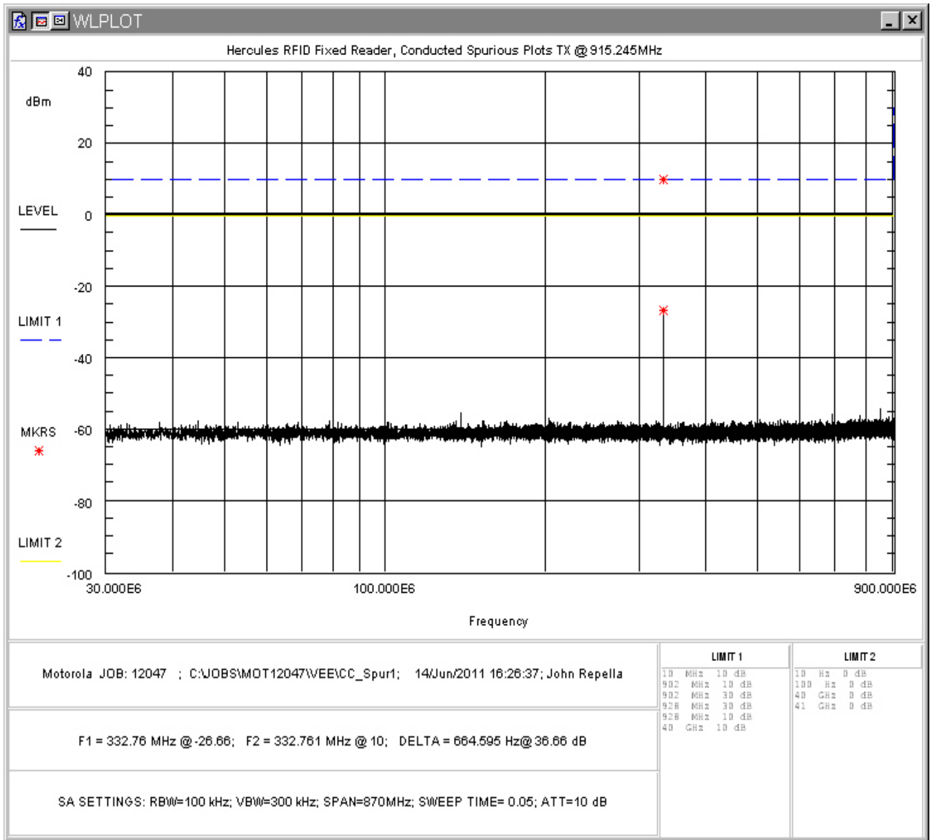
Figure 24: Conducted Spurious Emissions, Mid Channel 30 - 900MHz
