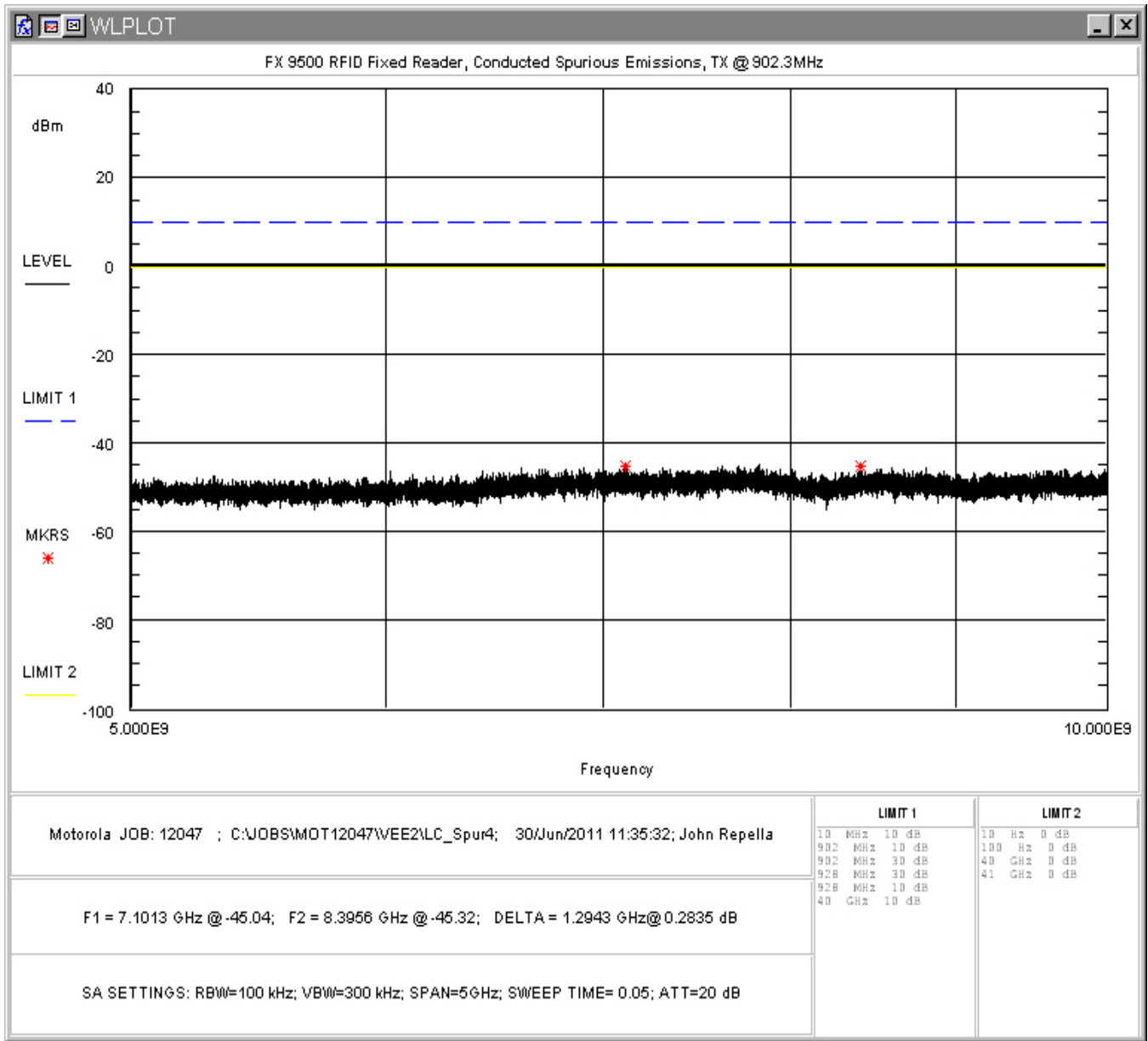
Figure 23: Conducted Spurious Emissions, Low Channel 5 - 10GHz
