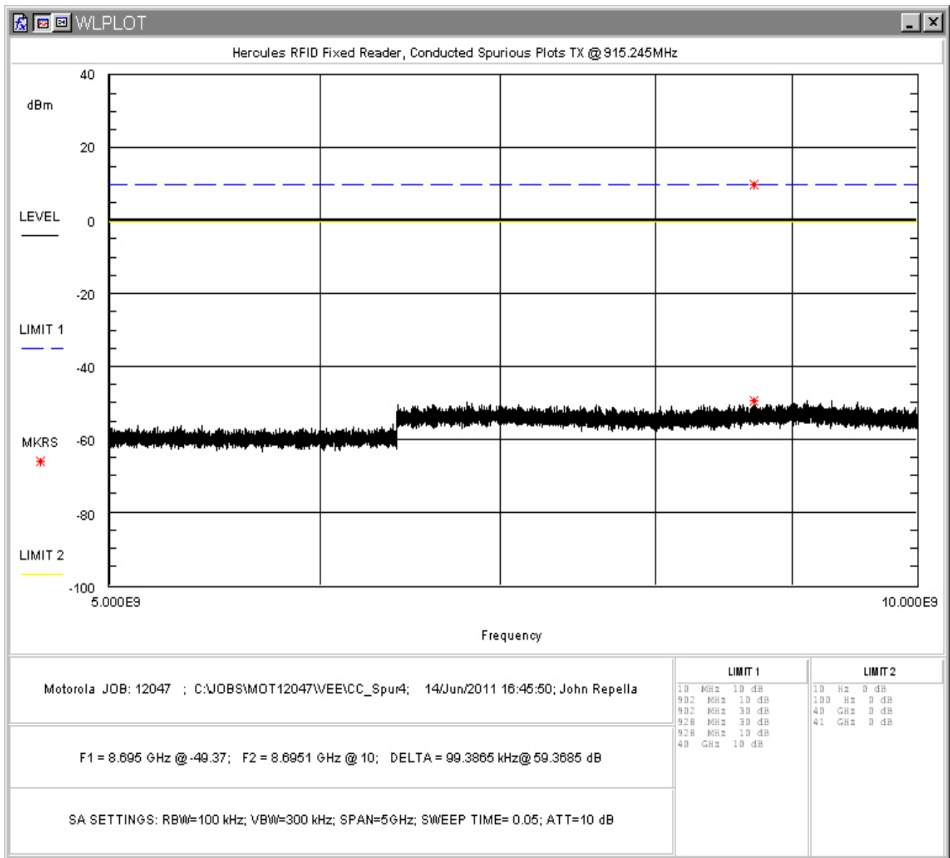
Figure 27: Conducted Spurious Emissions, Mid Channel 5 - 10GHz
