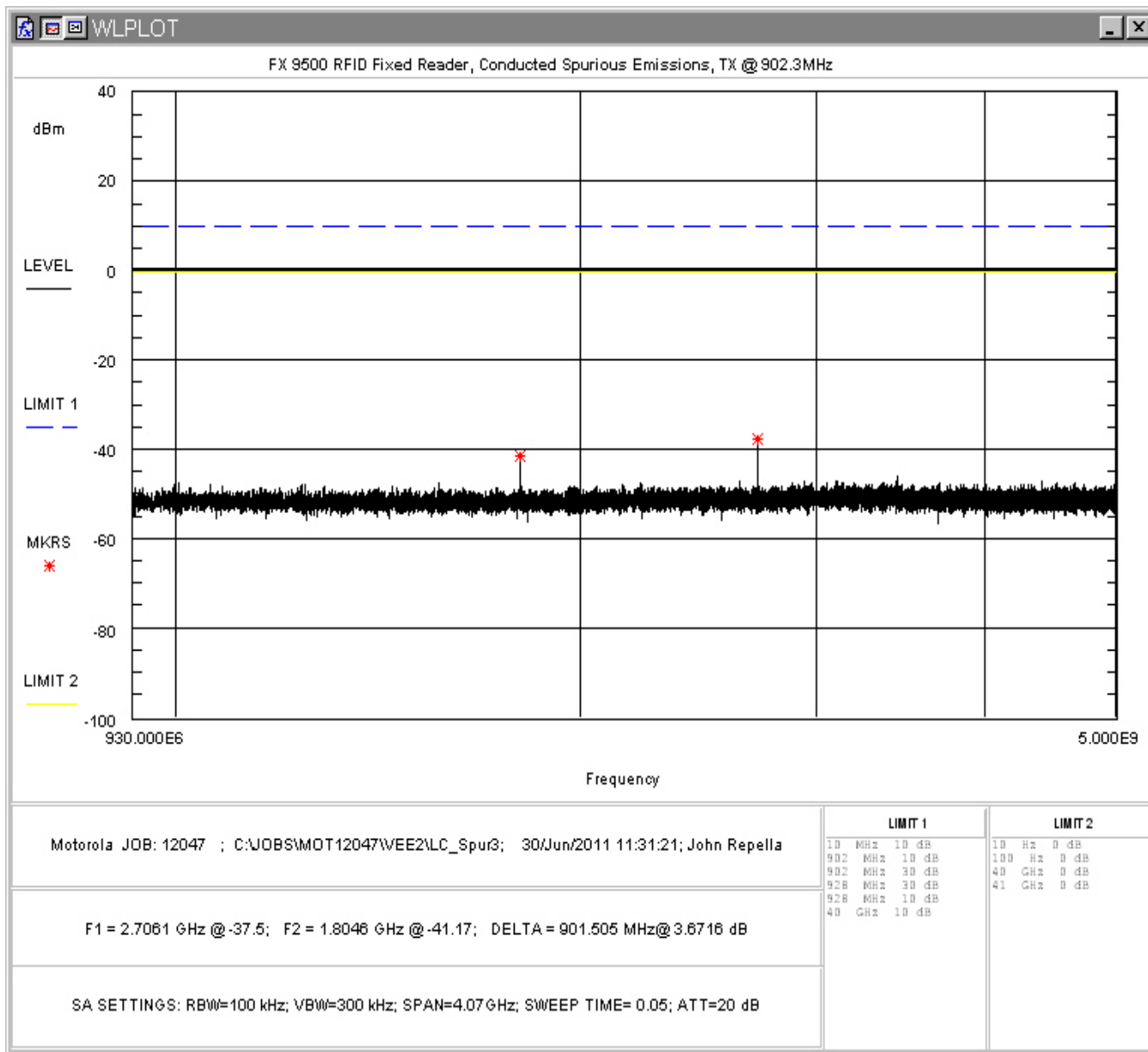
Figure 22: Conducted Spurious Emissions, Low Channel 930MHz – 5GHz
