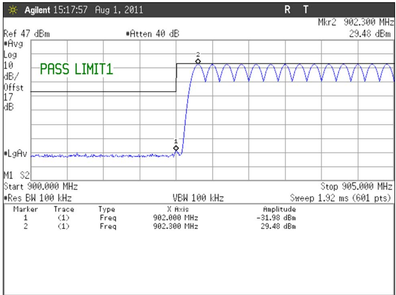
Figure 21: Band Edge Plot (Non-Hopping), Low Channel TX @902.3MHz
