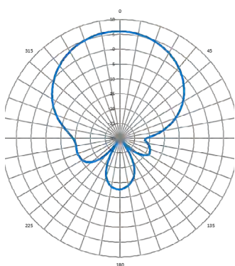
Horizontal (FCC)
