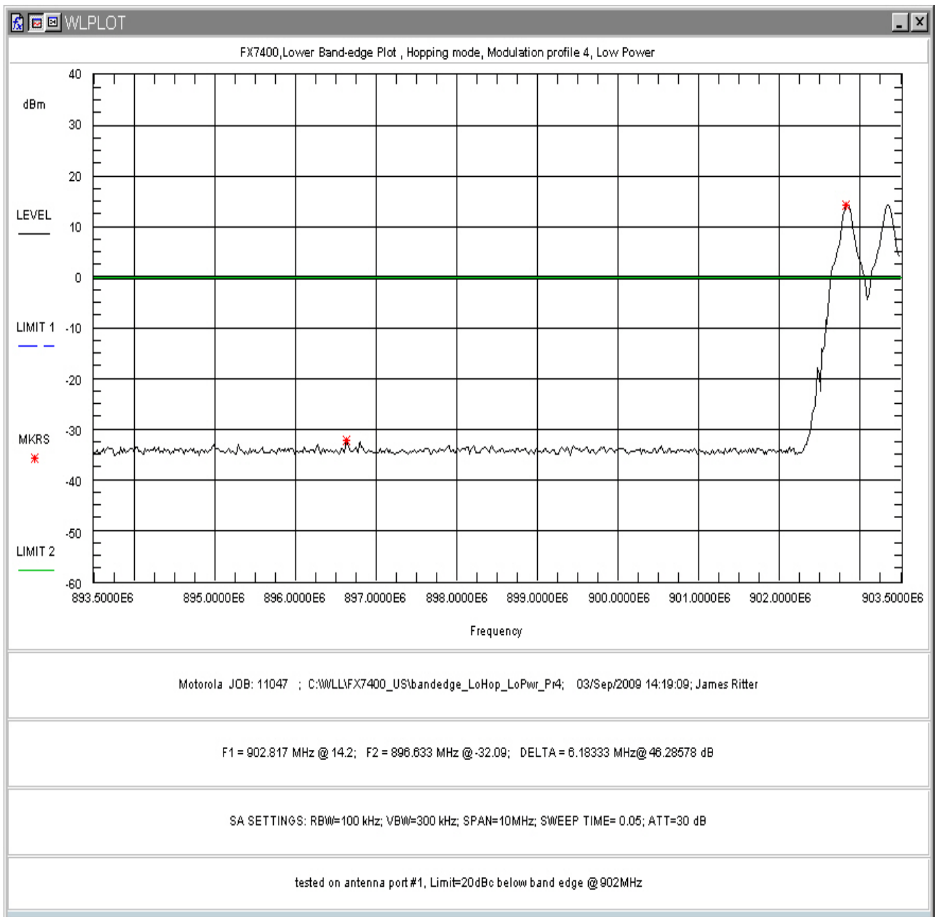
Figure 183: Lower Band-edge Hopping, Low Power, Modulation Profile 4
