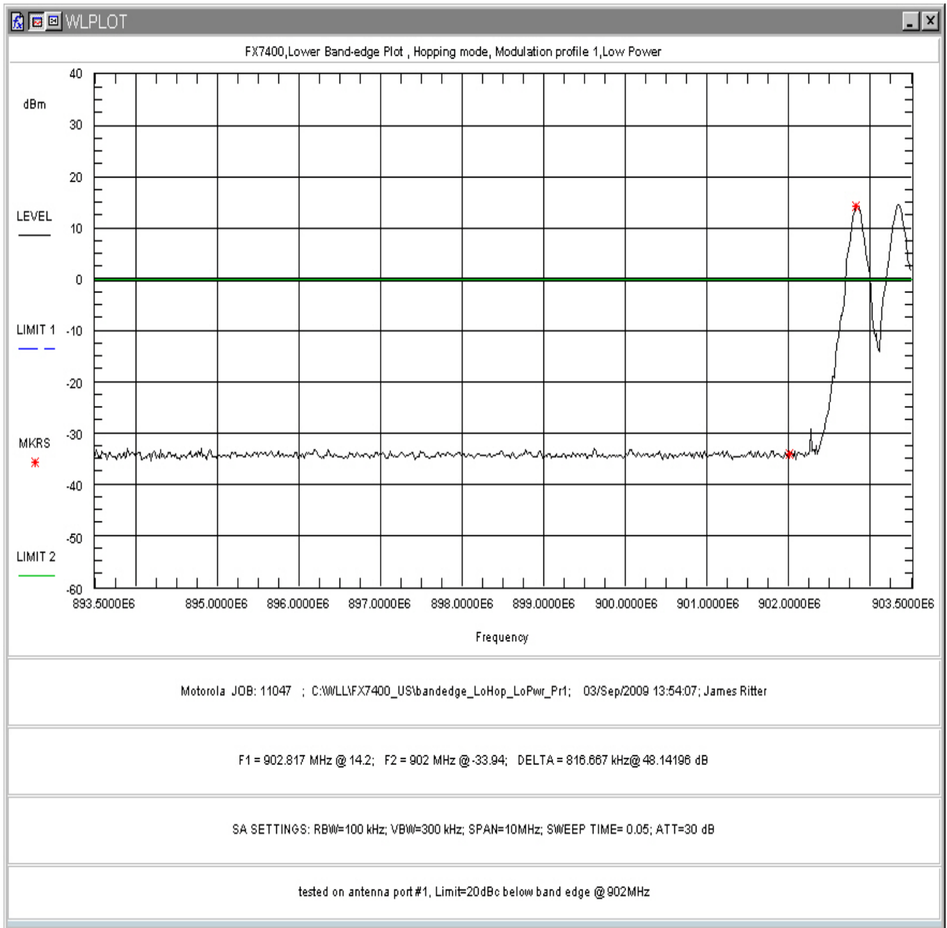
Figure 180: Lower Band-edge Hopping, Low Power, Modulation Profile 1
