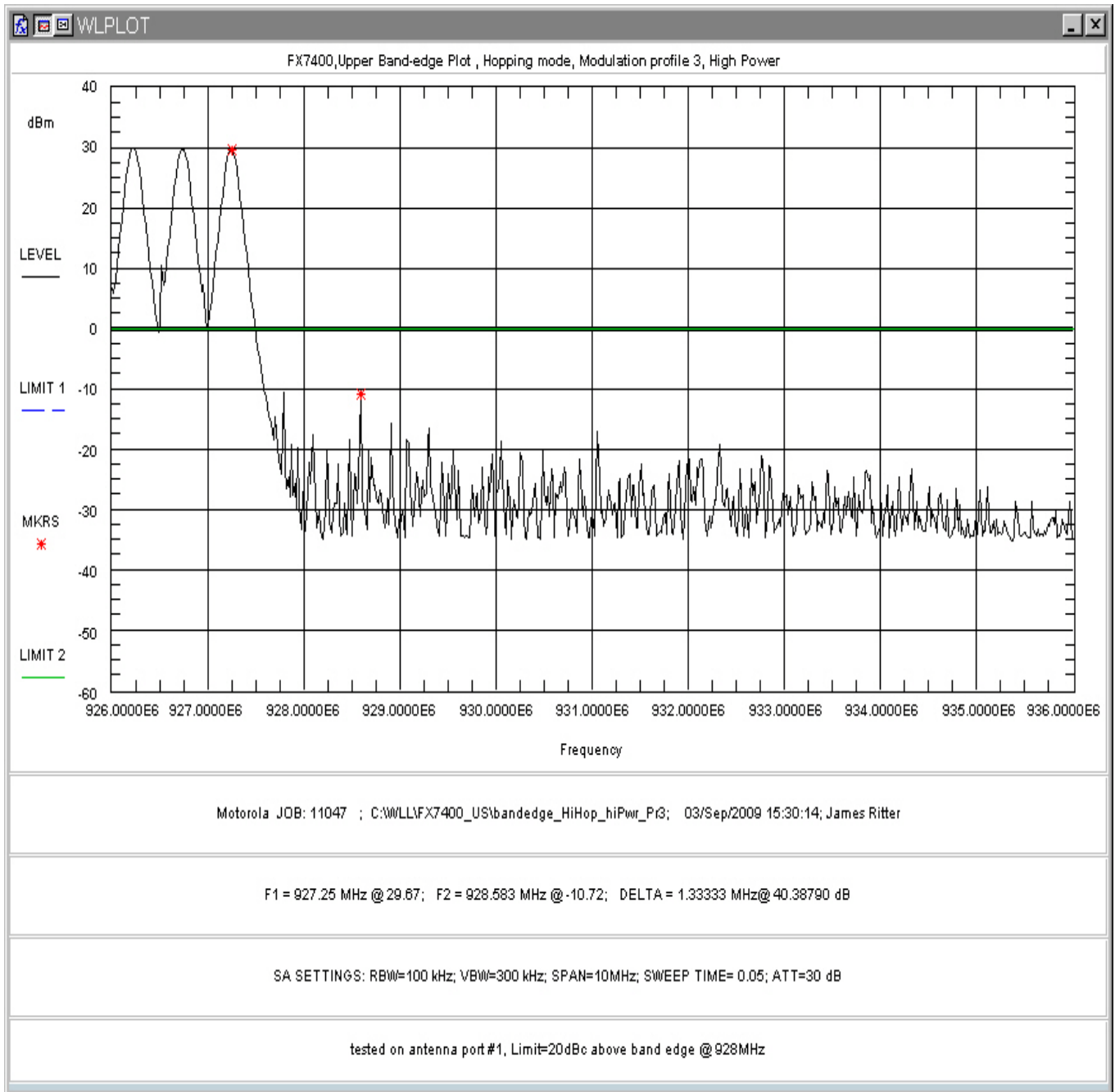
Figure 158: Upper Band-edge Hopping, High Power, Modulation Profile 3
