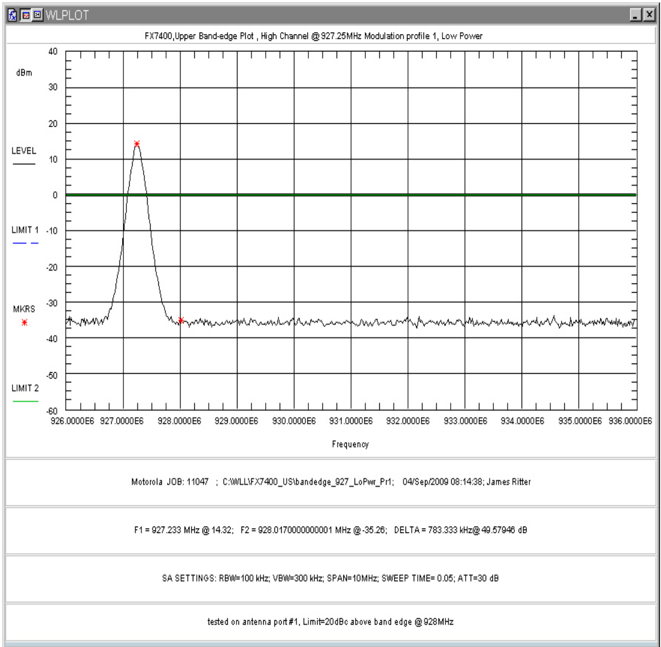
Figure 172: High Band-edge Non-hopping, Low Power, Modulation Profile 1
