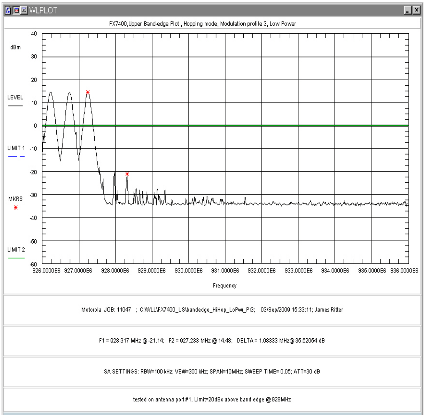
Figure 190: Upper Band-edge Hopping, Low Power, Modulation Profile 3
