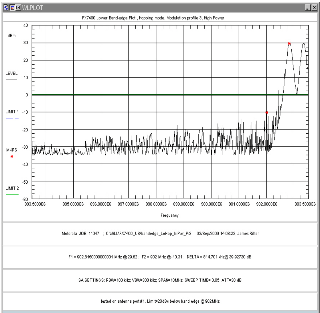
Figure 150: Lower Band-edge Hopping, High Power, Modulation Profile 3
