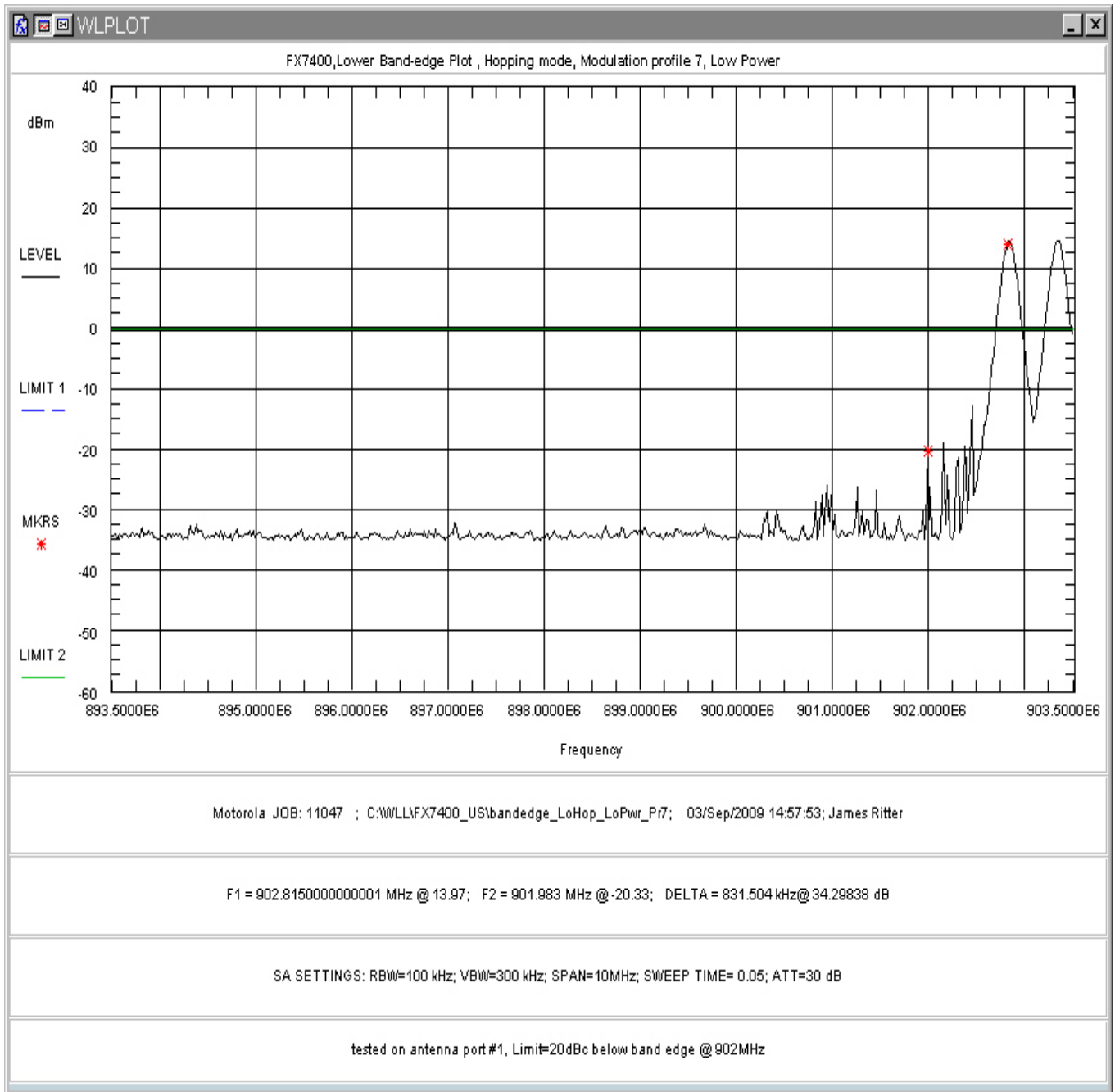
Figure 186: Lower Band-edge Hopping, Low Power, Modulation Profile 7
