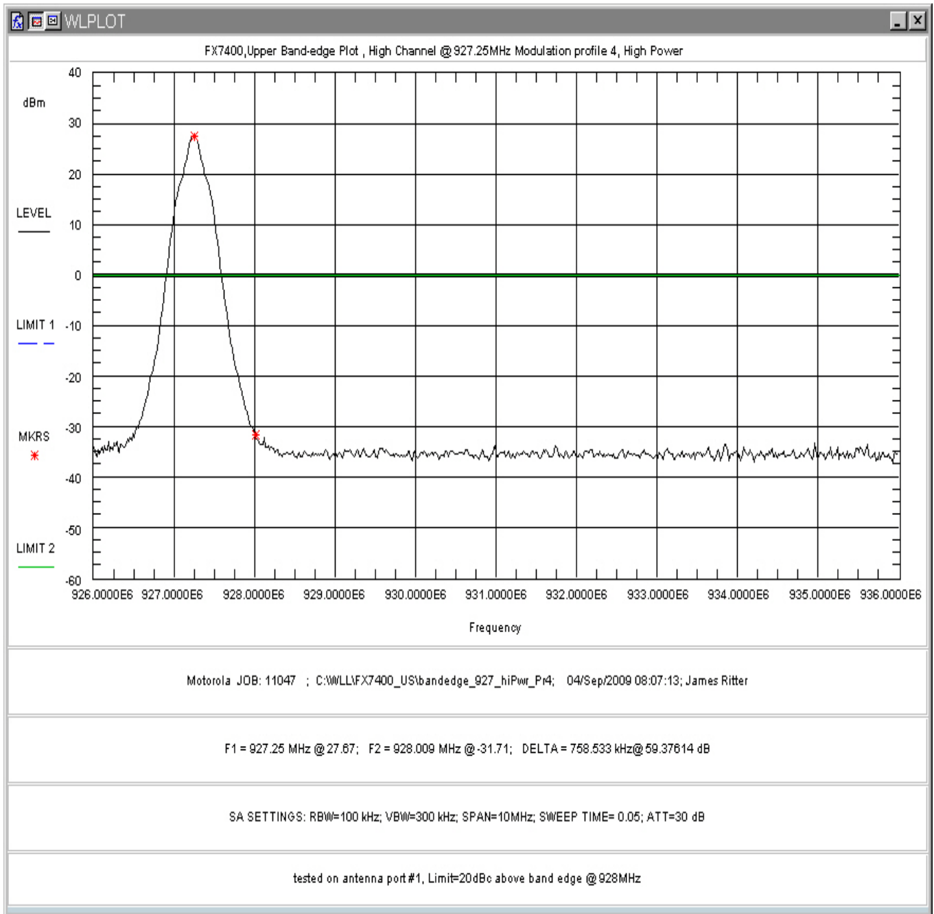
Figure 143: Upper Band-edge Non-hopping, High Power, Modulation Profile 4
