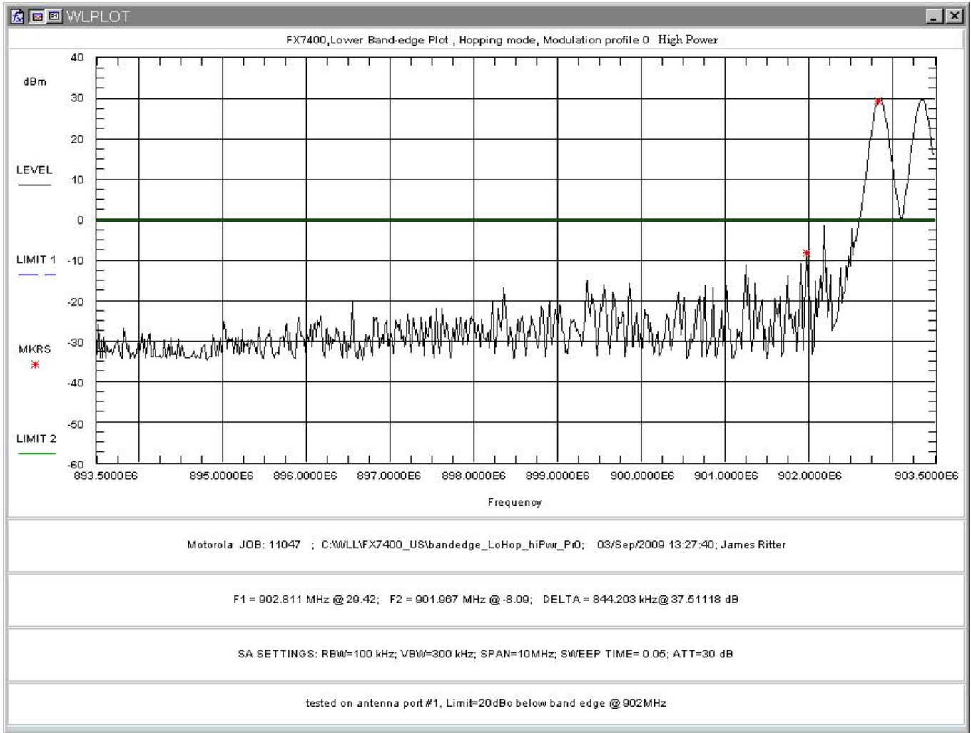
Figure 147: Lower Band-edge Hopping, High Power, Modulation Profile 0
