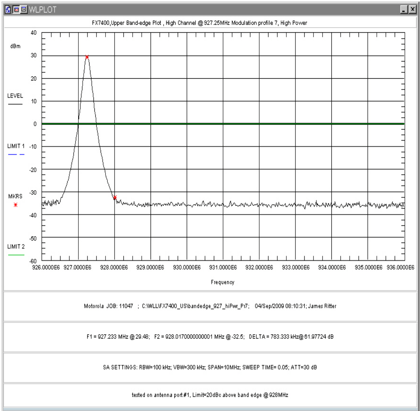
Figure 146: Upper Band-edge Non-hopping, High Power, Modulation Profile 7
