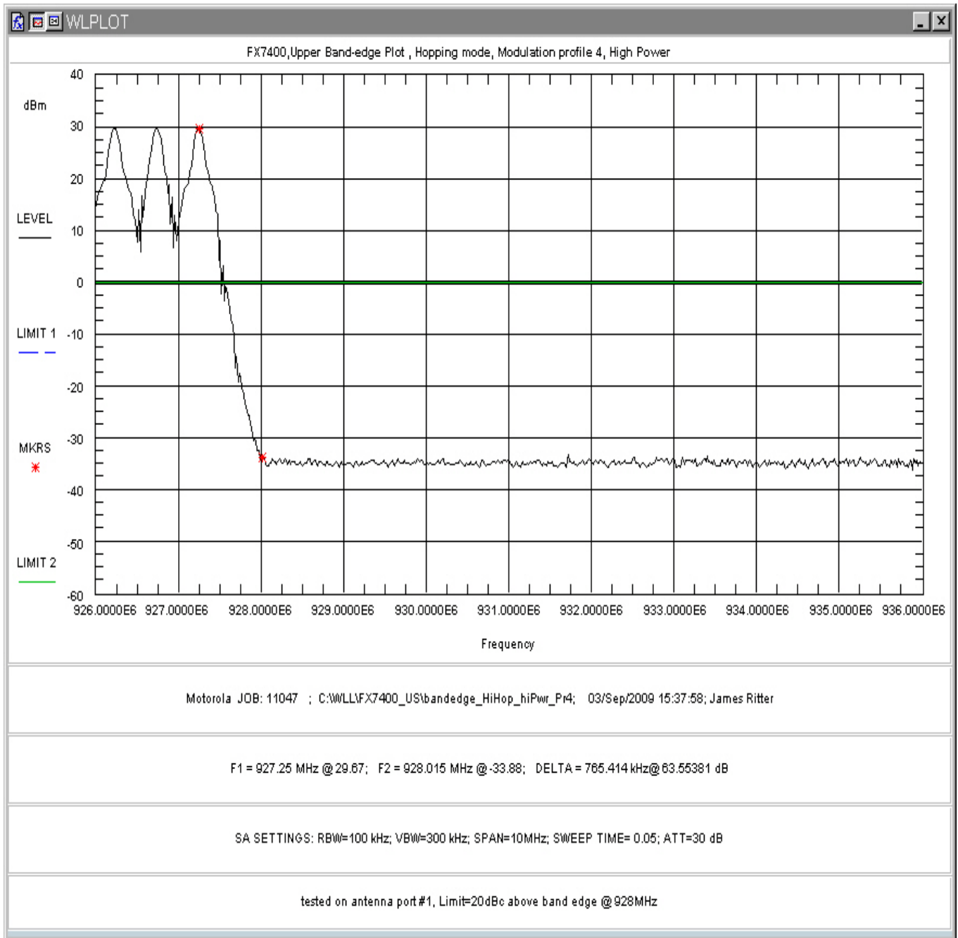
Figure 159: Upper Band-edge Hopping, High Power, Modulation Profile 4
