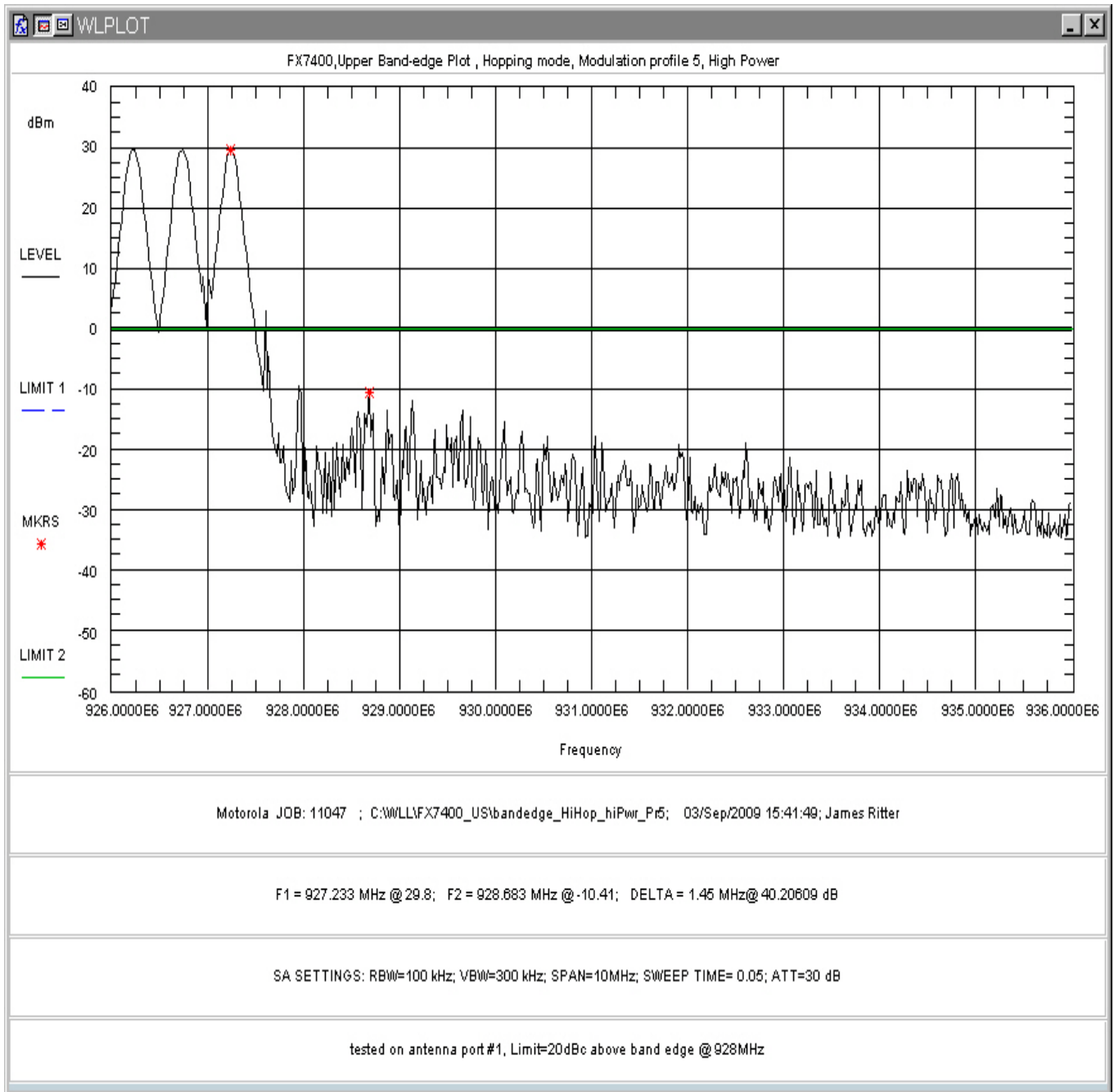
Figure 160: Upper Band-edge Hopping, High Power, Modulation Profile 5
