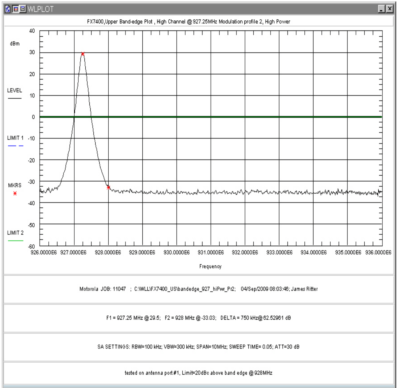
Figure 141: Upper Band-edge Non-hopping, High Power, Modulation Profile 2
