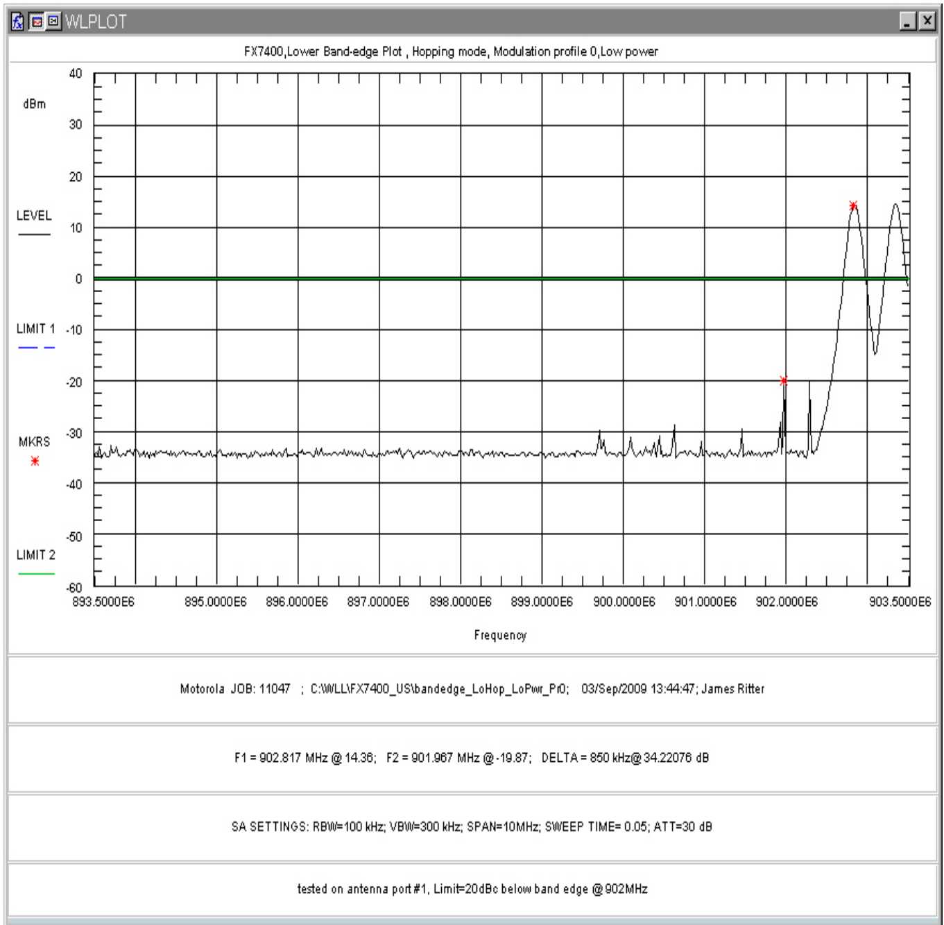
Figure 179: Lower Band-edge Hopping, Low Power, Modulation Profile 0
