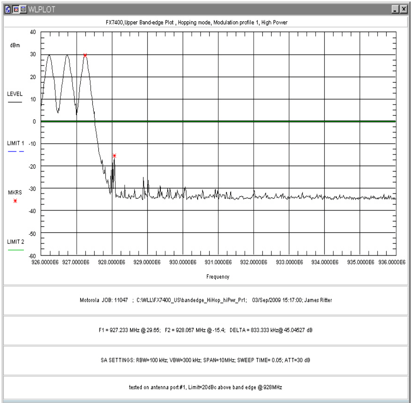
Figure 156: Upper Band-edge Hopping, High Power, Modulation Profile 1
