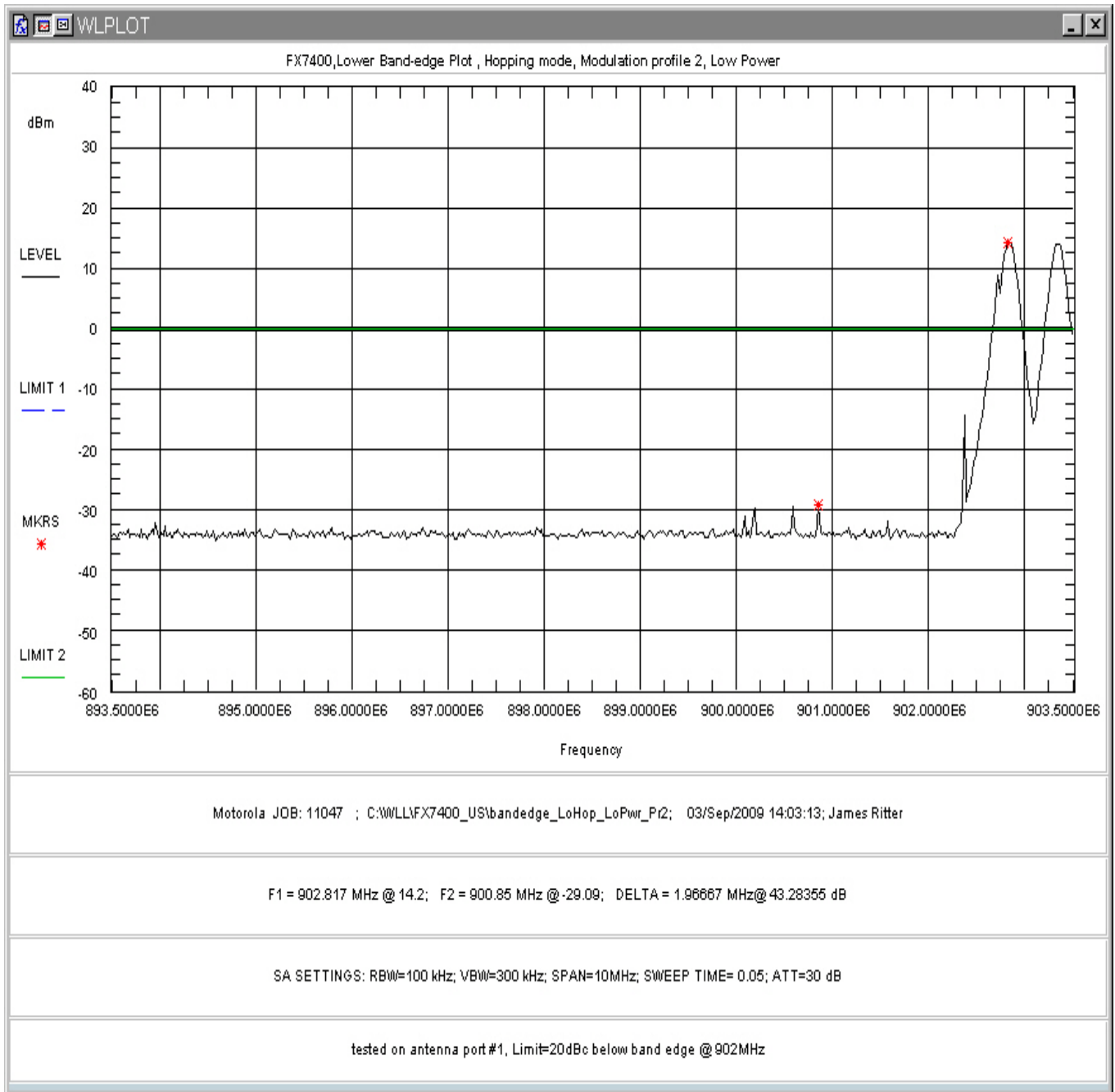
Figure 181: Lower Band-edge Hopping, Low Power, Modulation Profile 2
