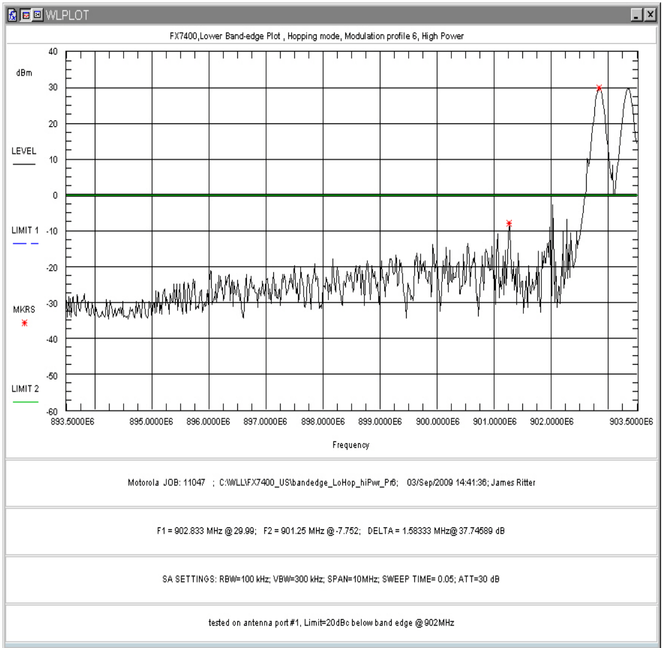
Figure 153: Lower Band-edge Hopping, High Power, Modulation Profile 6
