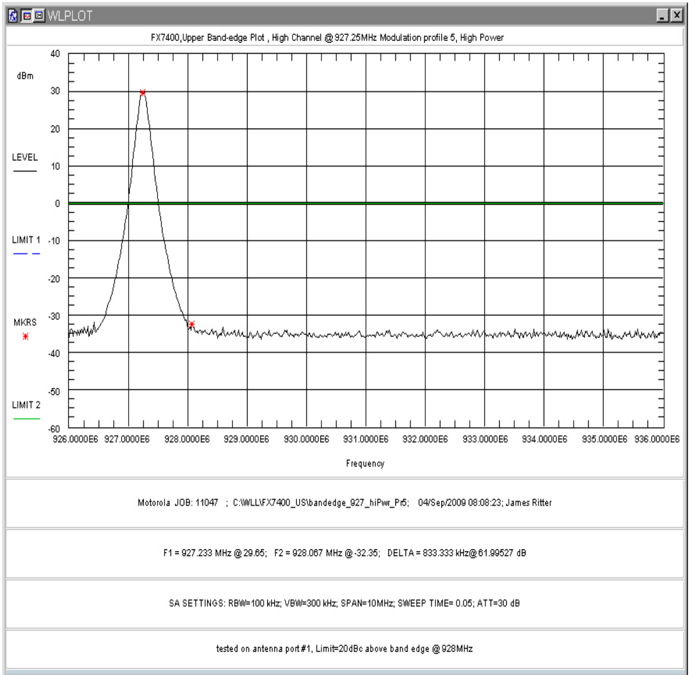
Figure 144: Upper Band-edge Non-hopping, High Power, Modulation Profile 5
