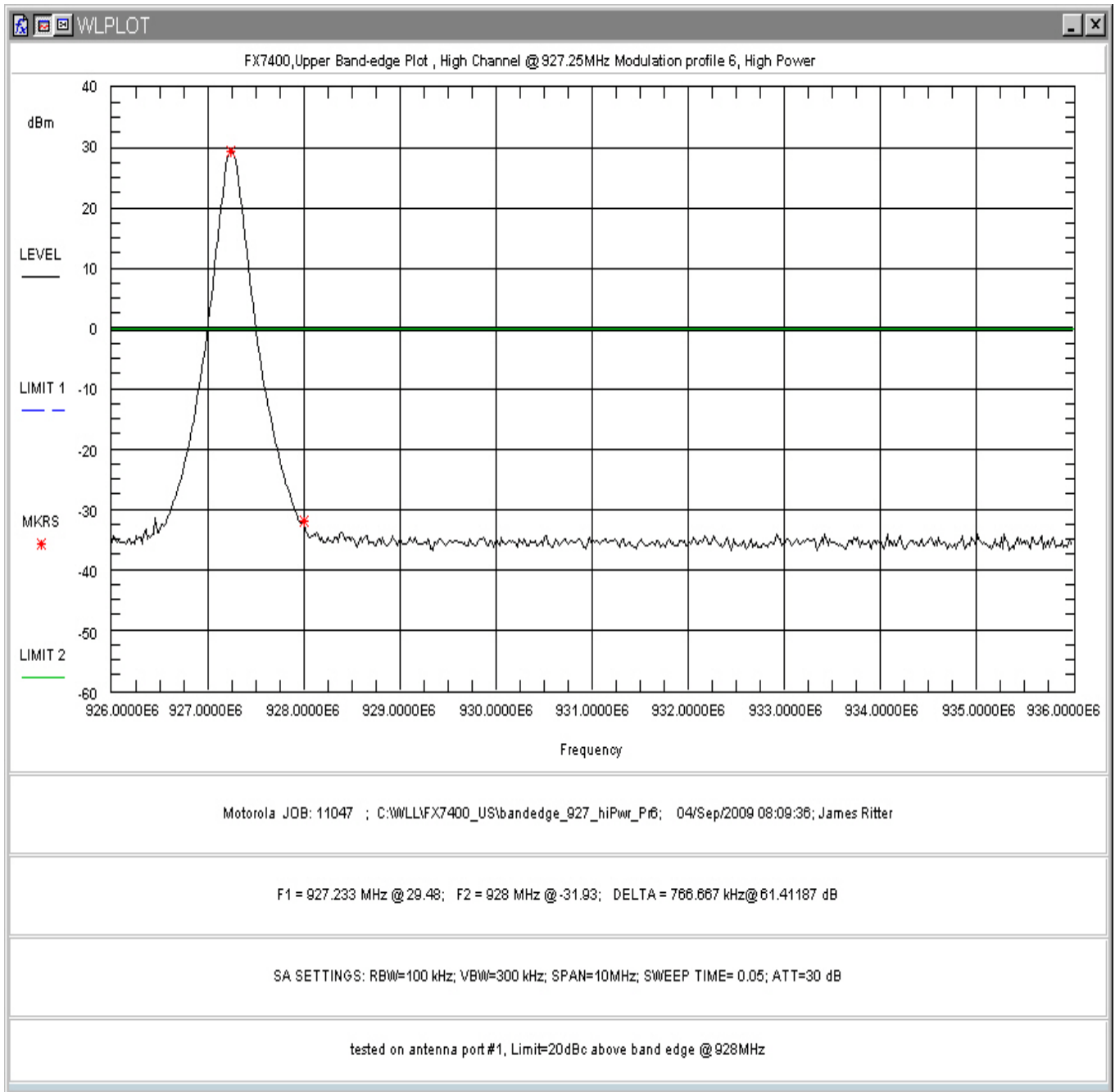
Figure 145: Upper Band-edge Non-hopping, High Power, Modulation Profile 6
