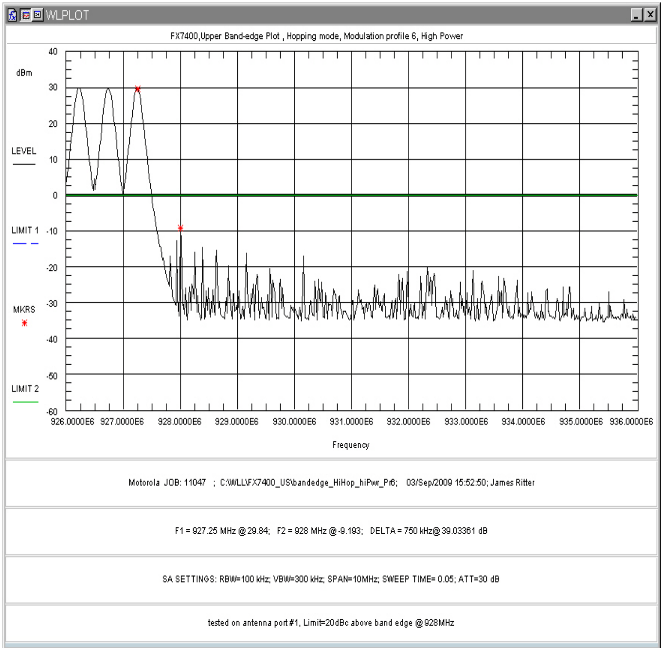
Figure 161: Upper Band-edge Hopping, High Power, Modulation Profile 6
