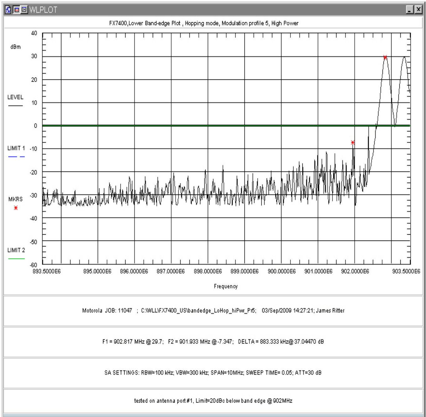
Figure 152: Lower Band-edge Hopping, High Power, Modulation Profile 5
