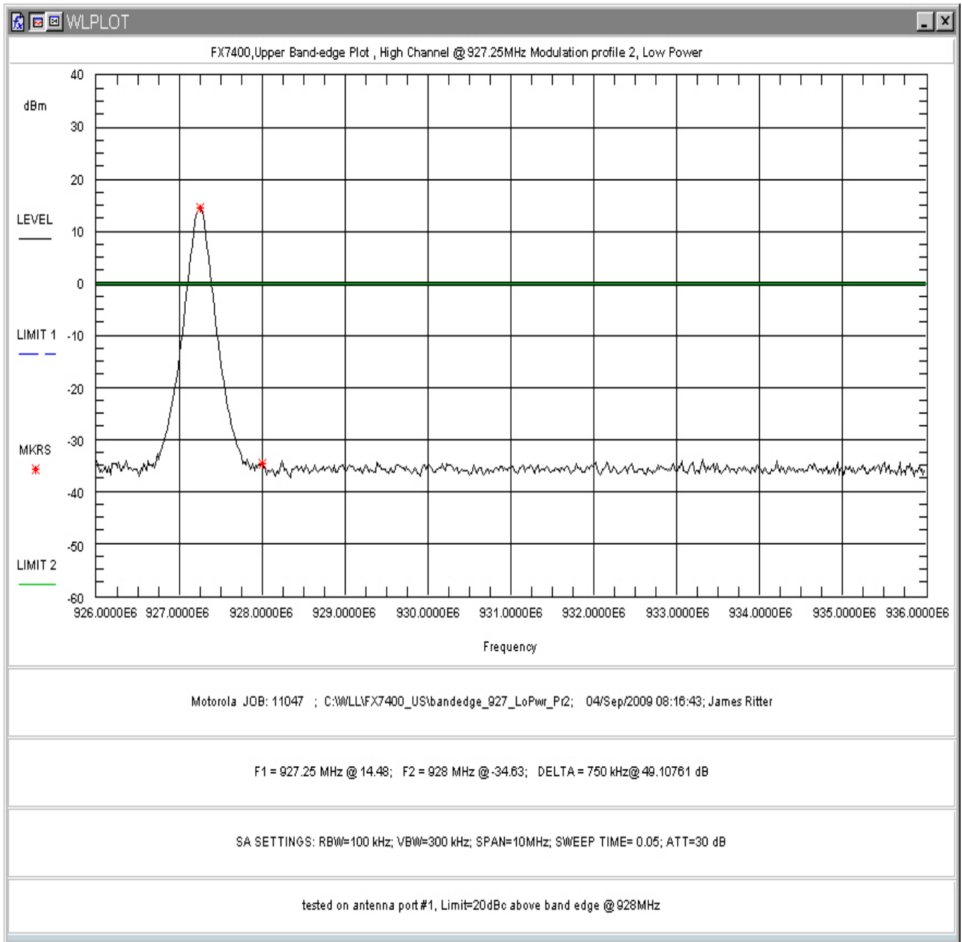
Figure 173: High Band-edge Non-hopping, Low Power, Modulation Profile 2
