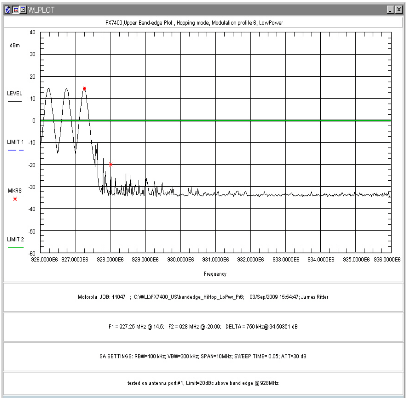
Figure 193: Upper Band-edge Hopping, Low Power, Modulation Profile 6
