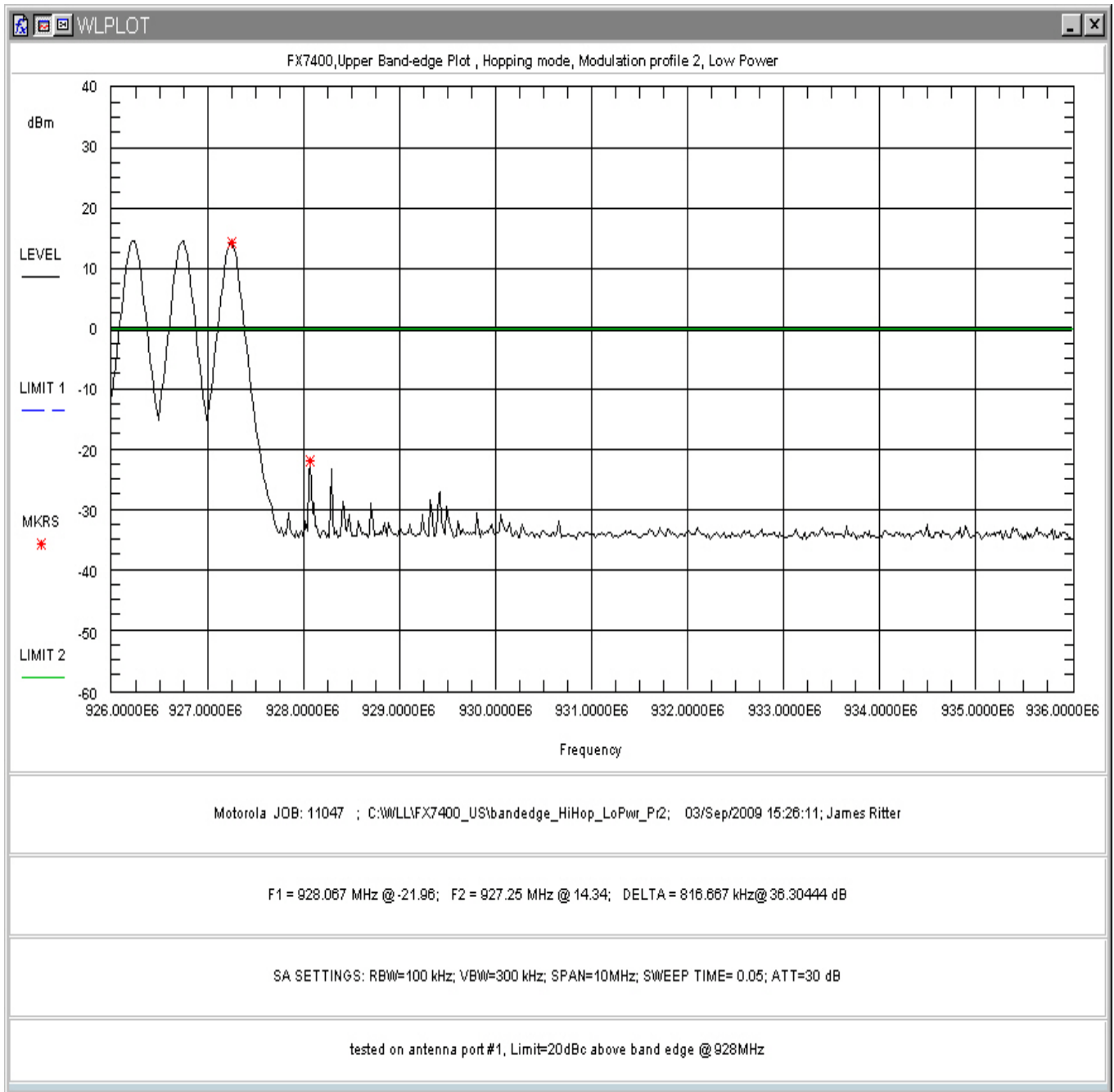
Figure 189: Upper Band-edge Hopping, Low Power, Modulation Profile 2
