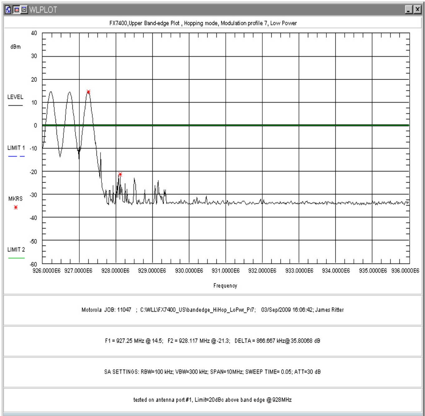
Figure 194: Upper Band-edge Hopping, Low Power, Modulation Profile 7
