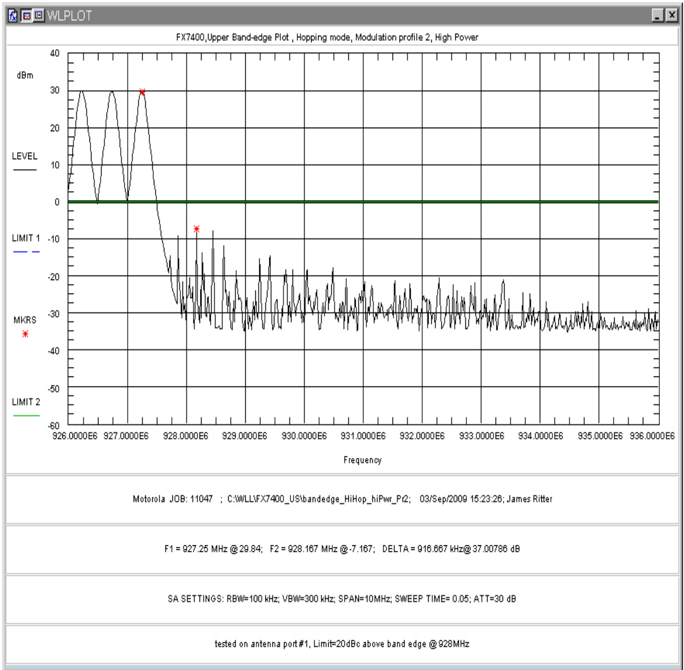
Figure 157: Upper Band-edge Hopping, High Power, Modulation Profile 2
