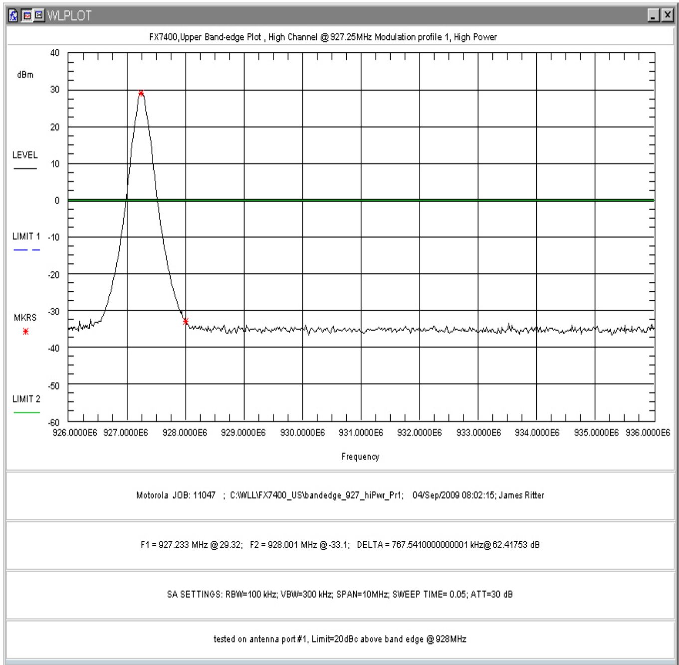
Figure 140: Upper Band-edge Non-hopping, High Power, Modulation Profile 1
