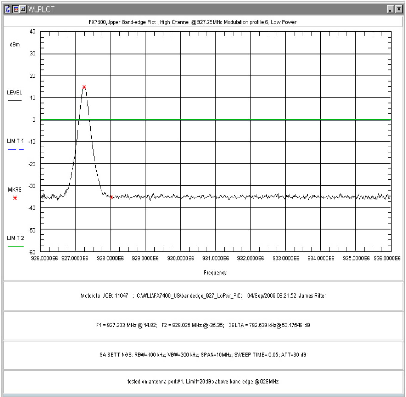
Figure 177: High Band-edge Non-hopping, Low Power, Modulation Profile 6
