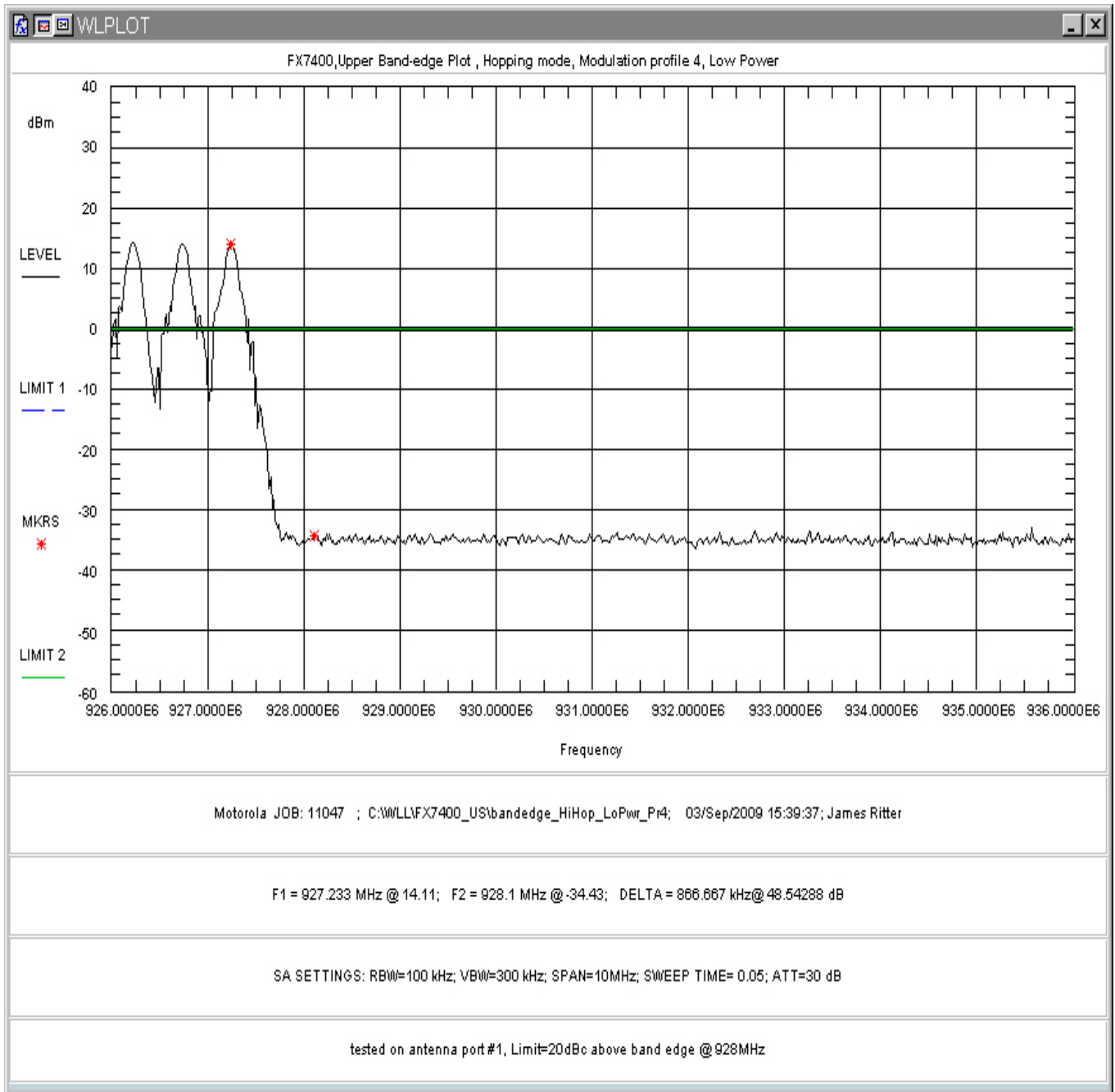
Figure 191: Upper Band-edge Hopping, Low Power, Modulation Profile 4
