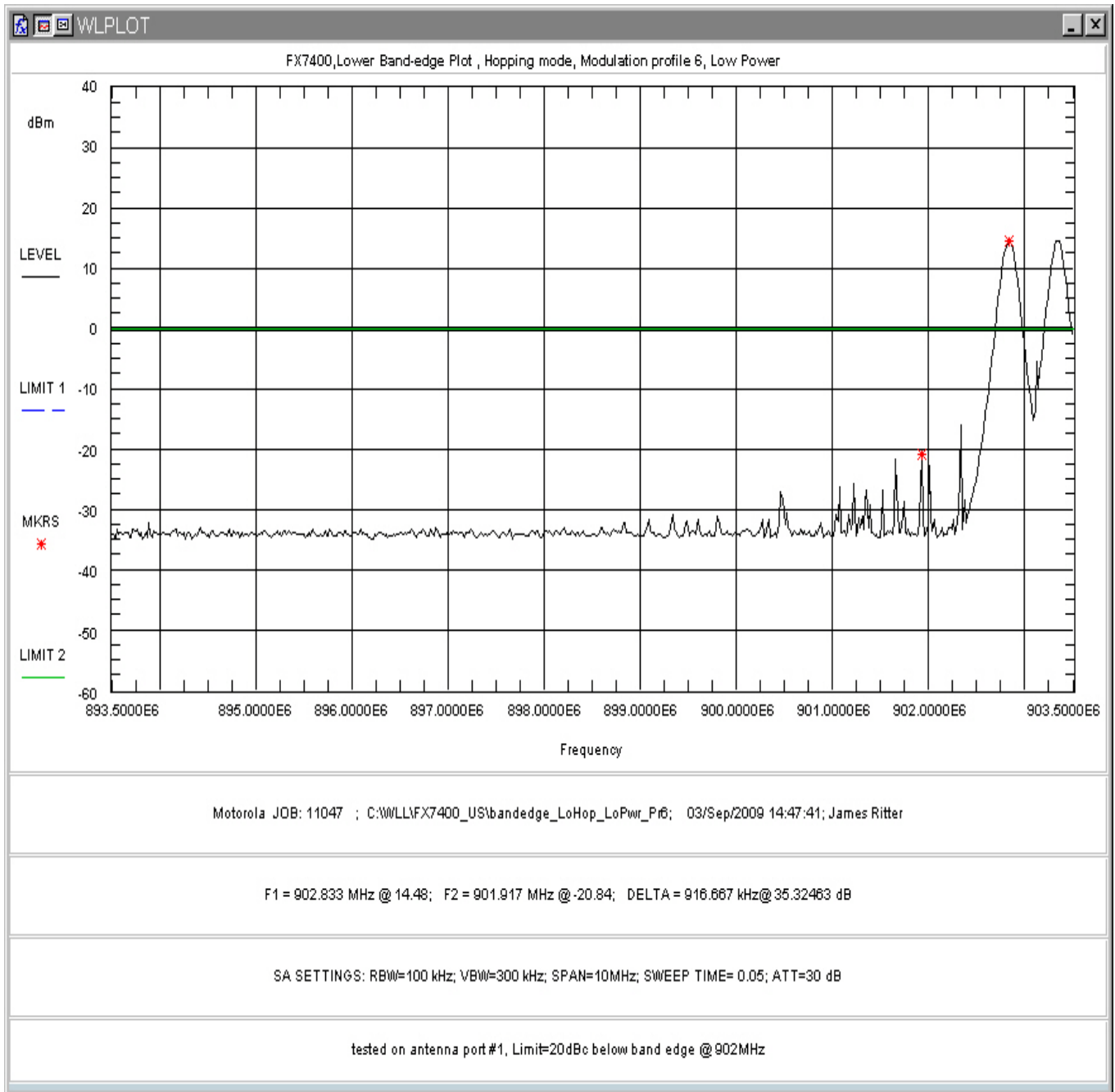
Figure 185: Lower Band-edge Hopping, Low Power, Modulation Profile 6
