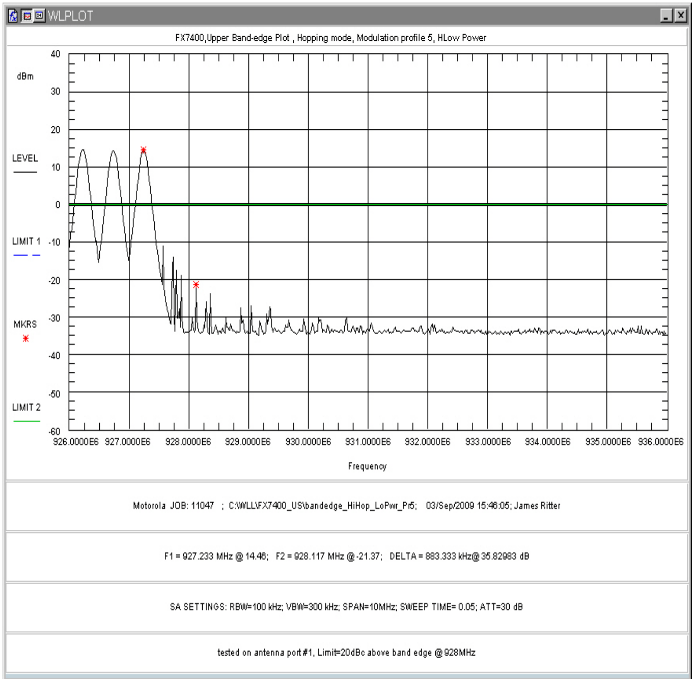
Figure 192: Upper Band-edge Hopping, Low Power, Modulation Profile 5
