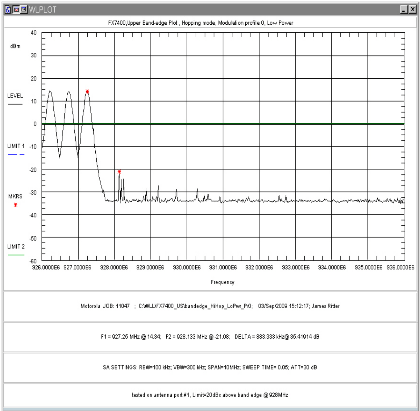
Figure 187: Upper Band-edge Hopping, Low Power, Modulation Profile 0
