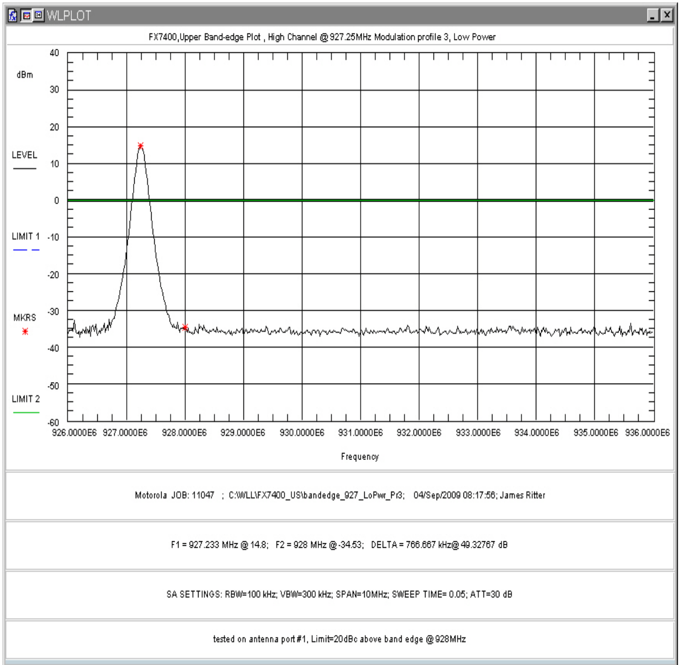
Figure 174: High Band-edge Non-hopping, Low Power, Modulation Profile 3
