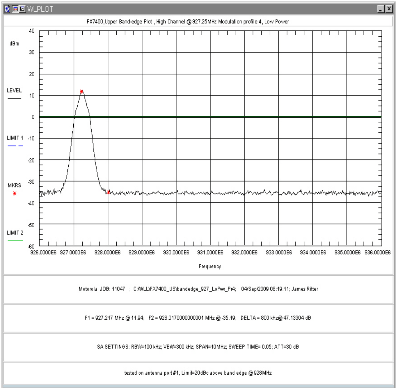
Figure 175: High Band-edge Non-hopping, Low Power, Modulation Profile 4
