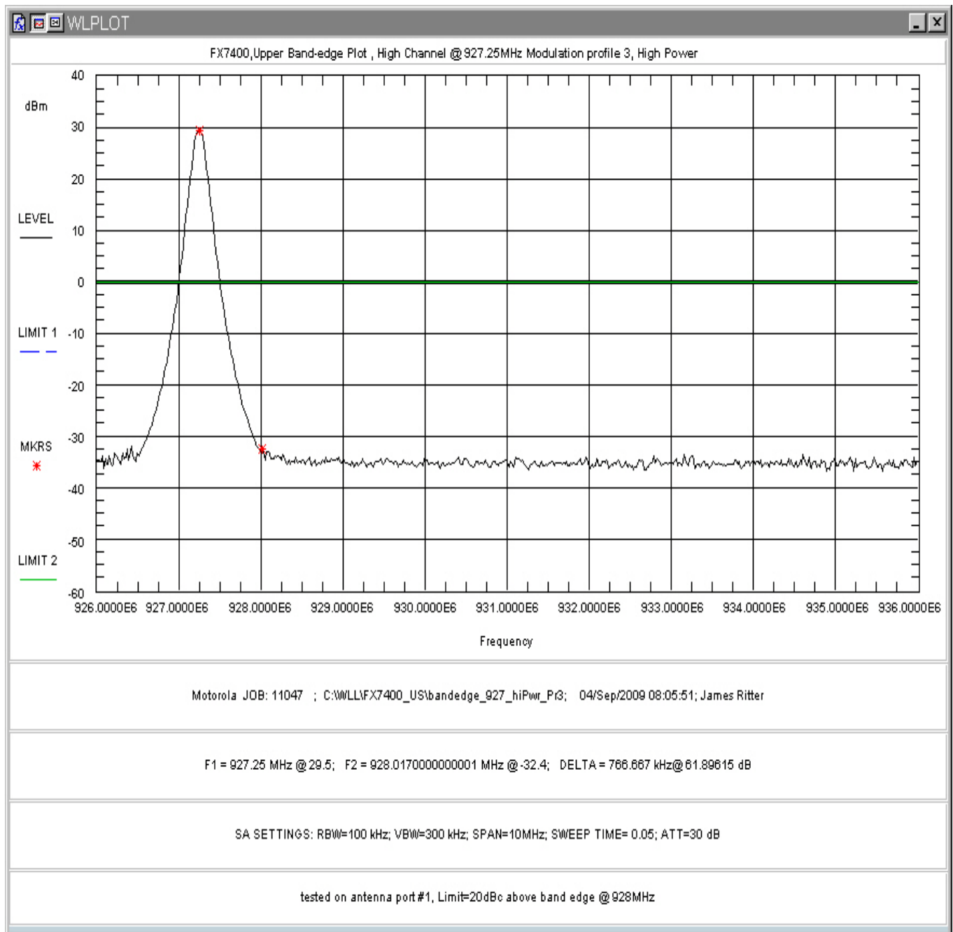
Figure 142: Upper Band-edge Non-hopping, High Power, Modulation Profile 3
