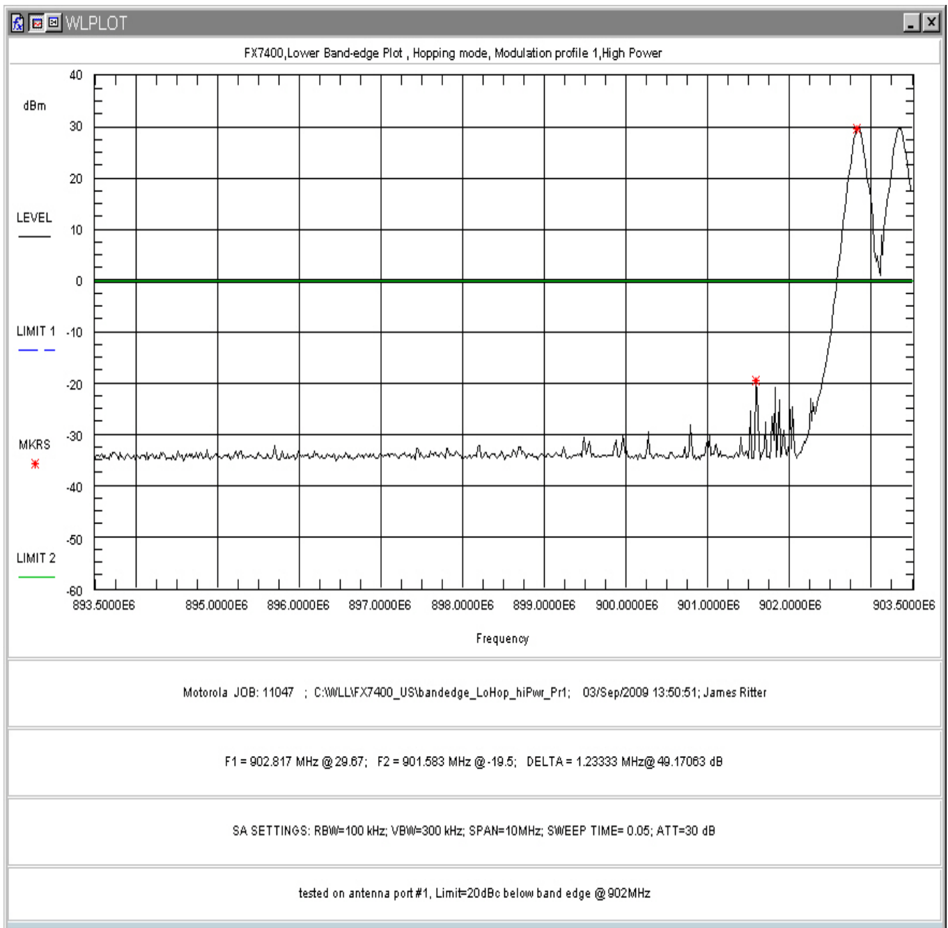
Figure 148: Lower Band-edge Hopping, High Power, Modulation Profile 1
