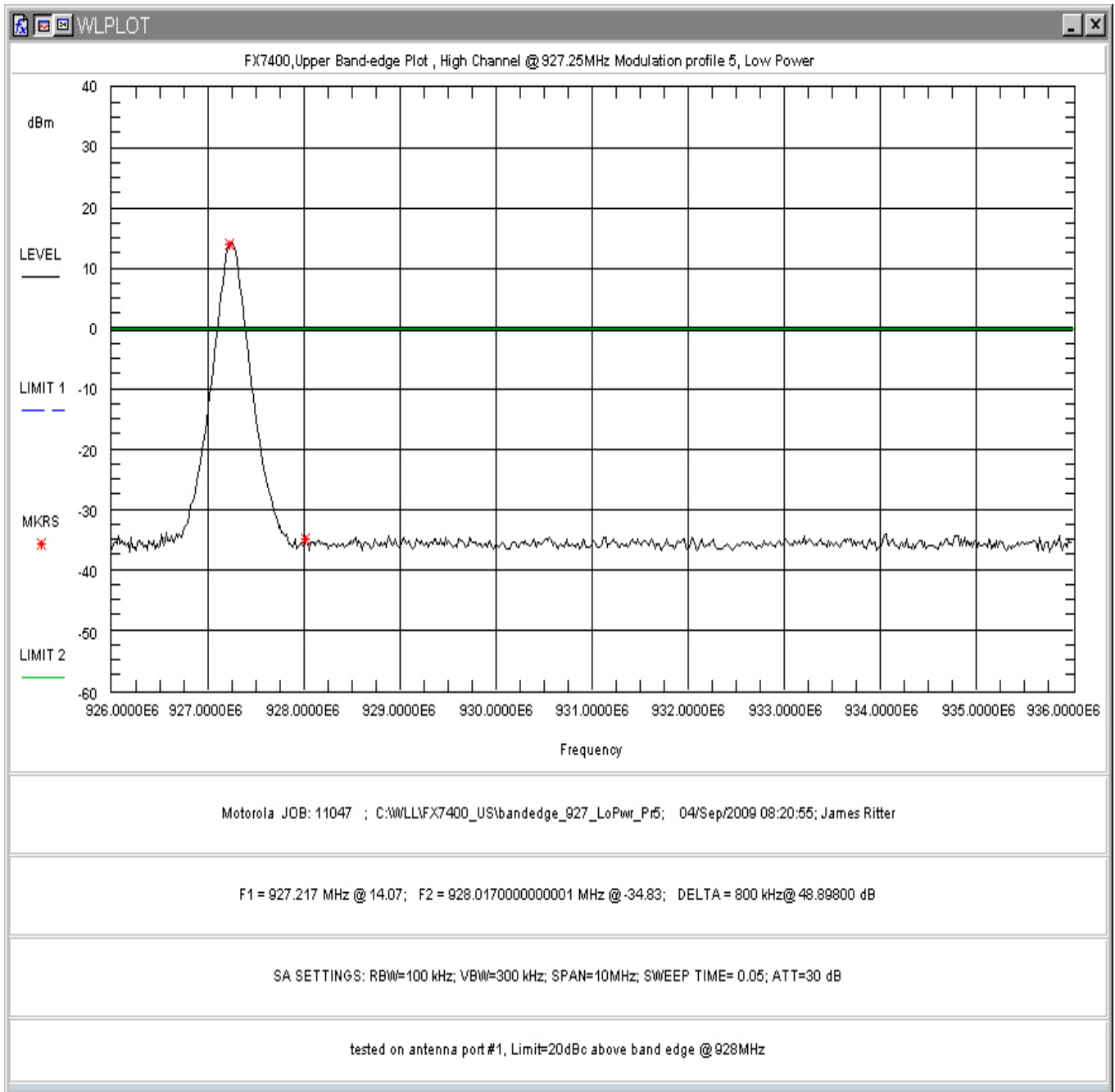
Figure 176: High Band-edge Non-hopping, Low Power, Modulation Profile 5
