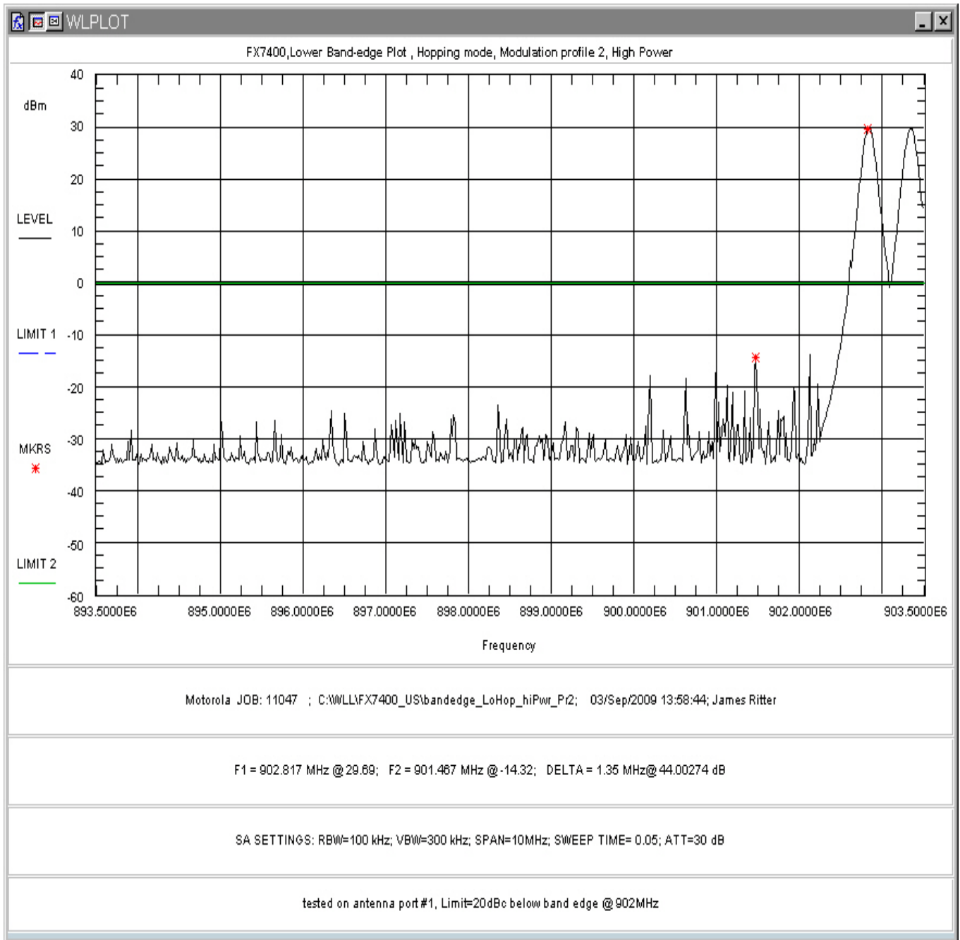
Figure 149: Lower Band-edge Hopping, High Power, Modulation Profile 2
