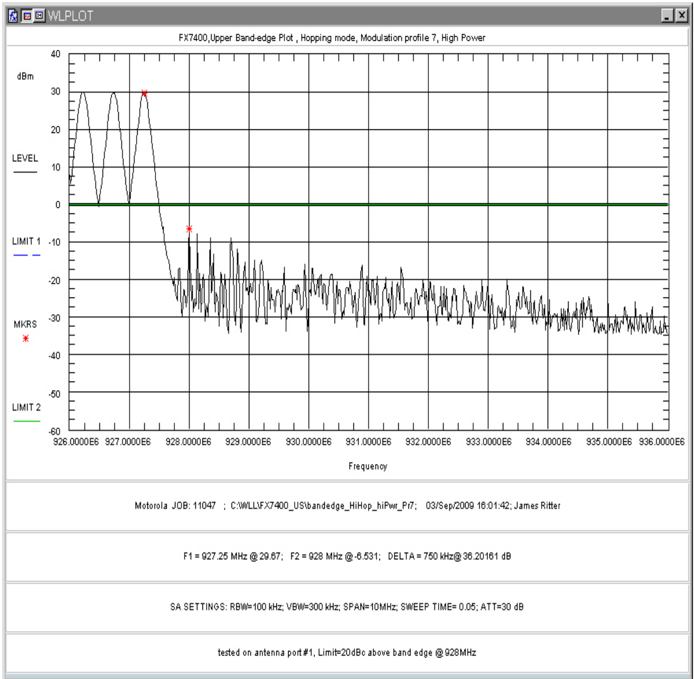
Figure 162: Upper Band-edge Hopping, High Power, Modulation Profile 7
