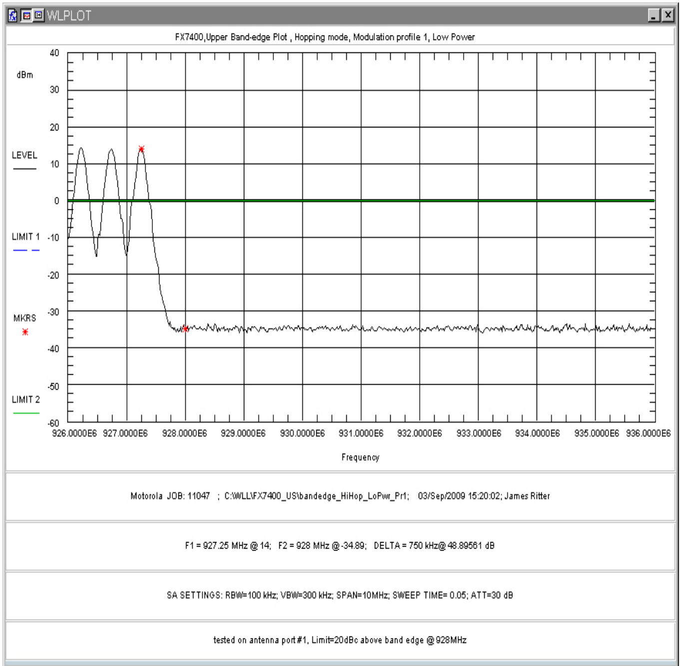
Figure 188: Upper Band-edge Hopping, Low Power, Modulation Profile 1
