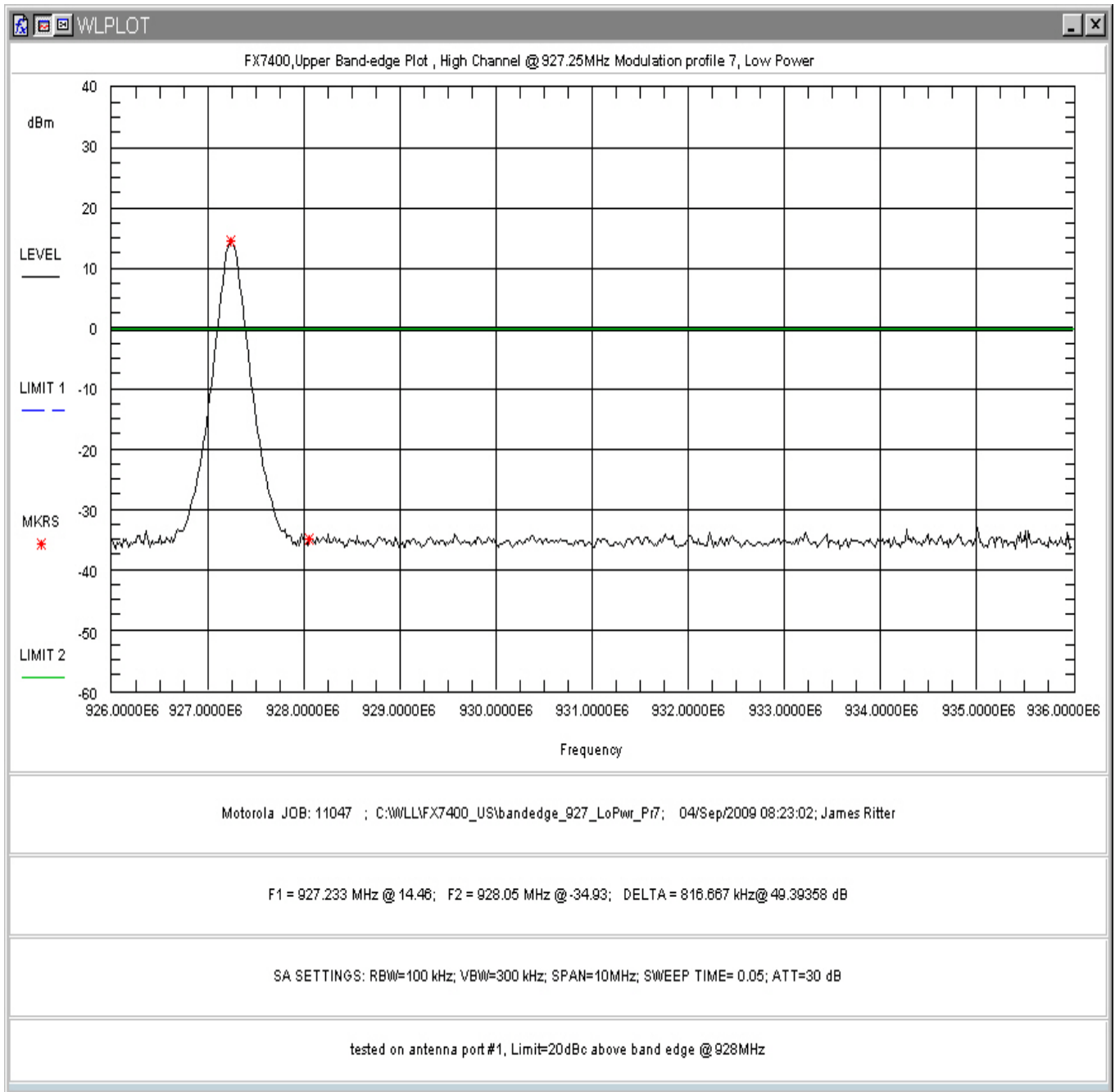
Figure 178: High Band-edge Non-hopping, Low Power, Modulation Profile 7
