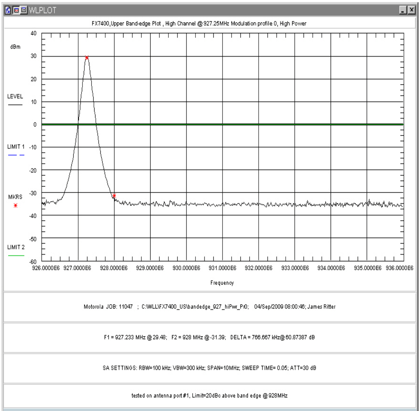
Figure 139: Upper Band-edge Non-hopping, High Power, Modulation Profile 0
