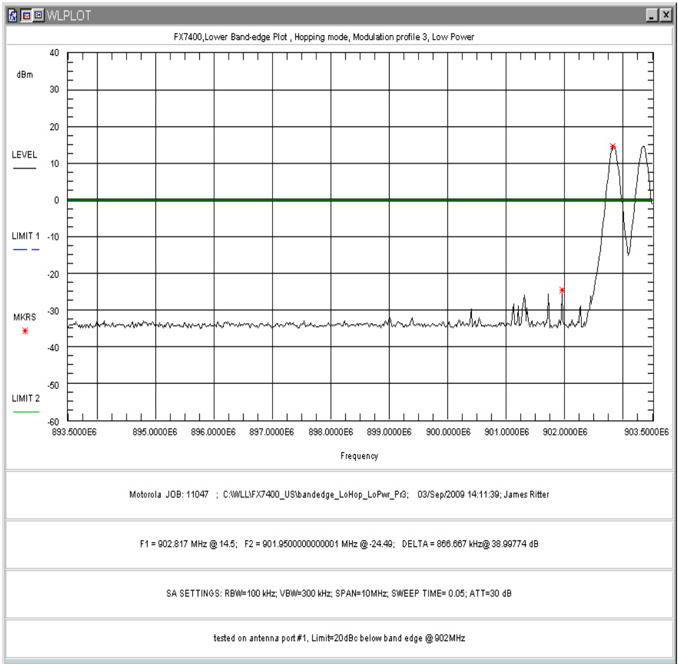
Figure 182: Lower Band-edge Hopping, Low Power, Modulation Profile 3
