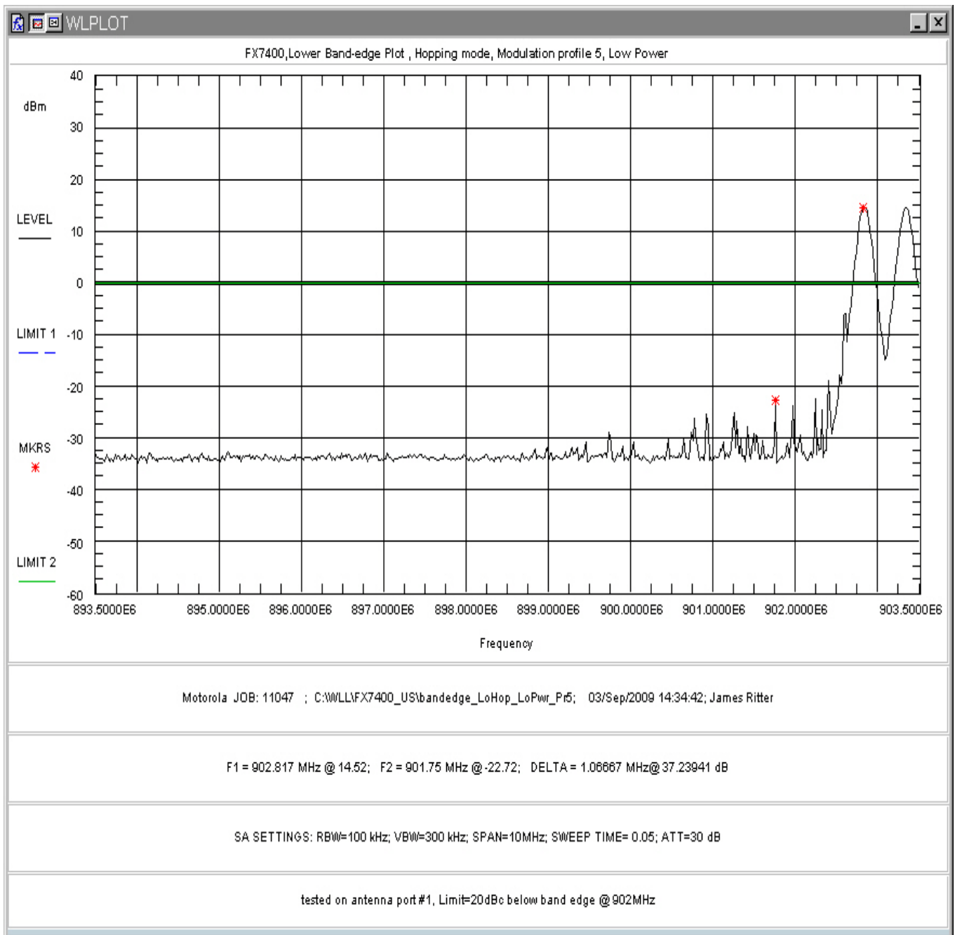
Figure 184: Lower Band-edge Hopping, Low Power, Modulation Profile 5
