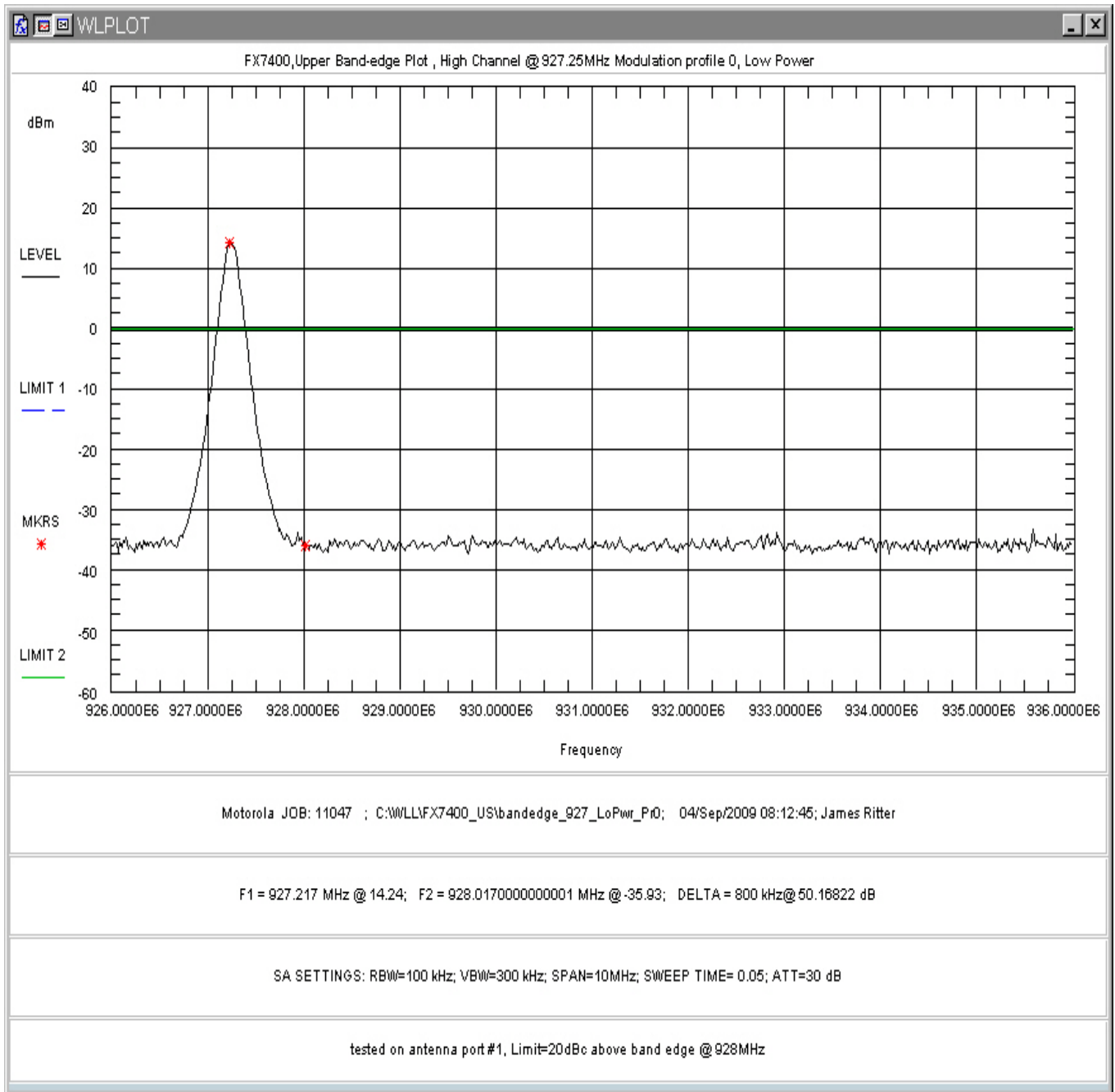
Figure 171: High Band-edge Non-hopping, Low Power, Modulation Profile 0
