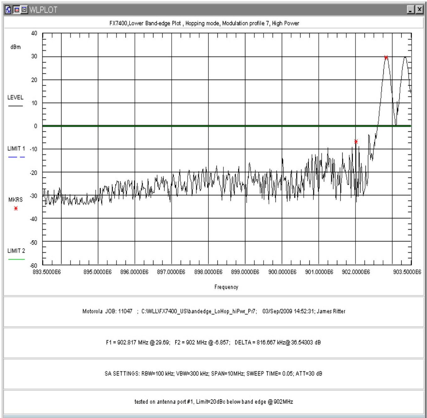
Figure 154: Lower Band-edge Hopping, High Power, Modulation Profile 7
