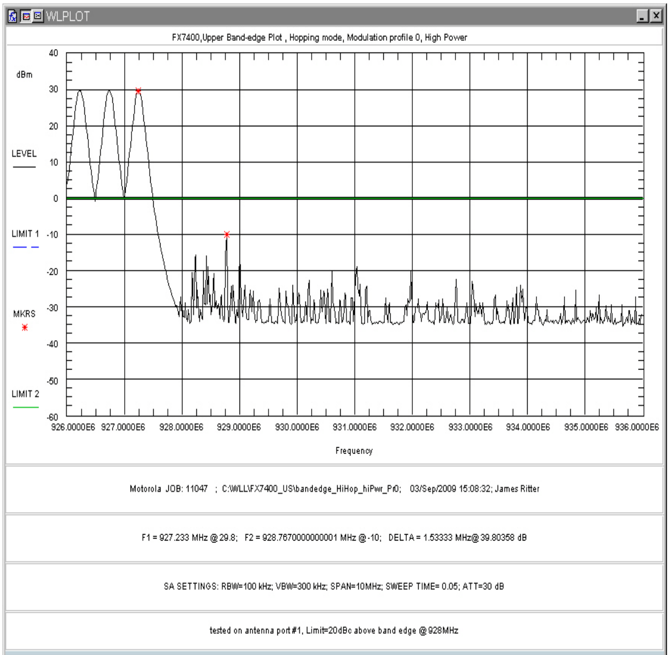
Figure 155: Upper Band-edge Hopping, High Power, Modulation Profile 0
