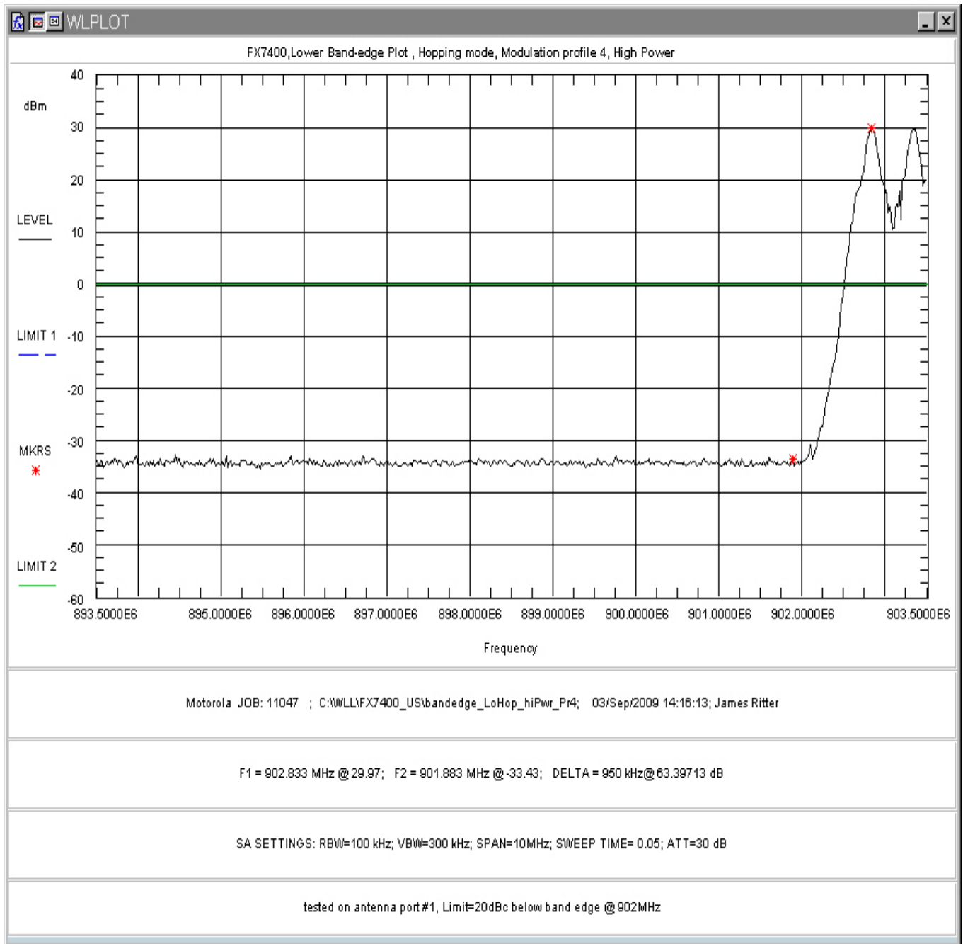
Figure 151: Lower Band-edge Hopping, High Power, Modulation Profile 4
