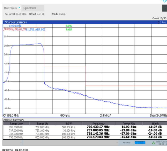
1-N13-PC3-15-5-H-6-CP-QPSK-Outer_Full-25@0-Ant0-PASS-see graph
