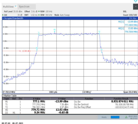
1-N13--15-10-M-4-DFT-64QAM-Outter_Full-50@0-Ant0-8.932-9.540-≤10-PASS
