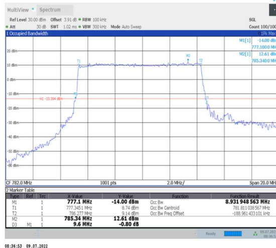
1-N13--15-10-M-3-DFT-16QAM-Outter_Full-50@0-Ant0-8.932-9.600-≤10-PASS
