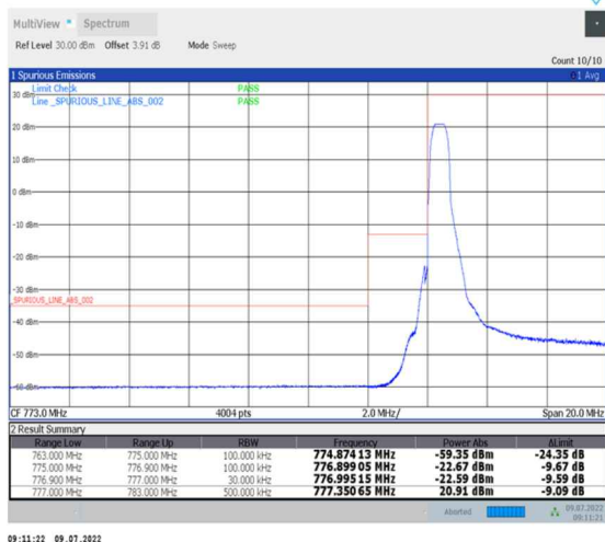
1-N13-PC3-15-10-L-4-CP-QPSK-Edge_1RB_Left-1@0-Ant0-PASS-see graph
