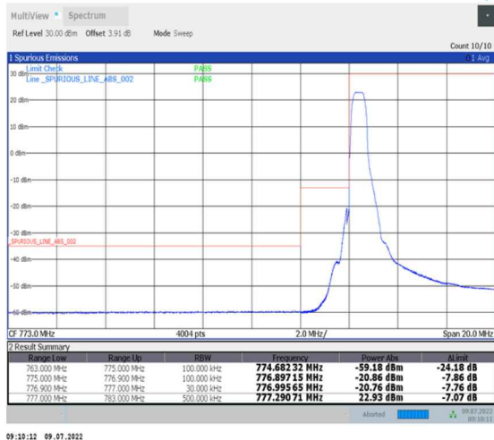
1-N13-PC3-15-10-L-1-DFT-PI2BPSK-Edge_1RB_Left-1@0-Ant0-PASS-see graph
