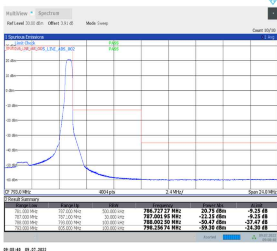
1-N13-PC3-15-5-H-5-CP-QPSK-Edge_1RB_Right-1@24-Ant0-PASS-see graph
