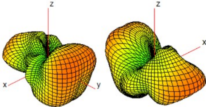
Ant 7(WiFi0/BT/GPS L1)_2450MHz
