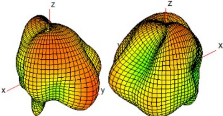
Ant 7(WiFi0/BT/GPS L1)_5300MHz
