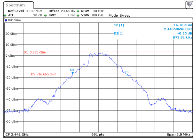
20 dB Bandwidth Plot on Channel 39
