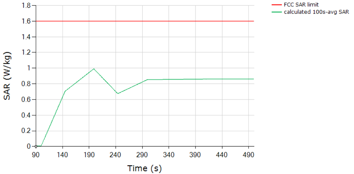
SAR (Test Sequence 1) Tech: LTE, Band 14
