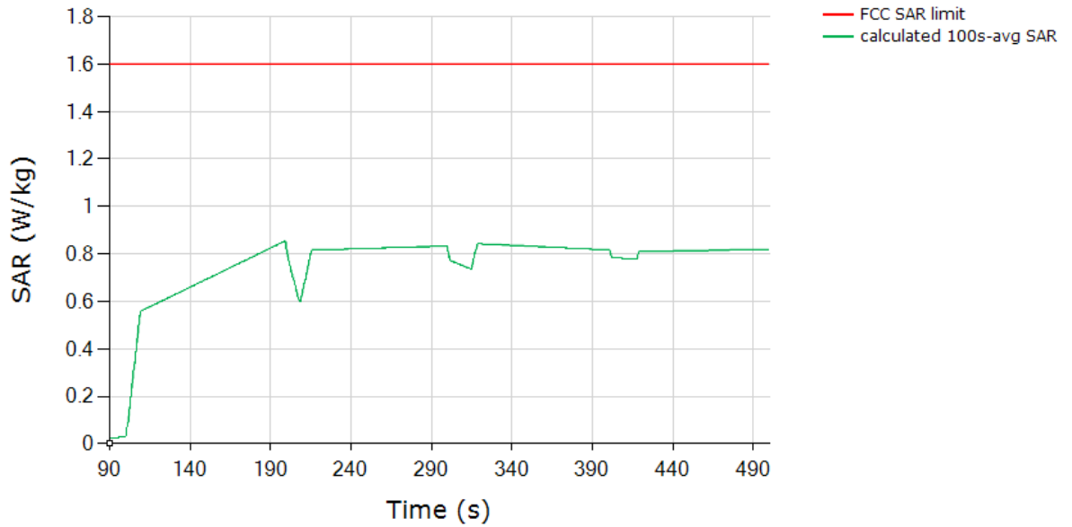
SAR (Test Sequence 1) Tech: WCDMA, Band 4
