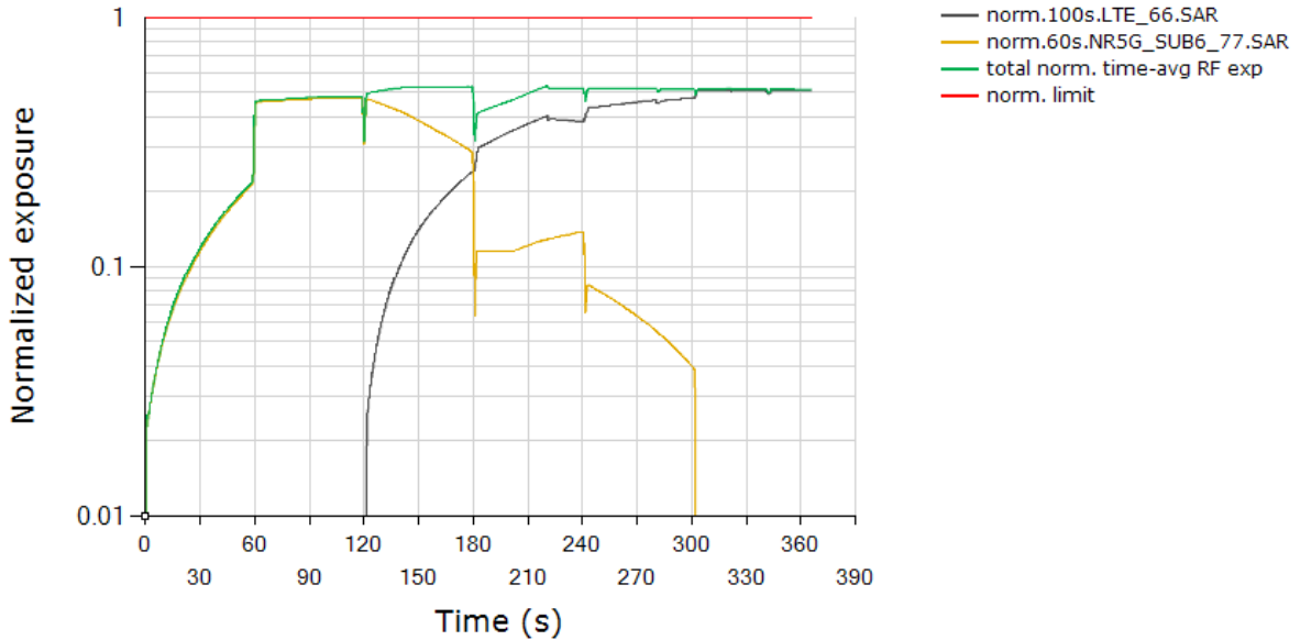
Total Normalized Time-averaged RF Exposure Tech: LTE, Band 66 / Tech: NR5G SUB6, Band 77
