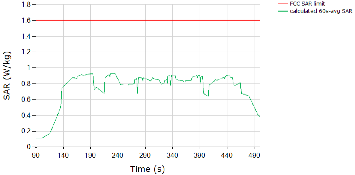
SAR (Test Sequence 2) Tech: LTE, Band 48
