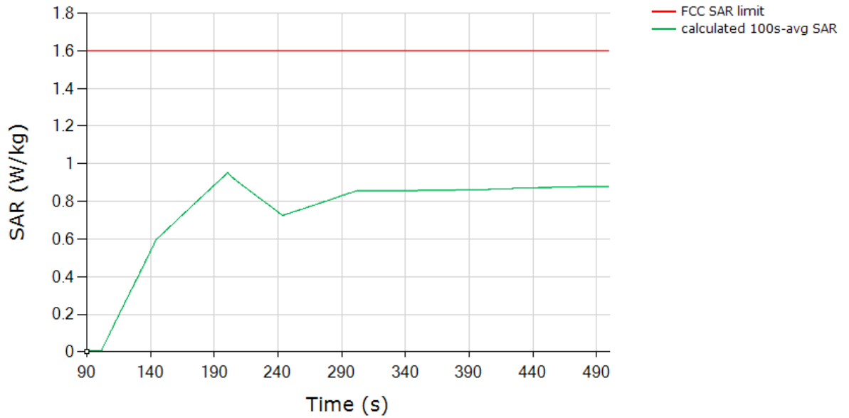
SAR (Test Sequence 1) Tech: NRSUB6, Band 71
