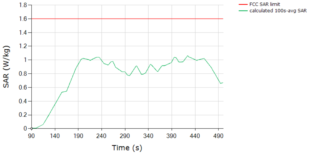
SAR (Test Sequence 2) Tech: LTE, Band 14
