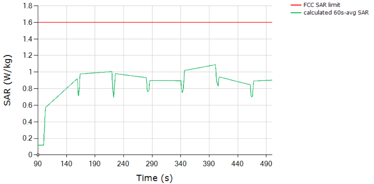
SAR (Test Sequence 1) Tech: LTE, Band 48
