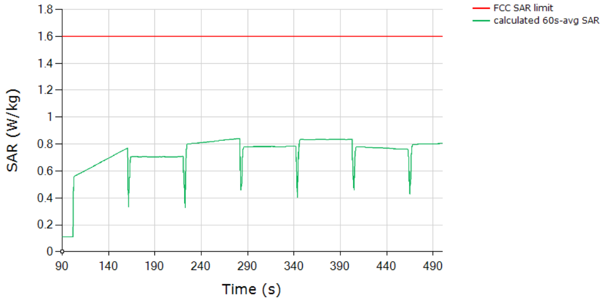
SAR (Test Sequence 1) Tech: NRSUB6, Band 77
