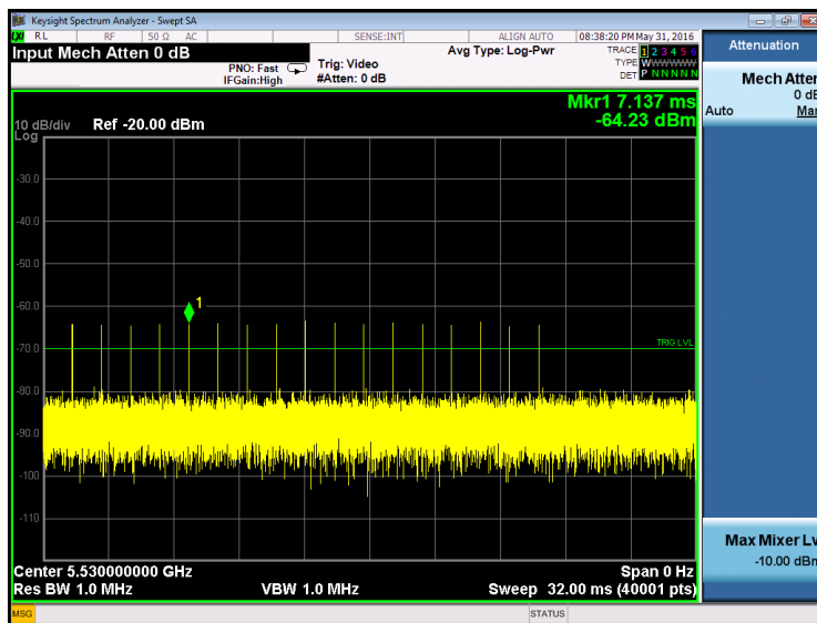
Calibration Radar #0 detection threshold level
