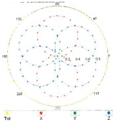
f=600 MHz,TEM
