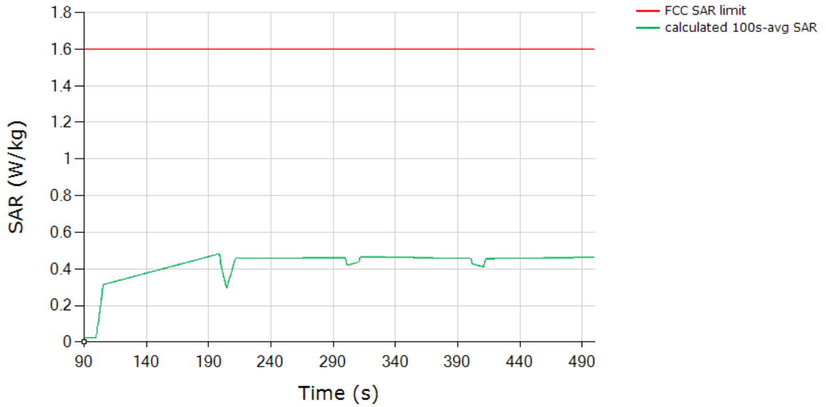
SAR (Test Sequence 1) Tech: LTE, Band 2
