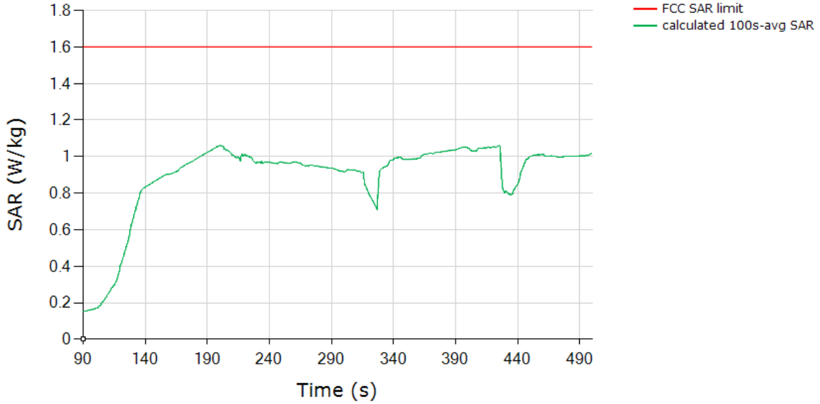
SAR (Test Sequence 2) Tech: NRSUB6SA, Band 41
