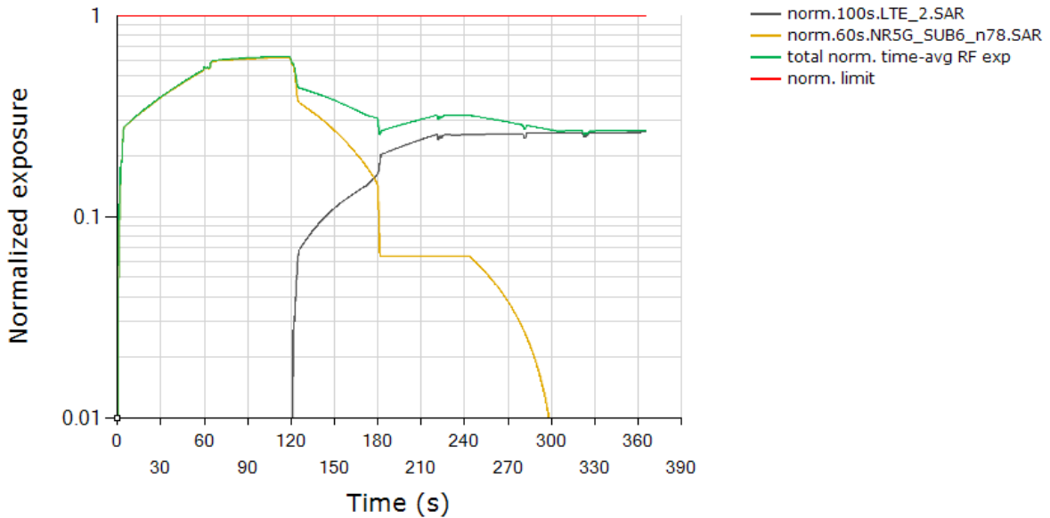
Total Normalized Time-averaged RF Exposure Tech: LTE, Band 2 / Tech: NR5G SUB6, Band n78
