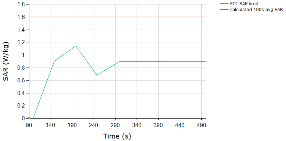
SAR (Test Sequence 1) Tech: LTE, Band 5
