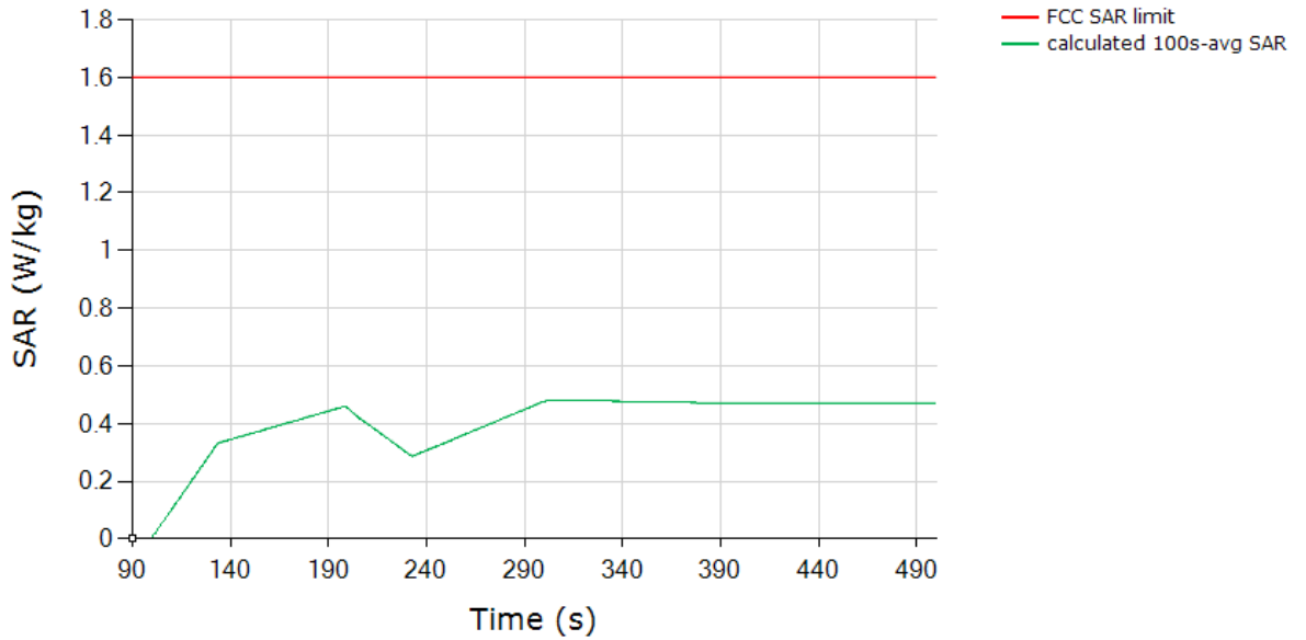
SAR (Test Sequence 1) Tech: WCDMA, Band 5
