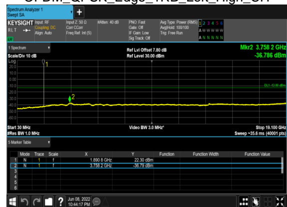
N2(20M)_DFT-s-OFDM_QPSK_Edge_1RB_Left_High_CH
