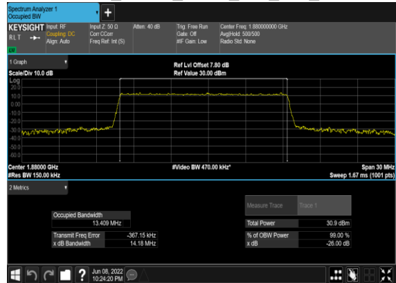
N2(15M)_DFT-s- OFDM_QPSK_Outer_Full_Mid_CH
