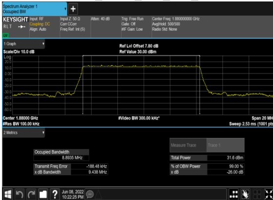
N2(10M)_DFT-s-OFDM_PI_2- BPSK_Outer_Full_Mid_CH
