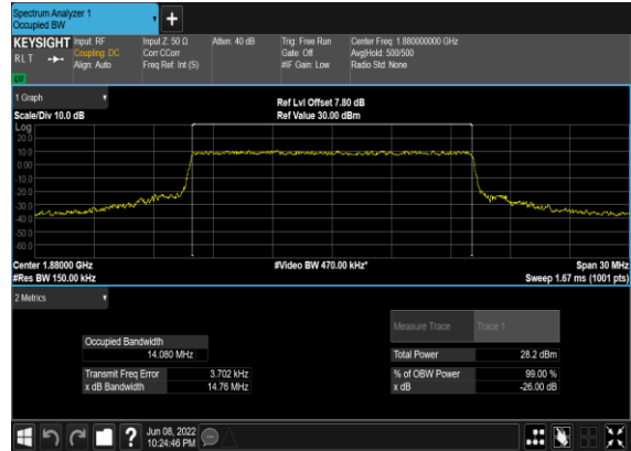
N2(15M)_CP-OFDM_16 QAM_Outer_Full_Mid_CH
