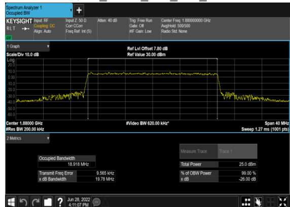
N2(20M)_CP-OFDM_256QAM_Outer_Full_Mid_CH
