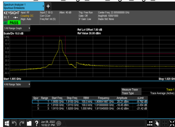
N2(10M)_DFT-s-OFDM_QPSK_Edge_1RB_Right_High_CH
