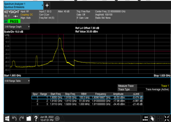
N2(5M)_DFT-s-OFDM_QPSK_Edge_1RB_Right_High_CH
