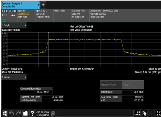
N2(15M)_CP- OFDM_QPSK_Outer_Full_Mid_CH
