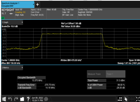
N2(15M)_DFT-s-OFDM_PI_2- BPSK_Outer_Full_Mid_CH
