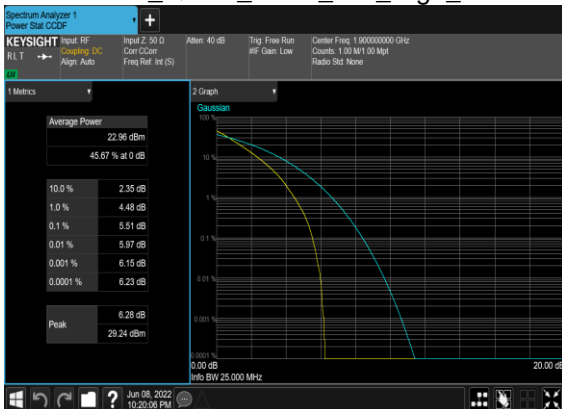
N2(20M)_DFT-s-OFDM_QPSK_Outer_Full_High_CH
