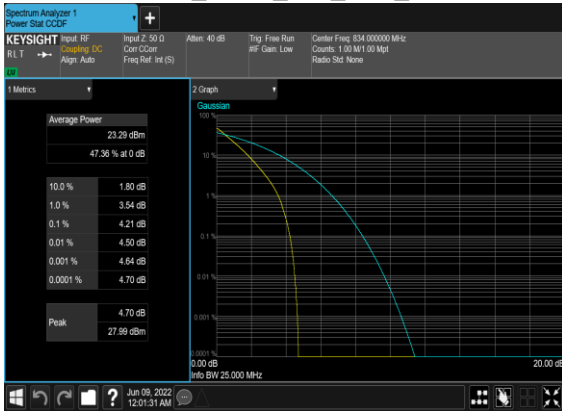
N5(20M)_DFT-s-OFDM_PI_2-BPSK_Outer_Full_Low_CH
