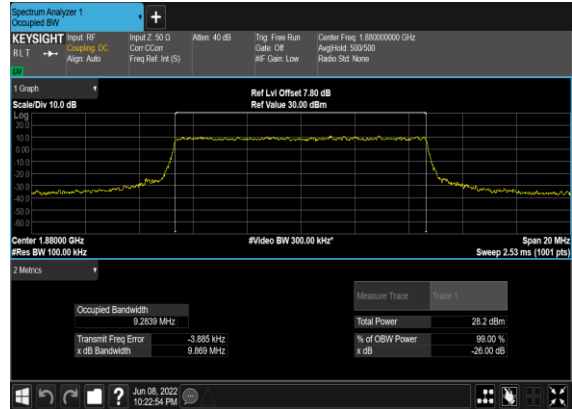
N2(10M)_CP-OFDM_16 QAM_Outer_Full_Mid_CH
