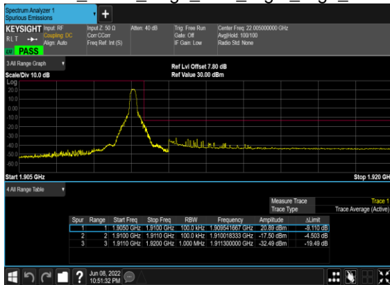
N2(10M)_DFT-s-OFDM_BPSK_Edge_1RB_Right_High_CH
