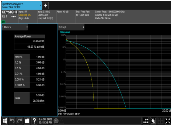
N2(20M)_DFT-s-OFDM_PI_2-BPSK_Outer_Full_Low_CH
