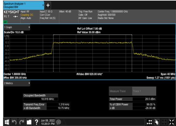
N2(20M)_CP-OFDM_16QAM_Outer_Full_Mid_CH
