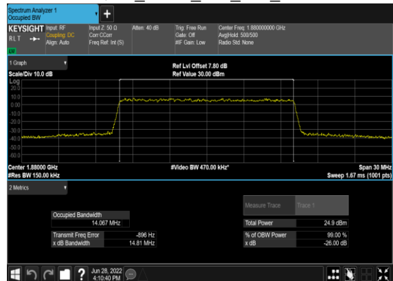
N2(15M)_CP-OFDM_256 QAM_Outer_Full_Mid_CH
