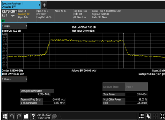
N2(10M)_CP- OFDM_QPSK_Outer_Full_Mid_CH
