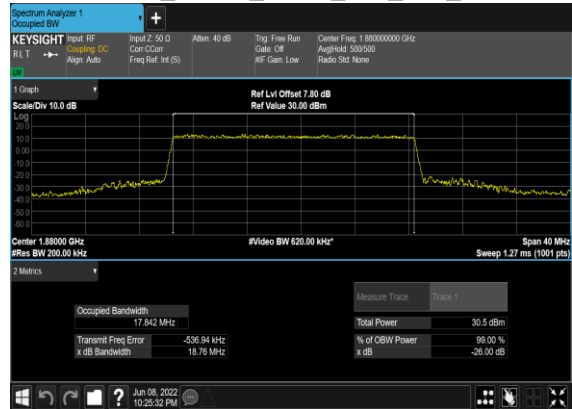
N2(20M)_DFT-s-OFDM_QPSK_Outer_Full_Mid_CH
