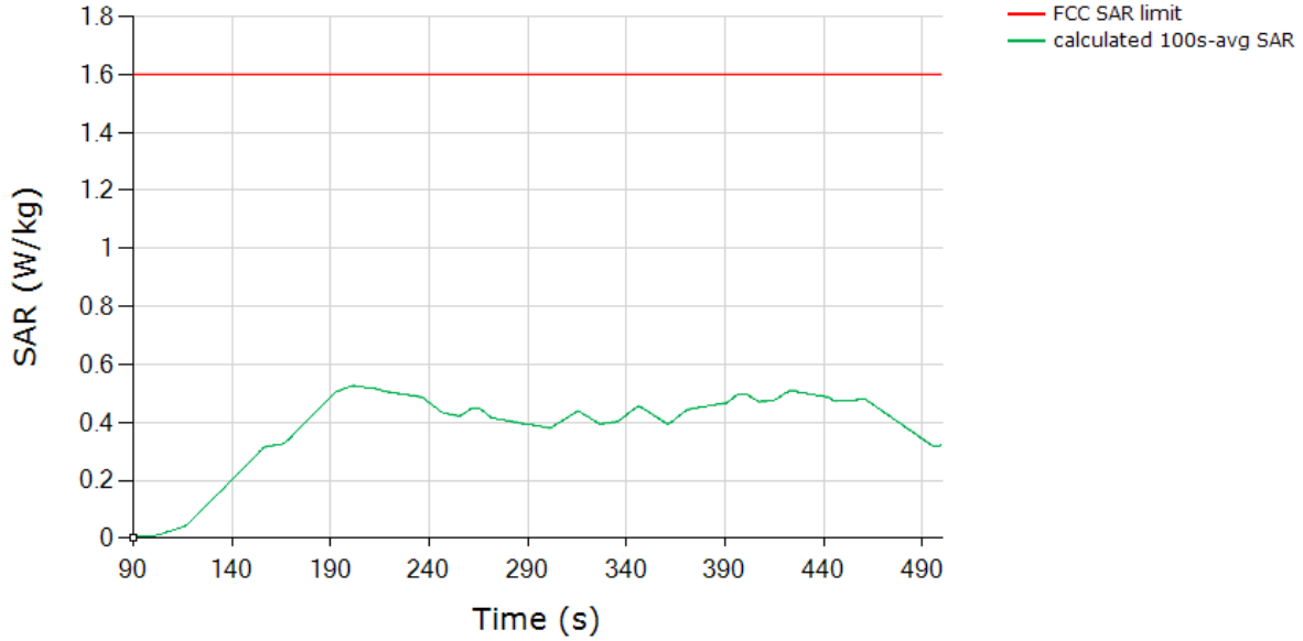
SAR (Test Sequence 2) Tech: NRSUB6SA, Band 7
