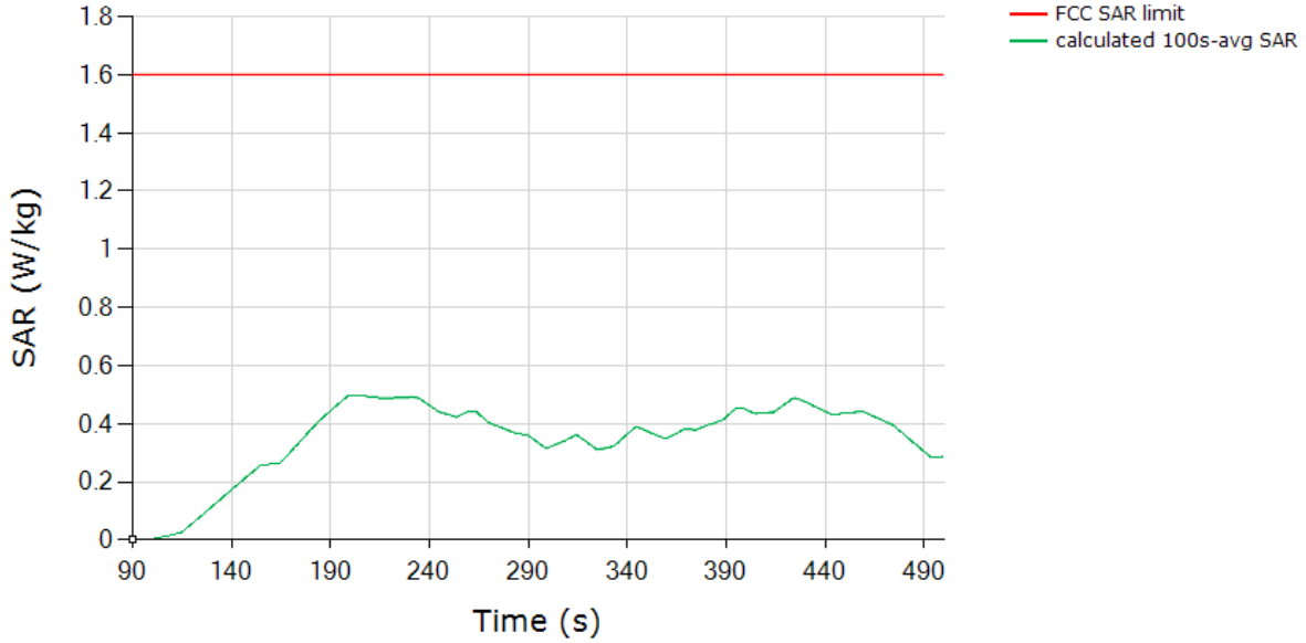
SAR (Test Sequence 2) Tech: LTE, Band 5
