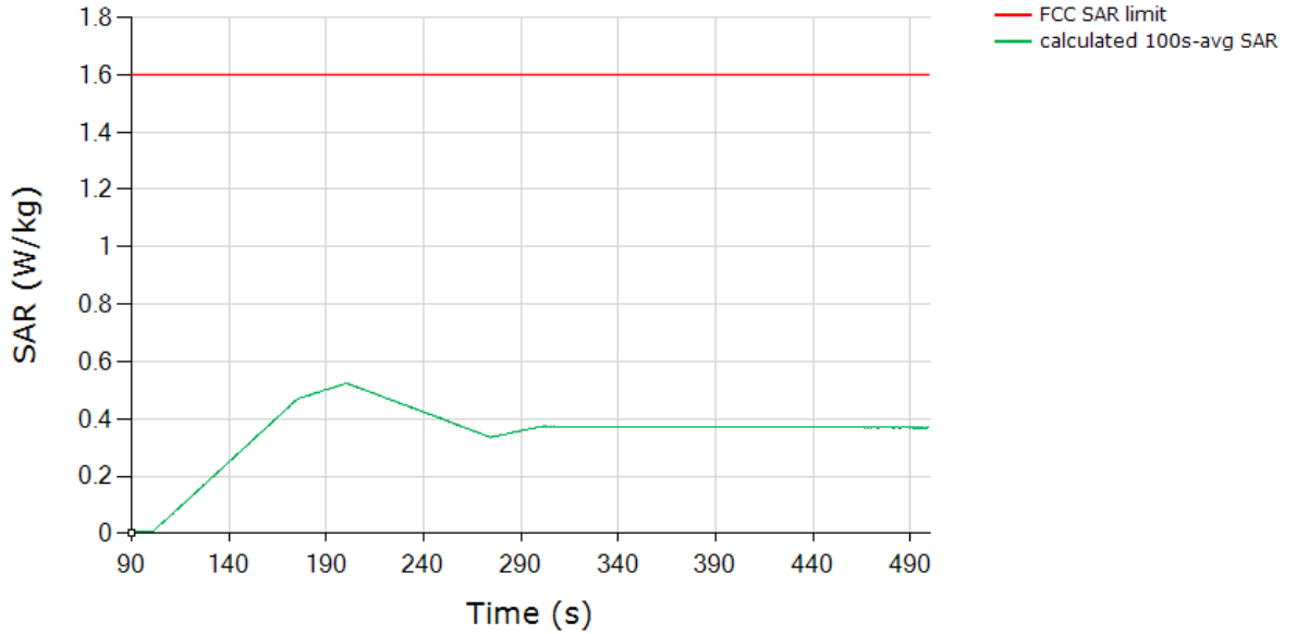
SAR (Test Sequence 1) Tech: NRSUB6SA, Band 7
