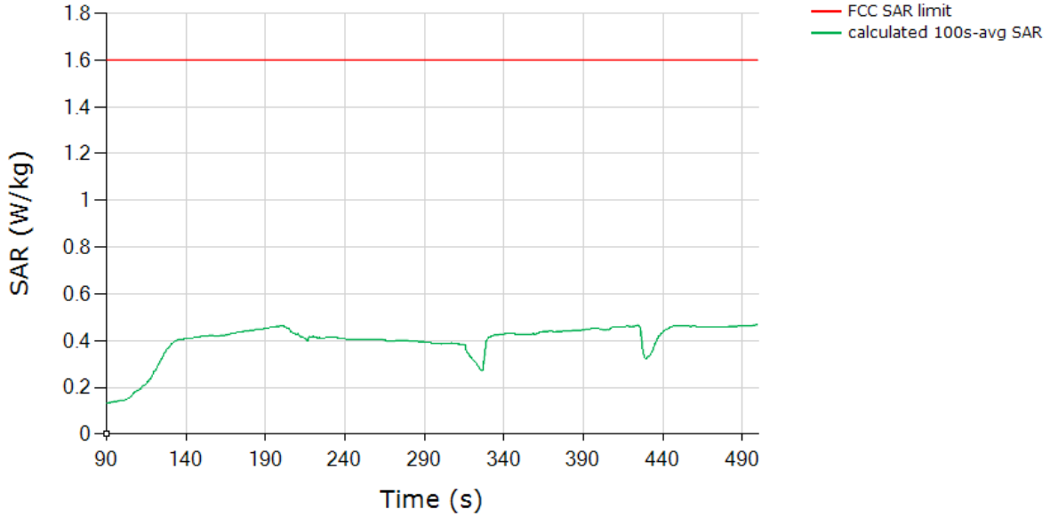
SAR (Test Sequence 2) Tech: NRSUB6SA, Band 38
