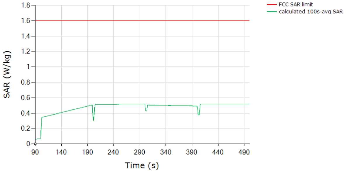
SAR (Test Sequence 1) Tech: LTE, Band 7
