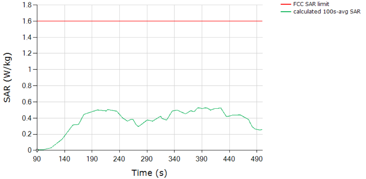
SAR (Test Sequence 2) Tech: GSM, Band 850
