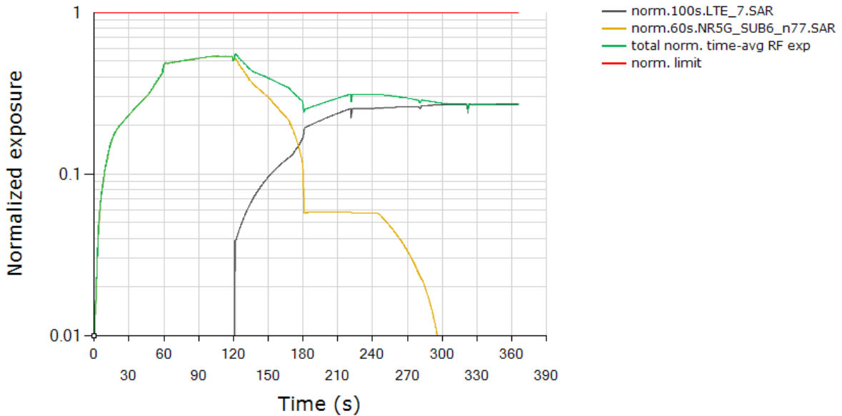
Total Normalized Time-averaged RF Exposure Tech: LTE, Band 7 / Tech: NR5G SUB6, Band n77
