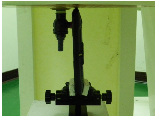
Primary Portrait with Phantom 0 cm Gap (EUT with Jelly Sets)
