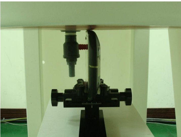
Front Face with Phantom 0 cm Gap (EUT with Holster)
