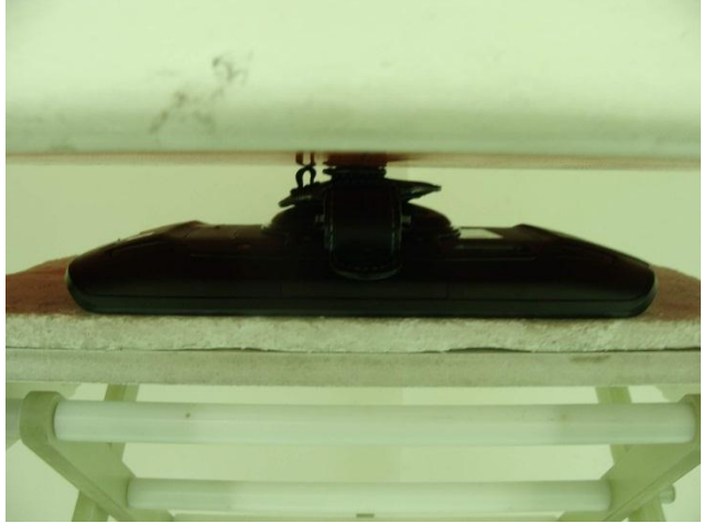
Bottom Face with Phantom 0 cm Gap (EUT with Hand Strap)
