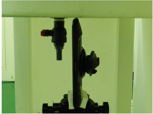
Secondary Portrait with Phantom 0 cm Gap (EUT with Hand Strap)
