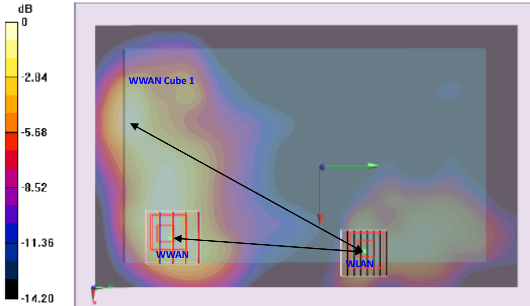
0 dB = 0.744 mW/g = -2.57 dB mW/g
