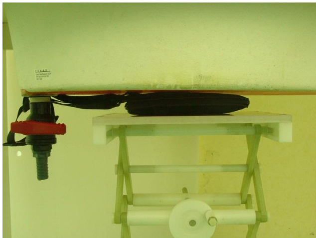
Front face of DUT with phantom 0 cm gap (DUT with Holster)
