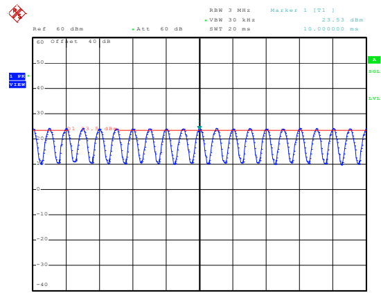
1880MHz - 80% AM
