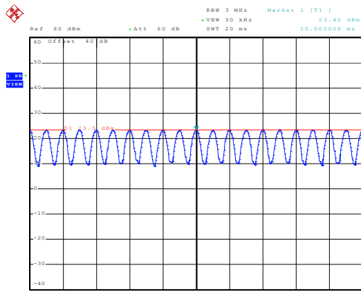
835MHz - 80% AM
