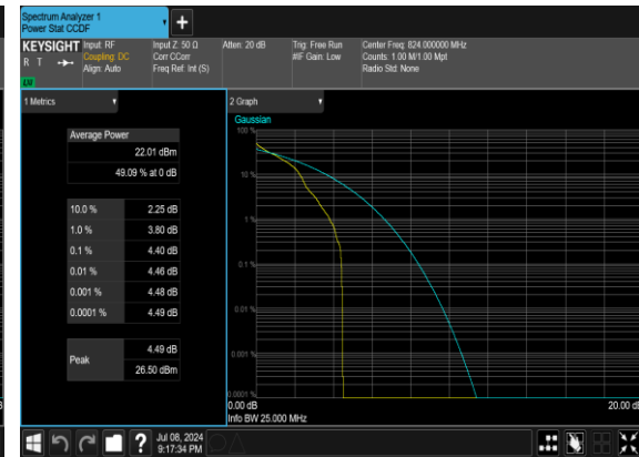
N26(20M)_DFT-s-OFDM_PI_2-BPSK_Edge _1RB_Left_Mid_CH
