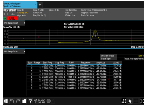
B2_N30(10M)_DFT-s- OFDM_BPSK_Edge_1RB_Right_Low_CH
