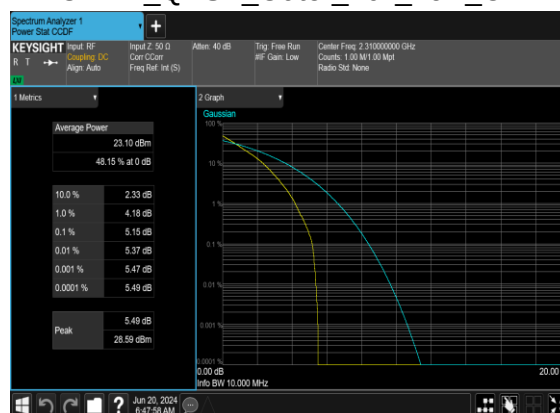
B5_N30(10M)_DFT-s-OFDM_QPSK_Outer_Full_Low_CH
