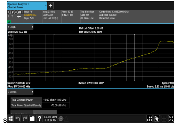
B2_N30(10M)_DFT-s- OFDM_BPSK_Edge_1RB_Left_Low_CH_CHP_PAS
