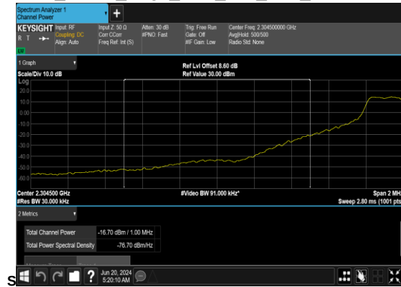
B2_N30(10M)_DFT-s- OFDM_QPSK_Edge_1RB_Left_Low_CH_CHP_PAS
