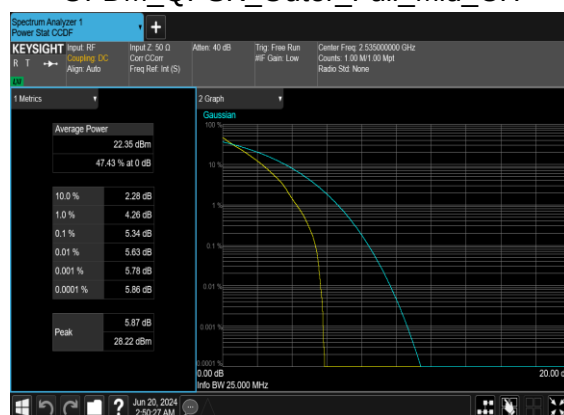
B2_N7(20M)_DFT-s-OFDM_QPSK_Outer_Full_Mid_CH
