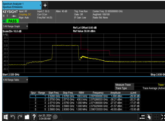
B2_N7(20M)_DFT-s- OFDM_QPSK_Outer_Full_High_CH
