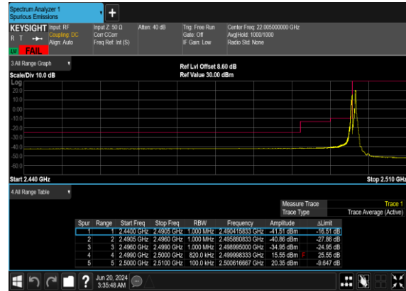
B2_N7(40M)_DFT-s- OFDM_BPSK_Edge_1RB_Left_Low_CH
