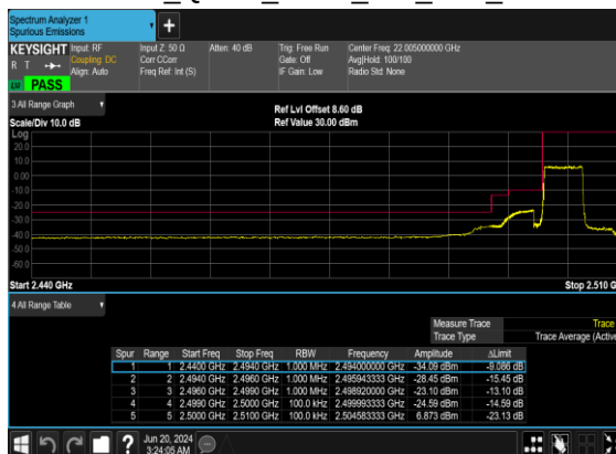
B2_N7(5M)_DFT-s- OFDM_QPSK_Outer_Full_Low_CH
