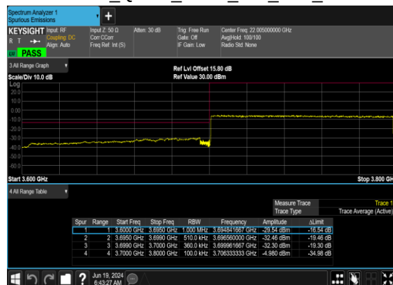
B2_N77(100M)_DFT-s- OFDM_QPSK_Outer_Full_Low_CH
